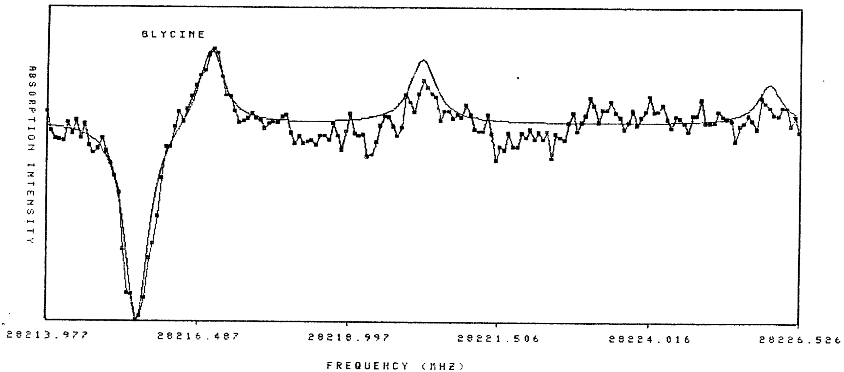
Fig. 2.13 Determination of the \mu_a dipole moment component with the transition ( J_{K_a K_c} = 4_2, 3^+3_2, 2_2 ). Plots of calculated and experimental spectra.
