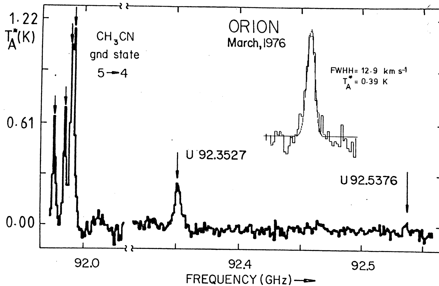
Fig. 5.3 The ( v = 0 ) and ( v_8 = 1 ) ( J = 5 \rightarrow 4 ) transitions of methyl cyanide from Ori A.
