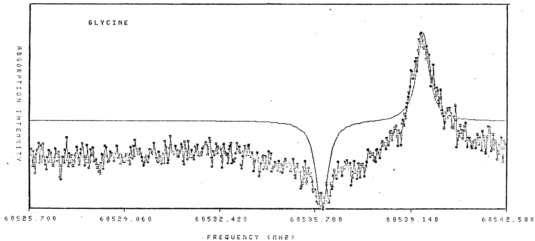
Fig. 2.14 Determination of the \mu_b dipole moment component with the transition ( J_{K_a K_c} = 8_{2,6} \leftarrow 7_{2,5} ).
