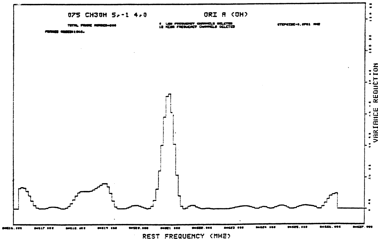
Fig. 4.1 The ( J_K = 5_{-1}^{-4}_0 E) emission of methanol from Ori A and its statistical analysis. The (1950) pointing position was:
