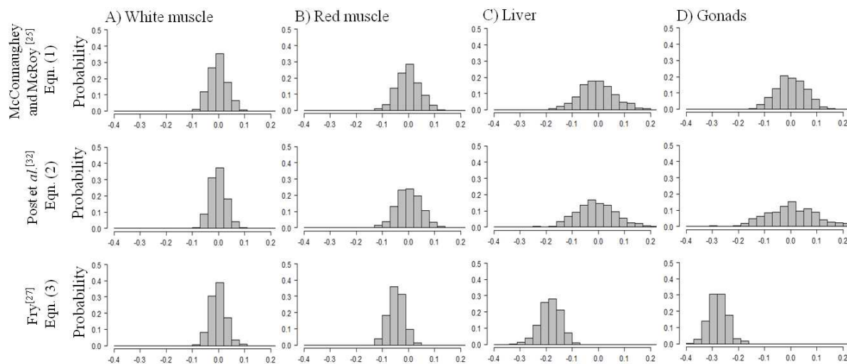
Fig. 5.4: Distributions of the \Delta\delta^{13}\text{C}_{\text{error}} , i.e. the differences between the lipid-corrected and observed lipid-free \delta^{13}\text{C} values in different tissues of tropical tuna. Lipid-corrected values were predicted from the three lipid-normalization models using a cross validation procedure that was repeated 500 times. \Delta\delta^{13}\text{C}_{\text{error}} = \delta^{13}\text{C}_{\text{corrected}} - \delta^{13}\text{C}_{\text{lipid-free}}
