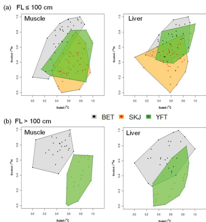
Fig. 6.3: Two-dimensional scaled isotopic space ( \delta^{15}\text{N} and \delta^{13}\text{C} ) in the muscle and liver of skipjack tuna (SKJ), yellowfin tuna (YFT) and bigeye tuna (BET) caught in the Western-Central Indian Ocean (WCIO), according to size class: (a) fish with fork length less than 100 cm ( \text{FL} \leq 100 cm), (b) fish with fork length higher than 100 cm ( \text{FL} > 100 cm).
