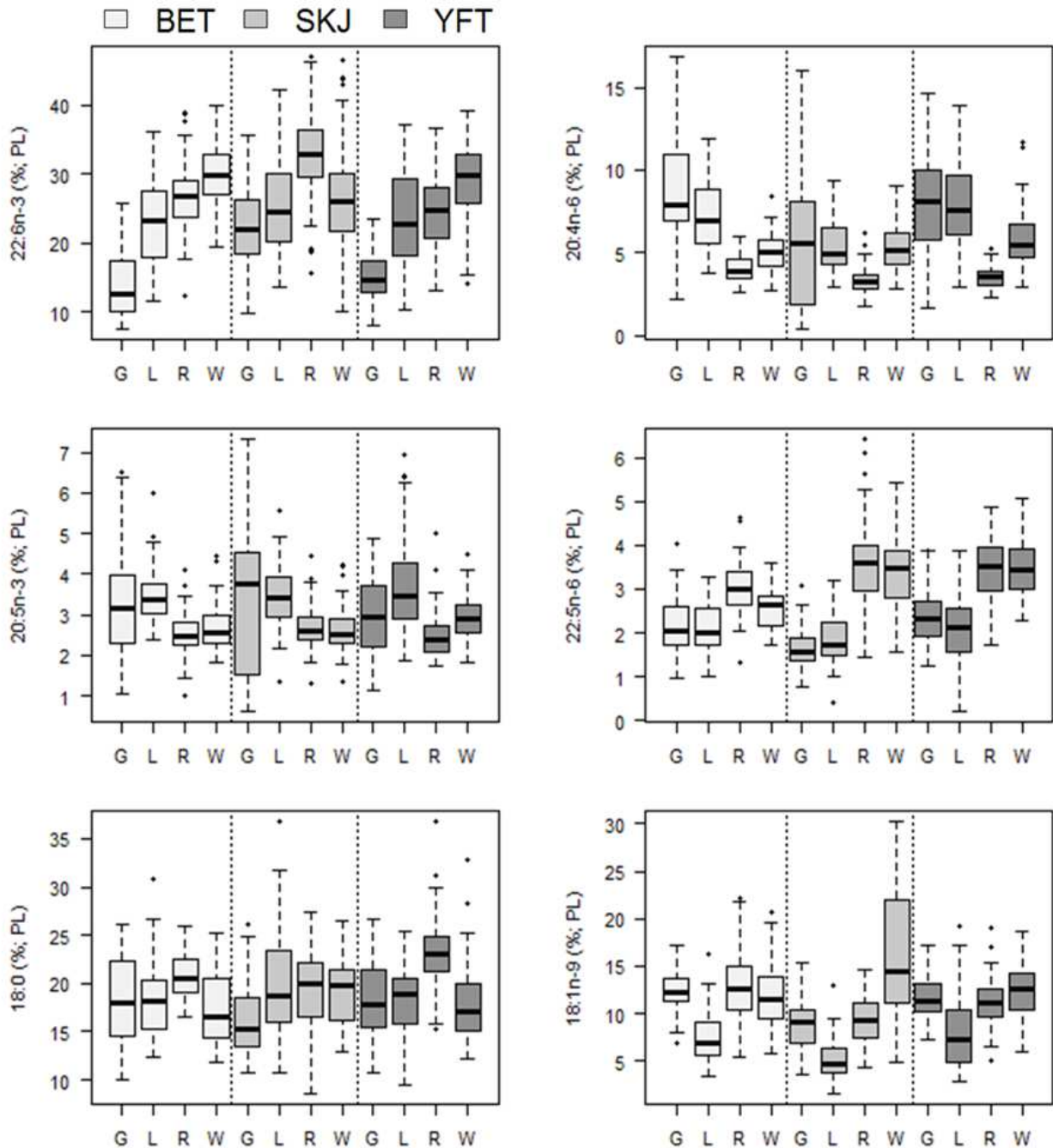
Fig. 8.4: Boxplots of some individual FA proportions in polar lipids (PL) of gonads (G; n=45, 49 and 43 in BET, SKJ and YFT respectively), liver (L; n=50, 55 and 49), red muscle (R; n=55, 59 and 54), white muscle (W; n=53, 59 and 54) in three tropical tunas from the Western Indian Ocean (BET, bigeye; SKJ, skipjack; YFT, yellowfin). The dots represent outliers.
