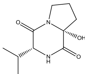
Bacillusamide B
