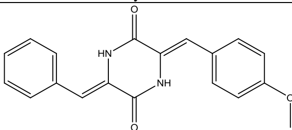
Phenylahistine
