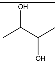
butan-2,3-diol
