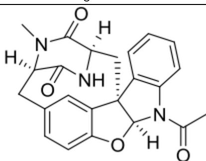
Azonazine
