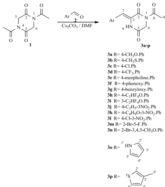
Scheme 1. Synthesis of arylidene 2,5-diketopiperazine derivatives 3a-p .
