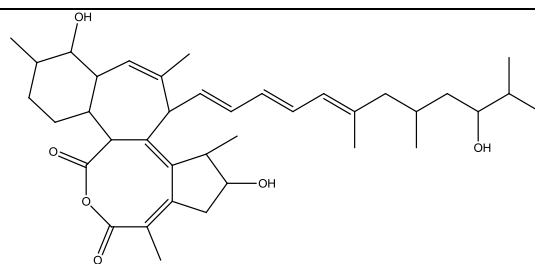
Aurantinine A
