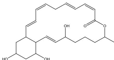
Macrolactine L
