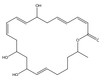
Macrolactine H
