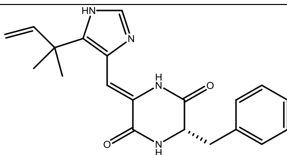
Phenylahistine
