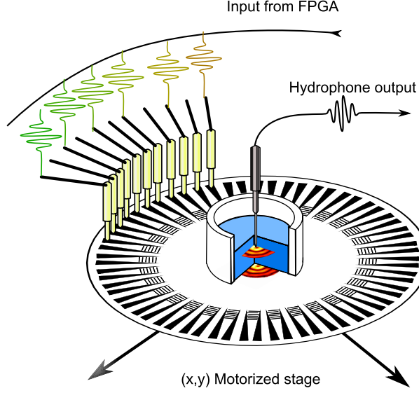
Figure IV.8: Experimental setup to study the degeneration of acoustical vortices.
