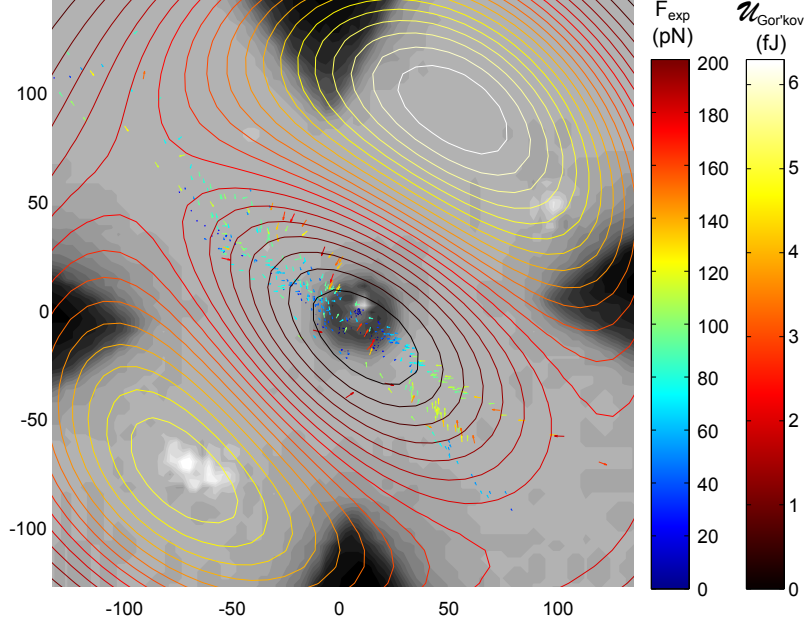
Figure IV.17: Experimental forces and theoretical Gor'kov potential \mathcal{U}_{\text{Gor'kov}} of a 10 MHz \mathcal{W}_1 swirling SAW acting on a 30\ \mu\text{m} diameter polystyrene sphere. The input voltage is 7\ V_{\text{rms}} which yields an electrical power of 1.0\ \text{W} . The x and y axis of the figure are labeled in \mu\text{m} . The geometry of the trap is clearly visible as an elongated valley.
