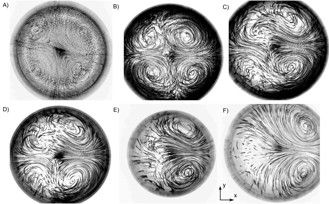
Figure III.2: Flow visualization of a 12.5 \mu\text{l} droplet from below, at various glycerol concentration. The SAW propagates from left to right with an amplitude u_0 = 62 \pm 1 pm. As the viscosity increases, one remarks the progressive transition from a four-vortex to a two-vortex flow structure. (A) Pure water (B) 30 wt% glyc. (C) 40 wt% glyc. (D) 60 wt% glyc. (E) 80 wt% glyc. (F) 90 wt% glyc.
