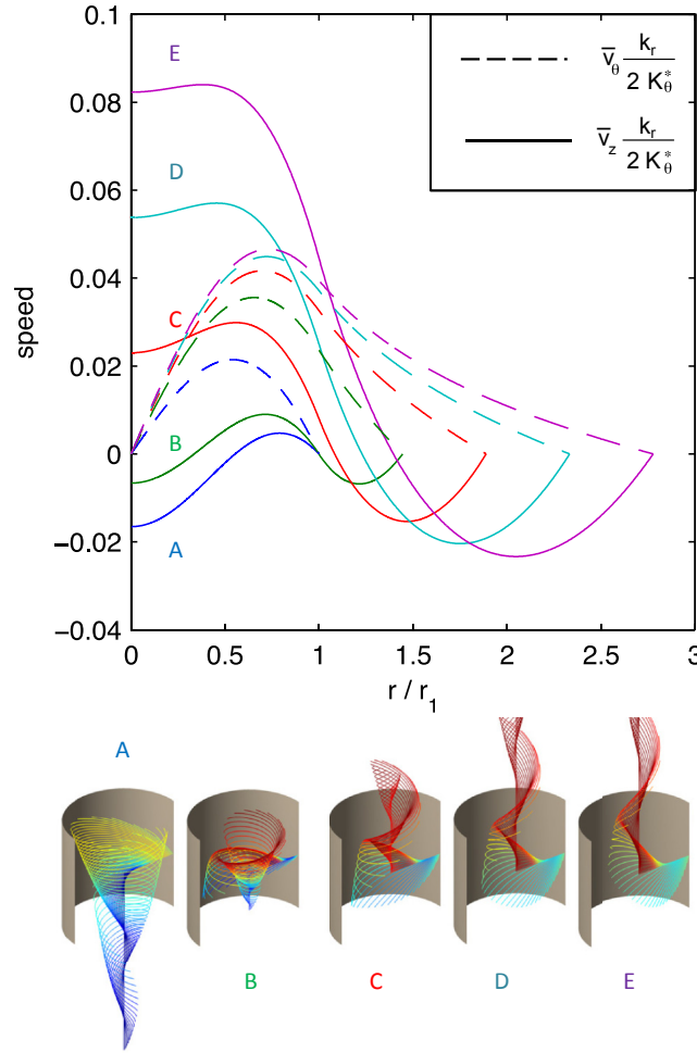
Figure IV.3: Top: Non-dimensional velocities for l = 1 , \tan(\alpha) = 1.21 and k_r r_1 = 1.84 for progressively increased cavity geometrical proportions r_0/r_1 = [1(\text{A}) \ 1.44(\text{B}) \ 1.89(\text{C}) \ 2.33(\text{D}) \ 2.78(\text{E})] . Axial velocity is represented by solid lines and the azimuthal component by the dashed ones. Bottom: Flow streamlines. Colors are indicative of the speed magnitude along \bar{v}_z : extrema are represented by the most intense colors, red for positive and blue for negative.
