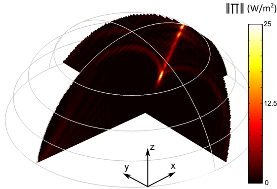
Figure III.6: Poynting vector in a 90 wt% glycerol droplet excited by a 20 MHz acoustic field. \|\langle \Pi \rangle\|_{max} = 25 W/m². Droplet volume is 12.5 \mu\text{L} , base diameter is 4.0 mm. The incident wave propagates along the x axis (from left to right) with an amplitude of 10 pm.
