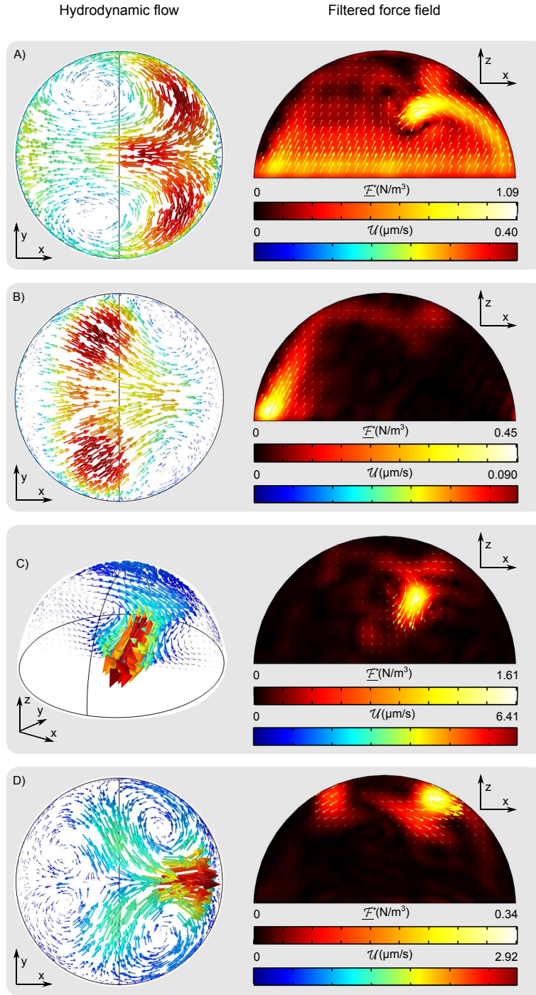
Figure III.9: Numerical simulation of the four main types of acoustic streaming generated by a plane SAW propagating from left to right. A) \alpha D = 0.17 , \Lambda = 5.0 ( \triangle ), B) \alpha D = 6.0 , \Lambda = 5.0 ( \circ ), C) \alpha D = 0.17 , \Lambda = 0.27 ( \nabla ), D) \alpha D = 6.0 , \Lambda = 0.27 ( \square ). Velocity field is depicted on the left, and the forcing term is on the right. Numerical values are computed for an incident SAW of frequency f = 20\text{MHz} and amplitude 10 pm. The droplet diameter is 3.7 mm, fluid properties are those of water, except for the dynamic viscosity \mu which was used to set \Lambda . The other parameter \alpha D was set by tuning the SAW attenuation coefficient in the solid.
