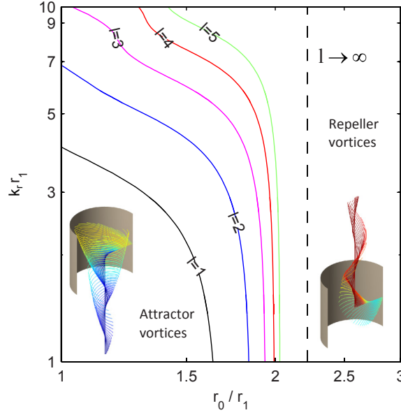
Figure IV.4: Contour plot of \bar{v}_z(r=0) = 0 at various topological charge l , typical dimension k_r r_1 and geometrical ratio r_0/r_1 . Parameters plane is partitioned into two areas, one close to the origin corresponding to attractor vortices with negative axial velocities at r=0 and the other one corresponding to repeller vortices. The dashed line at r_0/r_1 \sim 2.218 indicates an asymptotic limit obtained for large l values.
