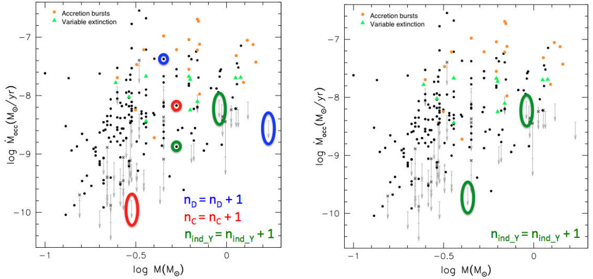
(c) Pairing of one detection and one upper limit.
