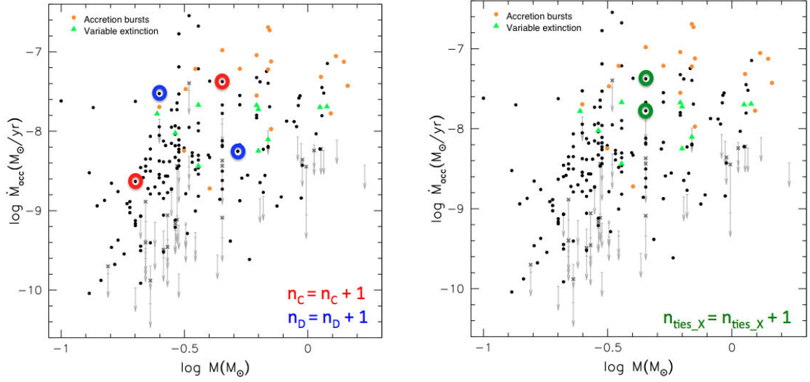
(a) Pairing of two detections at different M_{\star} .
