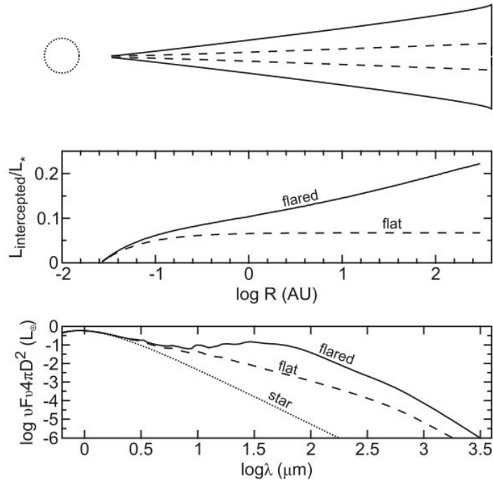
Figure 1.5: Comparison of the disk geometry (upper panel), fraction of stellar flux intercepted (middle panel) and emitted spectral energy distribution (lower panel) for a flared disk as opposed to a flat disk. From Garcia et al. (2011).
