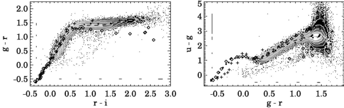
Figure 3.1: Color loci of point sources in the SDSS sample on the (g - r, u - g) and (r - i, g - r) diagrams (from Covey et al. 2007). Small black dots correspond to individual sources; contours show source density, starting from 10 000 objects per square magnitude and increasing by a factor of 3 between contours. The dashed line indicates the location of the median stellar locus.
