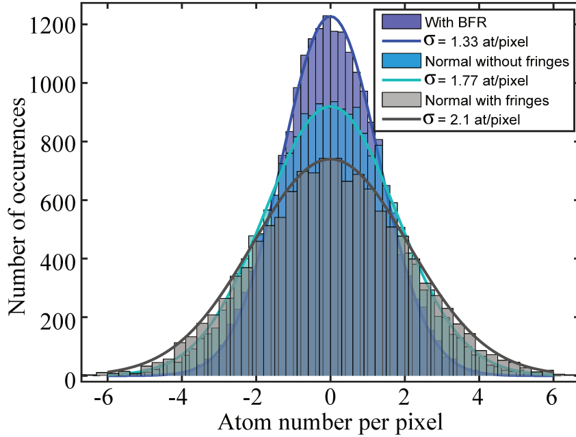
Figure 3.9: Detection noise estimation in three different cases. Histograms of the calculated atom numbers per pixel over the same area as figure 3.6 at I = I_{sat} and without atoms, without fringes (clear blue), with fringes (grey) and using the fringe reconstruction algorithm (dark blue). The standard deviation of the data without fringes was directly derived from eq. (3.19) showing that the detection is limited by photon shot noise in the absence of fringes. On the other hand, a Gaussian adjustment is applied in the first and last cases giving a standard deviation of 2.1 > \sigma_{PSN} for the degraded data and \sigma_{PSN}/\sqrt{2} < 1.33 < \sigma_{PSN} after correction.
