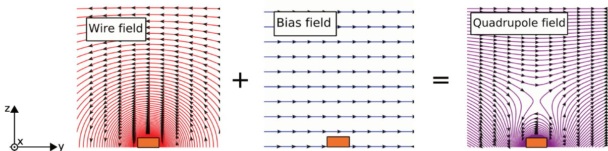
Figure 1.2: Principle of a quadrupole magnetic trap. The combination of the field radiated by a current carrying wire and a homogeneous bias field results in a quadrupole field that presents a local minimum inside which atoms can be trapped. Taken from [103].
