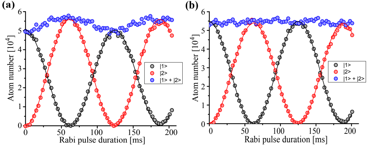
Figure 3.11: Comparison of the two detection schemes in term of state detectivity. Rabi oscillations between the two clock states |1\rangle (black) and |2\rangle (red) detected with the two presented detection methods. In the case of the SDD (a), the oscillation of the total atom number (blue) testifies of a state-dependent detection efficiency. The sinusoidal fits give a detection efficiency of |1\rangle lower than the one of |2\rangle by a factor 0.89. On the other hand, for the ARP (b) the total atom number (blue) remains constant and the fits give the same detection efficiency for the two states.
