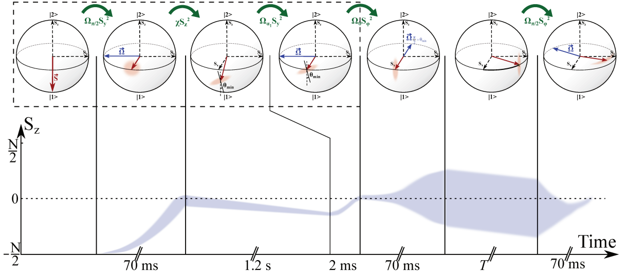
Figure 5.17: Ramsey interferometry below the standard quantum limit. The previously described procedure is used to generate a squeezed spin state, which is then placed back on the equator of the Bloch sphere using the correction pulse detailed in section 4.4.3. Next, a \frac{\pi}{2} + \theta_{min} -pulse rotates the spin noise distribution until its small axis is aligned with the phase quadrature. After a free evolution time T , another \frac{\pi}{2} -pulse converts the accumulated phase into populations that can be probed with a precision better than the SQL. The evolution of the population difference is also indicated.
