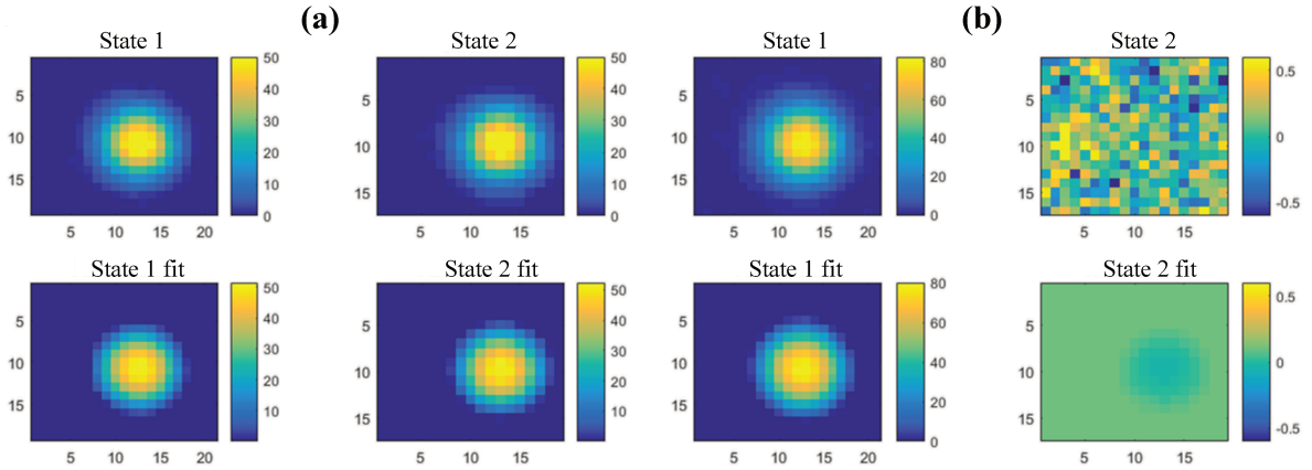
Figure 3.14: Characterization on the ARP efficiency. (a) 4000 atoms are prepared in a coherent superposition and imaged with the standard double state detection method 50 times. The 50 images are averaged (upper images), and the averaged clouds are fitted with a parabola (lower images). (b) 4000 atoms are prepared in |1\rangle and imaged with the ARP method + repumper 50 times. The "state 1" images correspond to the atoms detected with the ARP and the "state 2" images correspond to the remaining one detected after being re-pumped.
