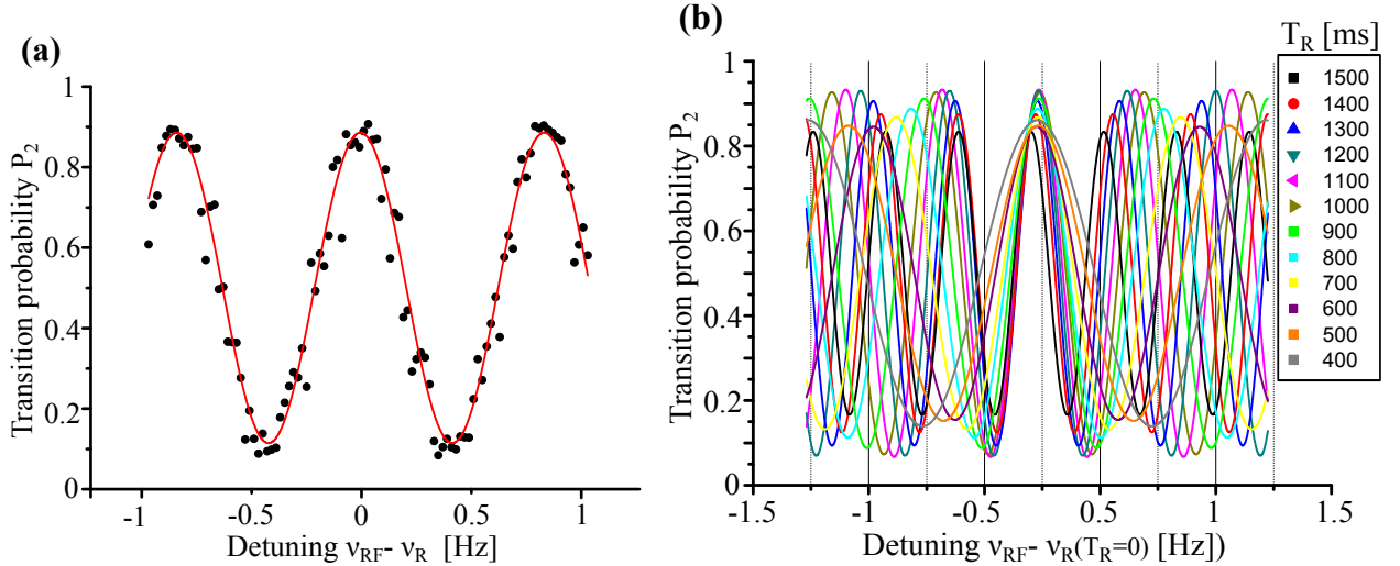
Figure 4.4: Ramsey spectra of 12.10^3 condensed atoms initially. (a) Ramsey spectrum for T_R = 1.2 s, obtained by scanning the local oscillator frequency. The black dots are experimental data, while the red line represents the a fit with eq. (4.13). (b) Fits of Ramsey spectra obtained for different Ramsey times (colored lines).
