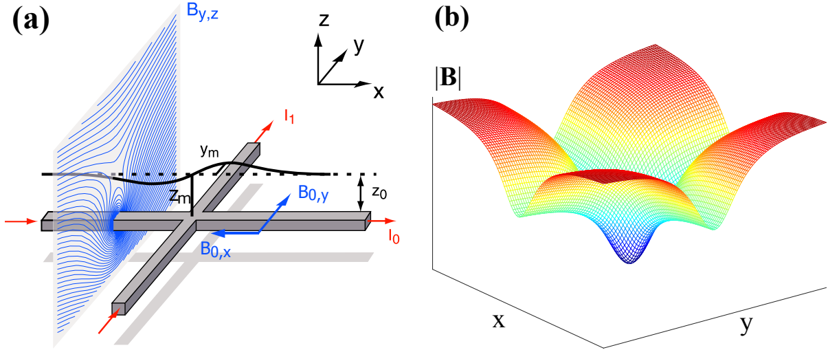
Figure 1.3: Dimple trap. (a) Three dimensional Ioffe-Pritchard trap generated by two crossing wires and a combination of two bias fields. The resulting field in the y - z plane is shown. Adapted from [89]. (b) Magnetic field strength in the x - y plane.
