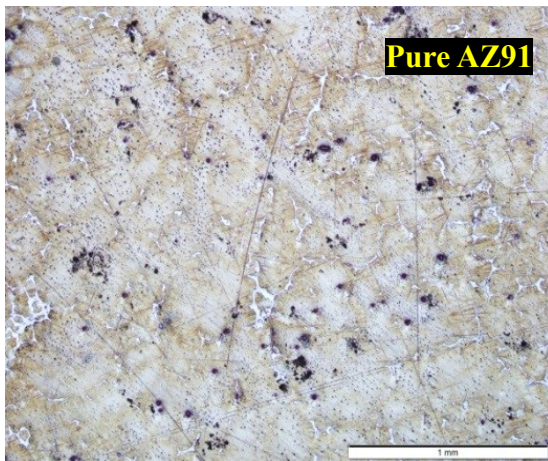
Fig 113 Pure Magnesium AZ91
