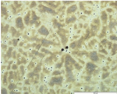
Fig 211 \text{Al}_2\text{O}_3 particle
