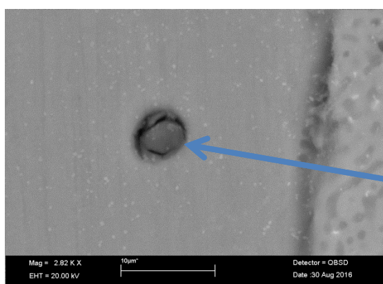
Fig 141 MgO Particle
