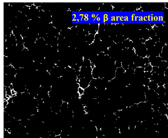
Fig 114 Pure Mg AZ91: \beta phase area fraction
