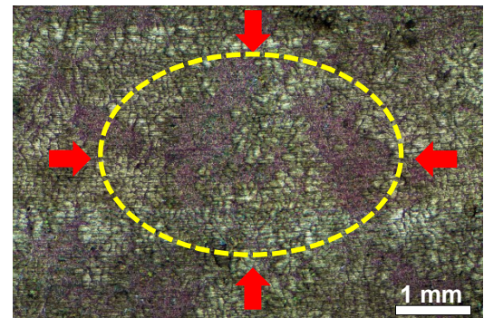
Fig 68 Stirred Al A357 at 70 mT
