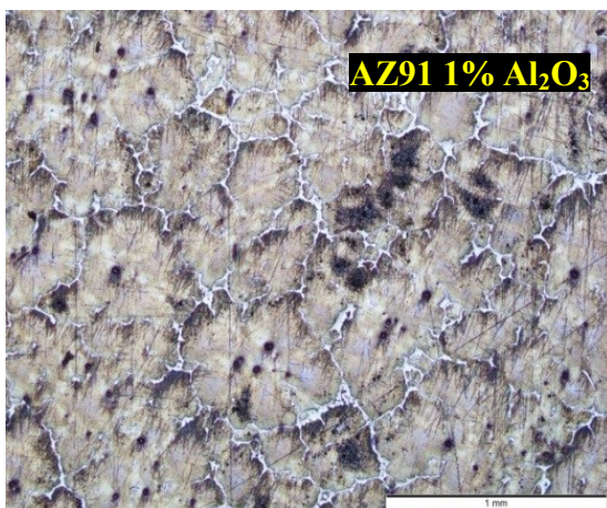
Fig 115 Mg AZ91 1% \text{Al}_2\text{O}_3
