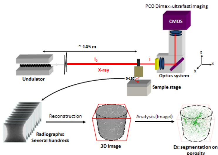
Fig 46 X-ray tomography system scheme
