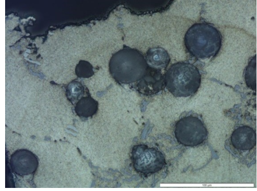
Fig 210 \text{Al}_2\text{O}_3 particles detail view 2
