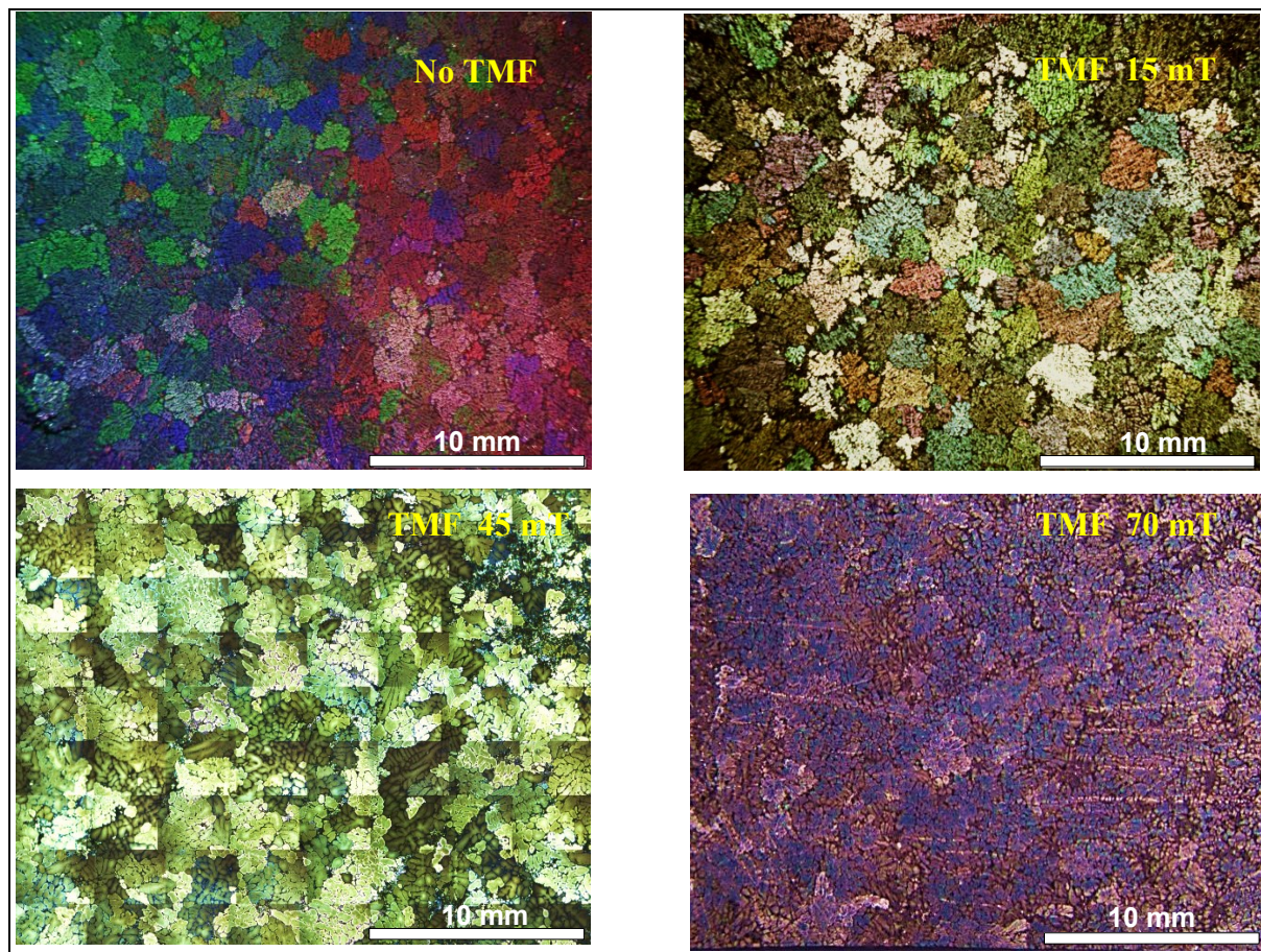
Fig 60 Aluminium A357 grain structure at different TMF intensities
