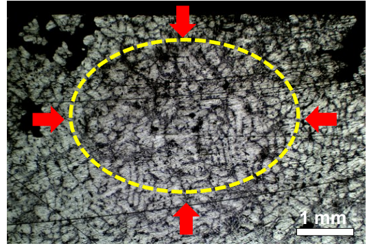
Fig 64 Detail view Al A357 stirred at 15mT
