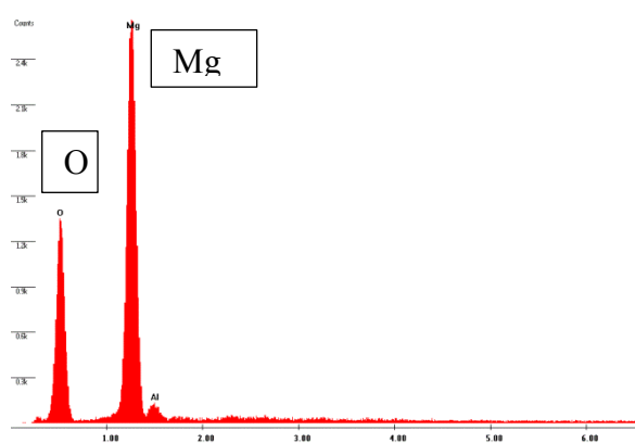
Fig 142 X-ray MgO spectrometry
