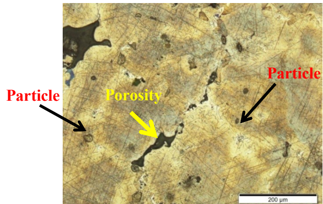
Fig 145 AZ91 + 2% SiC 0.1-1μm sample
