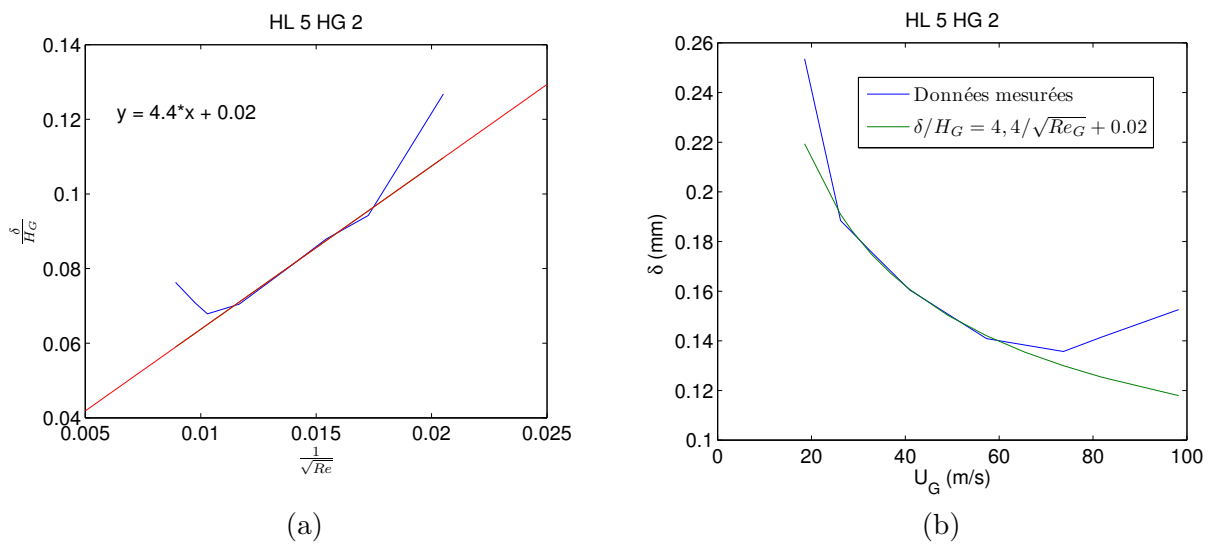
FIGURE C.1 –  paisseur de vorticit  H_L = 5 mm H_G = 2 mm.
