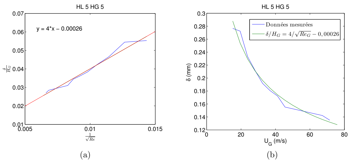
FIGURE C.2 –  paisseur de vorticit  H_L = 5 mm H_G = 5 mm.
