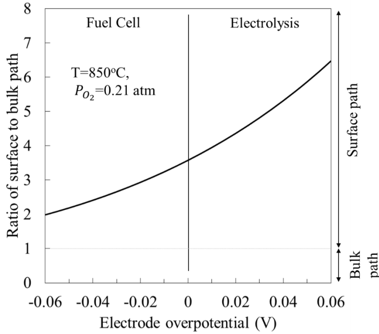
Figure V.5 - Kinetic rate ratio of surface path (TPBs) to bulk path (MIEC surface) for the studied LSCF-GDC and LSCF electrode.
