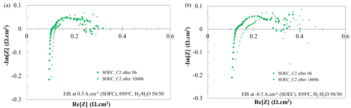
Figure IV.11 - Electrochemical Impedance Spectra of SOEC_C2 after 0h and 1000h (a) at 0.5 A.cm^{-2} and (b) at -0.5 A.cm^{-2} . There is a clear increase of the high frequency contribution in SOEC mode.
