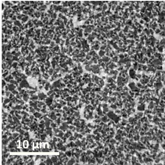
Figure V.16 – View of a slice extracted from a 3D reconstruction obtained by nano-holotomography of a LSCF-GDC electrode.
