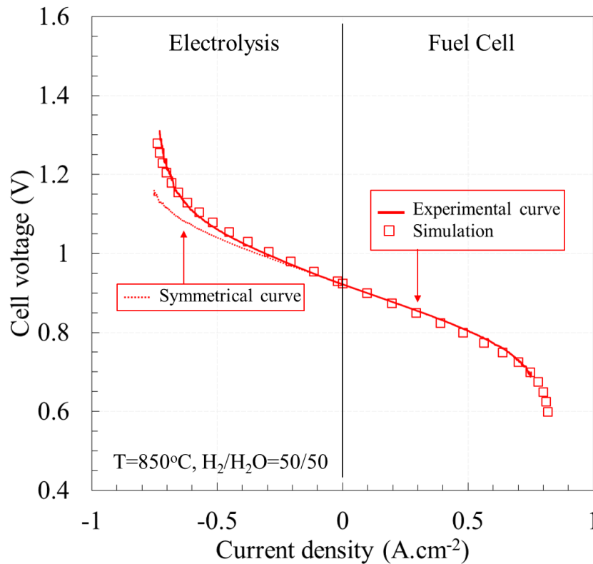
Figure V.9 – Experimental and simulated polarisation curves for a pristine cell at 850°C, \text{H}_2/\text{H}_2\text{O}=50/50 . The dissymmetry is highlighted by the symmetrical fuel cell curve reported in electrolysis mode. Gas flows were 7.84 \cdot 10^{-5} \text{ mol.s}^{-1} and 2.8 \cdot 10^{-4} \text{ mol.s}^{-1} for \text{H}_2 and \text{O}_2 electrode respectively.
