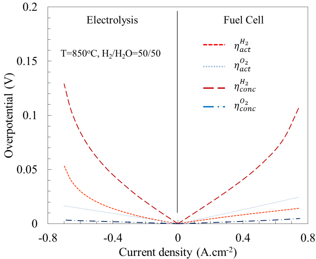
Figure V.10 – Activation and concentration overpotentials obtained with the modelling approach at 850°C, H 2 /H 2 O=50/50 and air. Gas flows were 7.84 10 -5 mol.s -1 and 2.8 10 -4 mol.s -1 for H 2 and O 2 electrode respectively.
