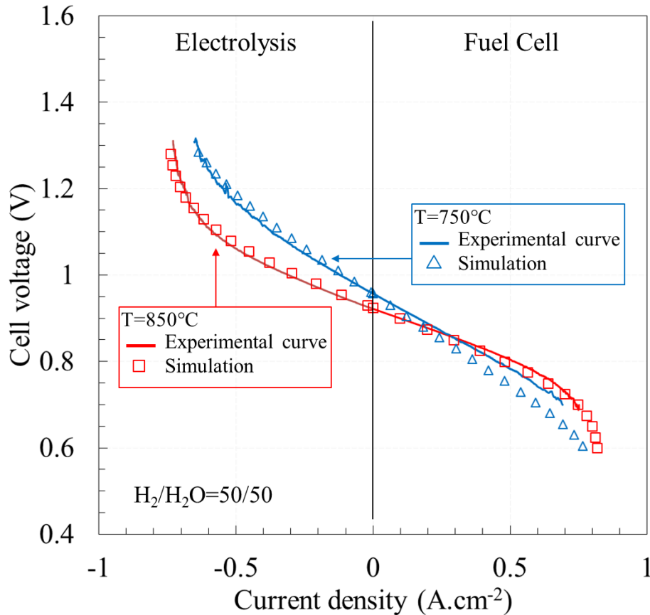
Figure V.8 – Experimental and simulated polarization curves for pristine cells at \text{H}_2/\text{H}_2\text{O}=50/50 , \text{O}_2/\text{N}_2=21/79 and different temperatures. Gas flows were 7.84 \cdot 10^{-5} \text{ mol.s}^{-1} and 2.8 \cdot 10^{-4} \text{ mol.s}^{-1} for \text{H}_2 and \text{O}_2 electrode respectively.
