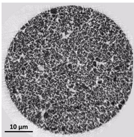
Figure III.13 – Slice extracted from a 3D reconstruction obtained by nano-holotomography of a LSCF-GDC electrode. The two solid phases cannot be satisfactorily distinguished (white=porosity, black=solid phases).
