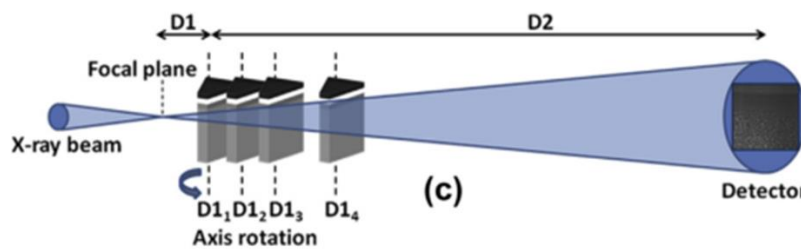
Figure II.3 - Schematic view of holotomography settings [Villanova2013]
