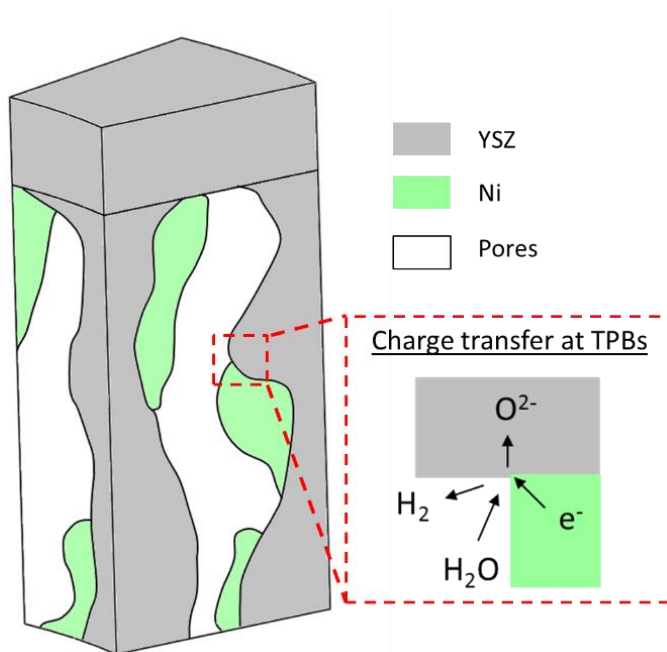
Figure V.2 – Schematic representation of the electrochemical reaction mechanism in electrolysis mode for the hydrogen electrode.
