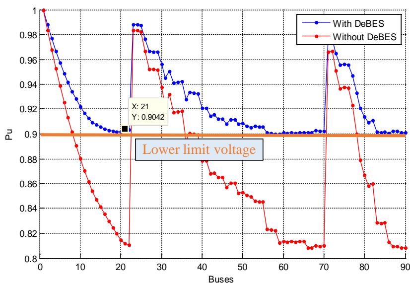
Figure III- 20 : Voltage profile with/without DeBES at time=19h00 (peak load)
