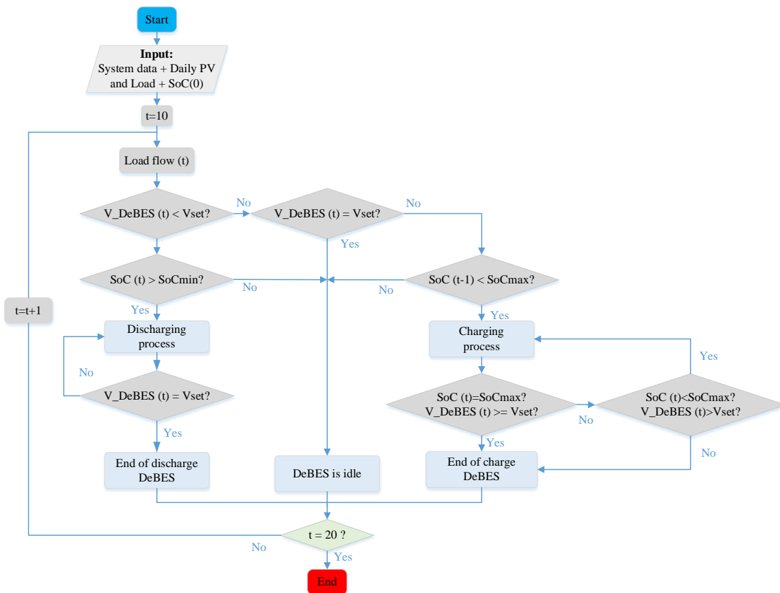
Figure III- 7 : Flowchart of decentralized control of DeBES from 10h00 to 20h00
