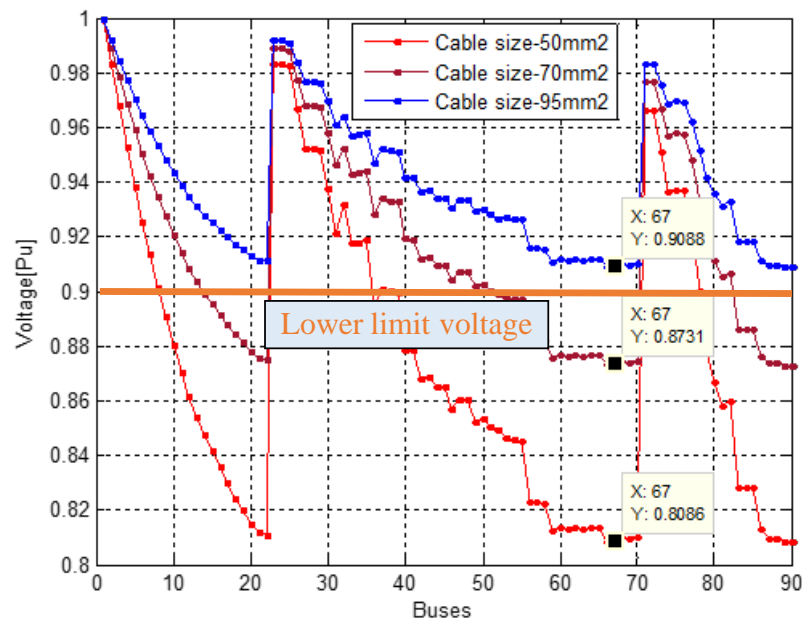
Figure III- 15 :Voltage profile of different cable sizes (50mm2-70mm2-95mm2)
