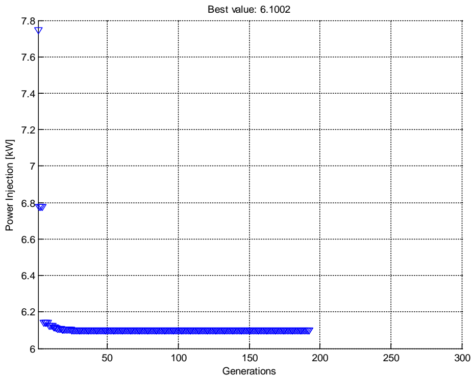
Figure IV-E-3: Evolution of the best DeBES-C location (21) and Sizing at 19h00 over 300 generations setting
