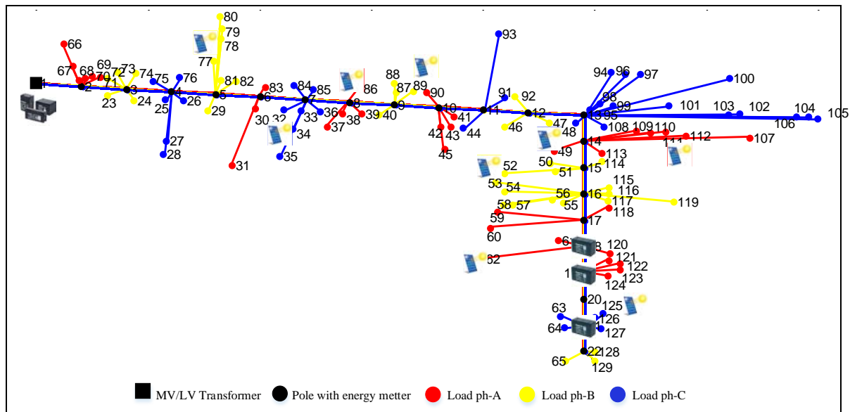
Figure IV- 15 : Radial topology with PV-DeBES-CeBES integration of Sandek village, Bathey, Kampong Cham, Cambodia
