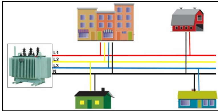
Figure II- 1 : Example of low voltage distribution system in urban areas
