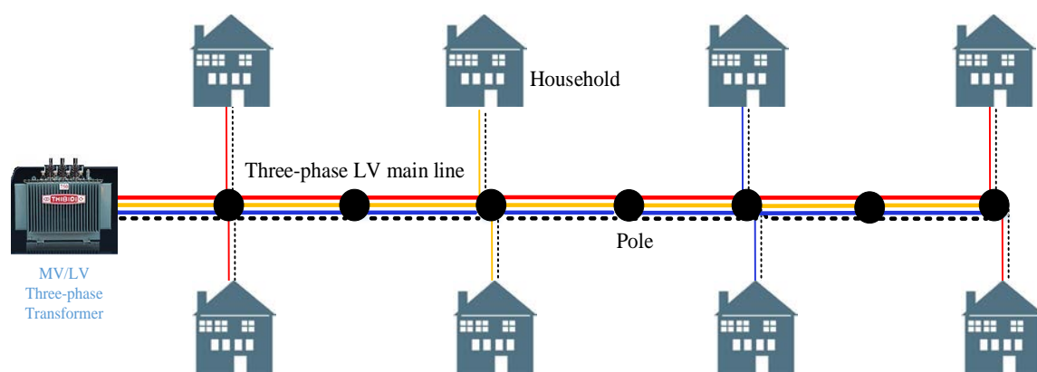
Figure I- 11 : Simple architecture of low-voltage distribution with a three-phase main line in rural area
