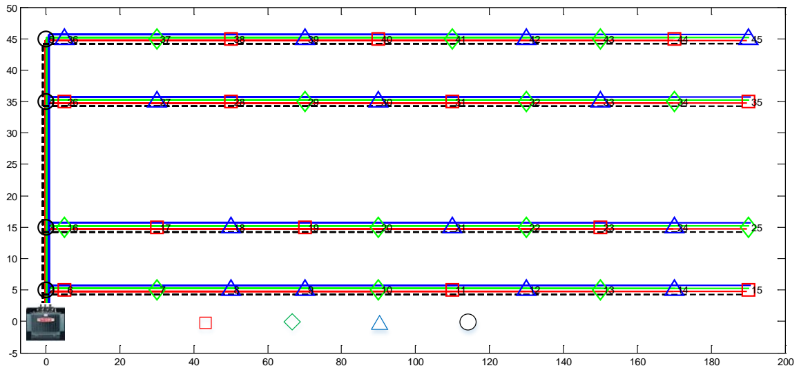
Figure IV- 6 : Optimal topology by SP and FFBP algorithm (Strategy 1)
