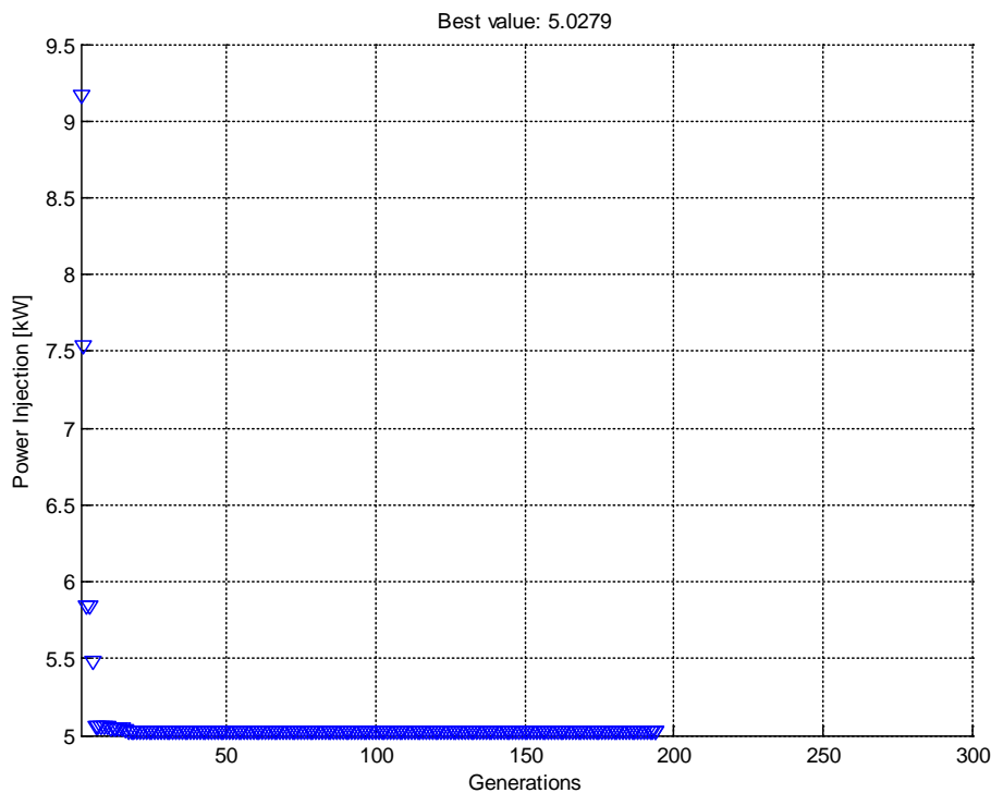
Figure IV-E-1: Evolution of the best DeBES-A location (18) and Sizing at 19h00 over 300 generations setting
