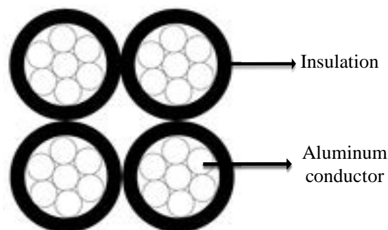
Figure II- 12 : LV-ABC-4Cores Cable
