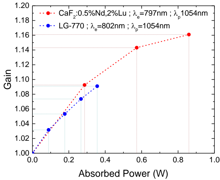
Fig. 4.8 Gain of phosphate glass LG-770 and \text{CaF}_2:0.5\% \text{Nd}, 2\% \text{Lu} as a function of absorbed pump power with probe beam at 1054 nm.
