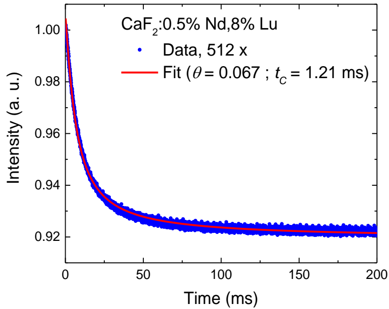
Fig. 3.5 TL measurements and fit of the CaF 2 :0.5% Nd,8% Lu sample.
