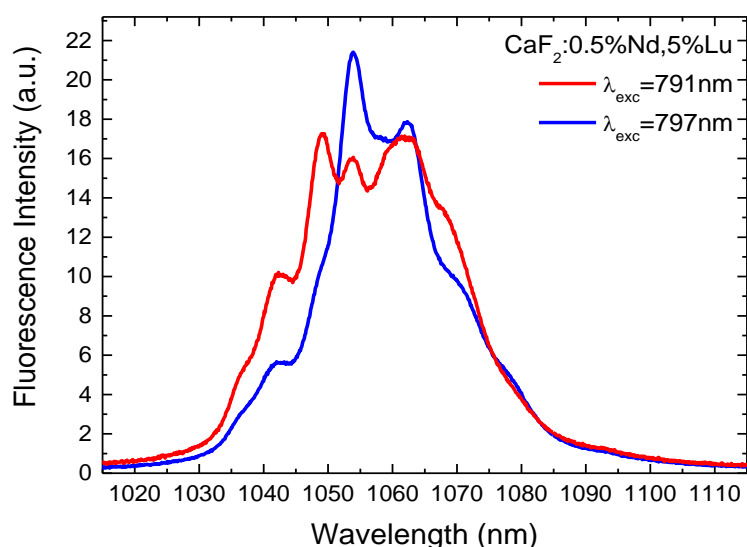
Fig. 2.8 Emission spectra ( {}^4\text{F}_{3/2} \rightarrow {}^4\text{I}_{11/2} transition) of a \text{CaF}_2:0.5\% \text{Nd}, 5\% \text{Lu} sample after excitation at 791 and 797 nm.
