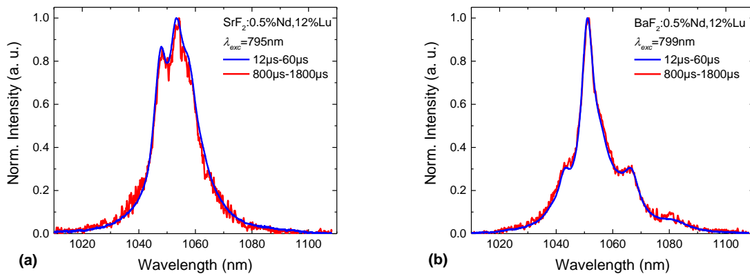
Fig. 2.28 Time-resolved spectra of (a) SrF 2 :0.5% Nd,12% Lu and (b) BaF 2 :0.5% Nd,12% Lu collected within a 'short' time span (12-60 μs) and a 'long' time span (800-1800 μs).
