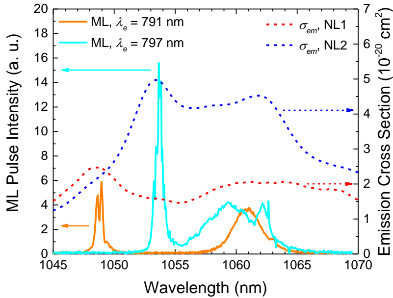
Fig. 4.20 Emission spectra of the mode-locked laser with a CaF 2 :0.5% Nd,5% Lu sample, compared to the emission cross section spectra for NL1 and NL2 centres.
