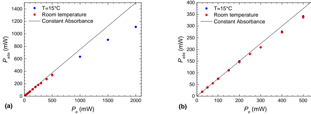
Fig. 4.9 (a) Power absorbed by a 3.7 mm thick \text{CaF}_2:0.5\% \text{Nd}, 12\% \text{Lu} sample versus incoming pump power for a beam with waist radius of 50 \mu\text{m} , without cooling (red diamonds) and with set temperature of 15^\circ\text{C} via chiller (blue dots), and compared to the calculated absorption from absorbance measurements (black line); (b) closeup of the 0-500 mW range.
