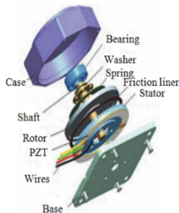
Fig. III-1. Structure diagram of USR60[42]
