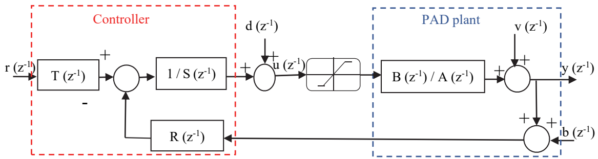
Fig. IV-17. Discrete time PAD plant controlled by RST regulator
