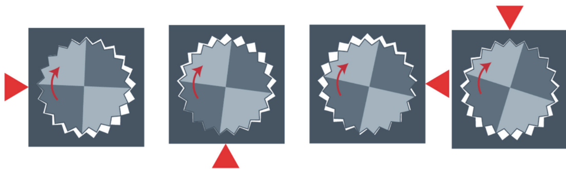
Fig. IV-2. The PAD rotation; The red arrow represents the direction of actuation. The shaft is fixed by a bearing while the ring is free to rotate around it. One revolution of the contact point will cause the motor shaft to step one tooth [139].
