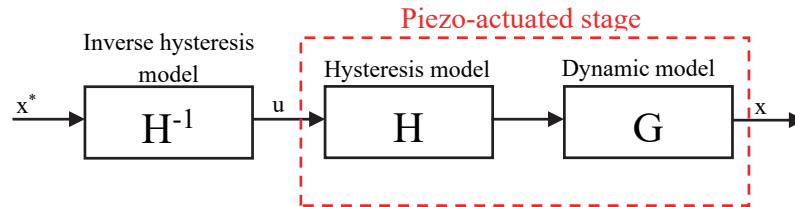
Fig. I-3. Feedforward control of Hysteresis effect
