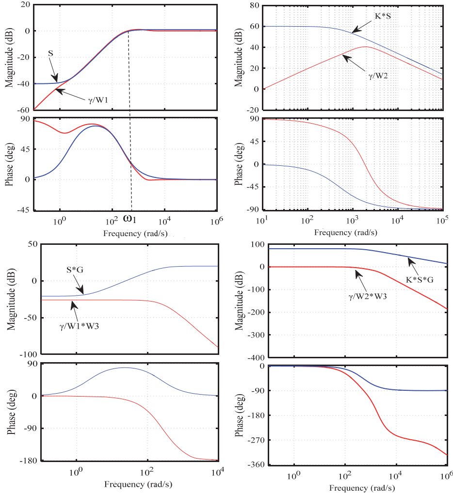
Fig. III-27. Frequency analysis of sensitivity transfer functions
