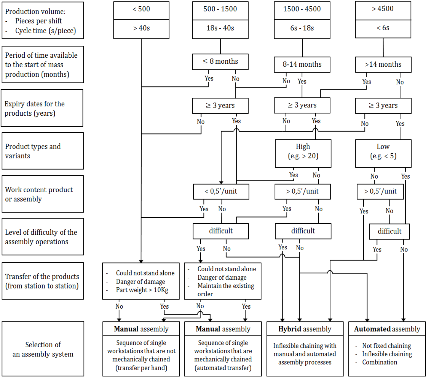
Annex A - Figure 2: The method M2 (Konold & Reger, 2003) description
