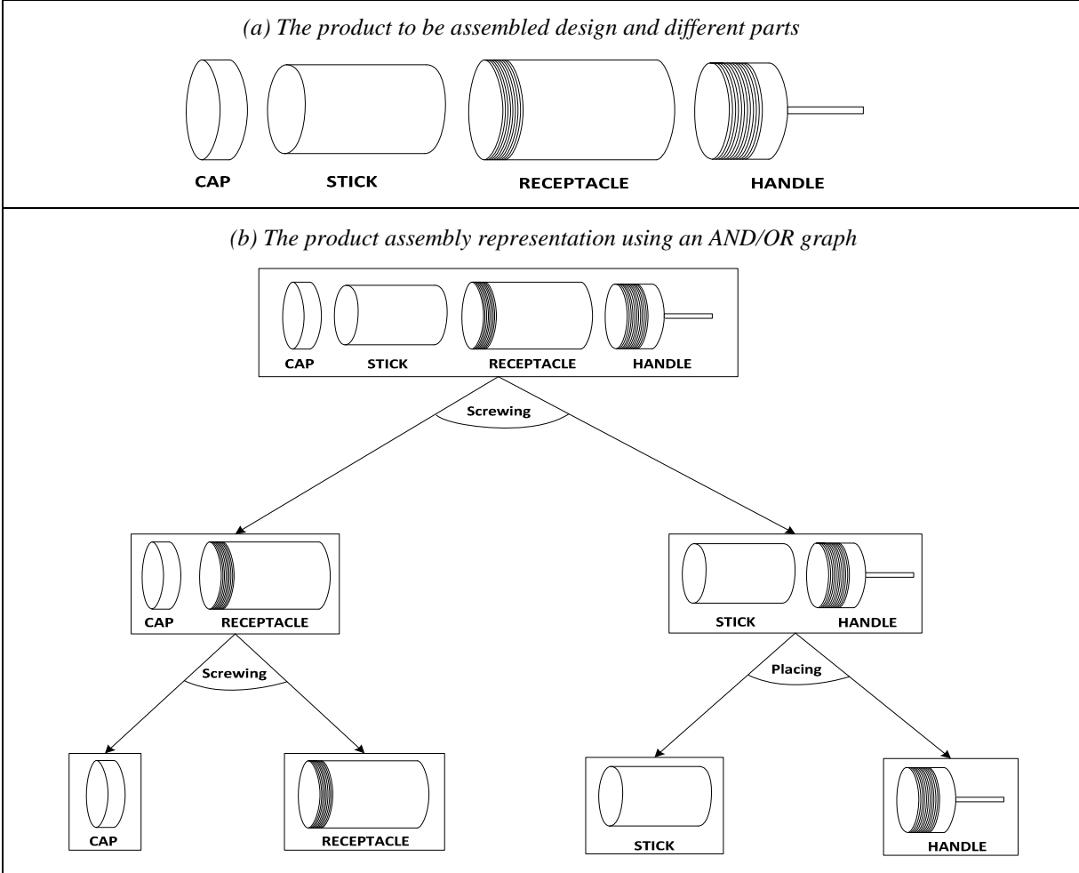
Figure 8: An example of an assembly system alternative
