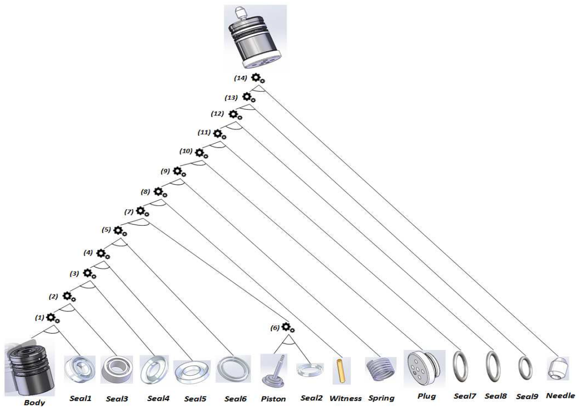
Figure 25: The product assembly sequence representation using an AND/OR graph
