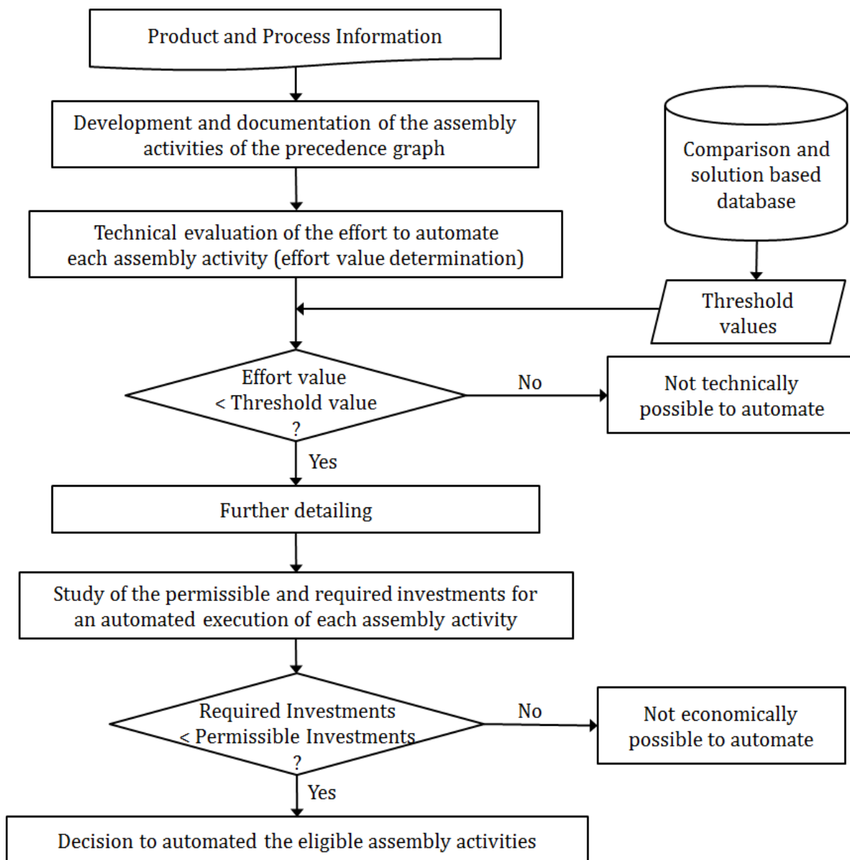
Annex A - Figure 1: The method M1 (Ross, 2002) description
