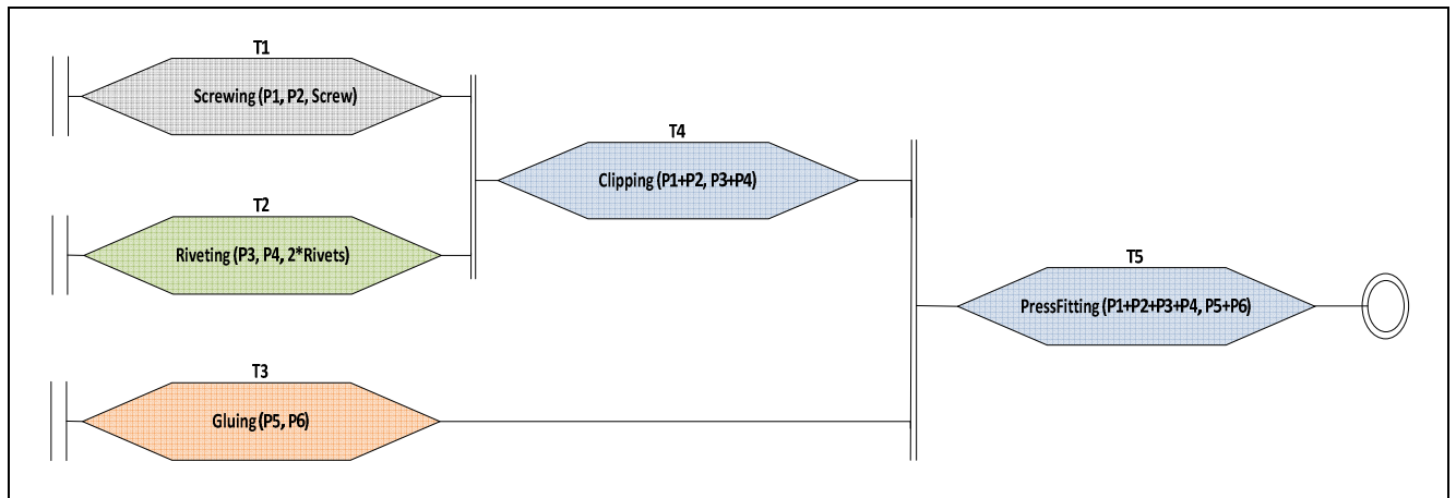
Figure 17: An automation combination to process tasks for a product assembly example
