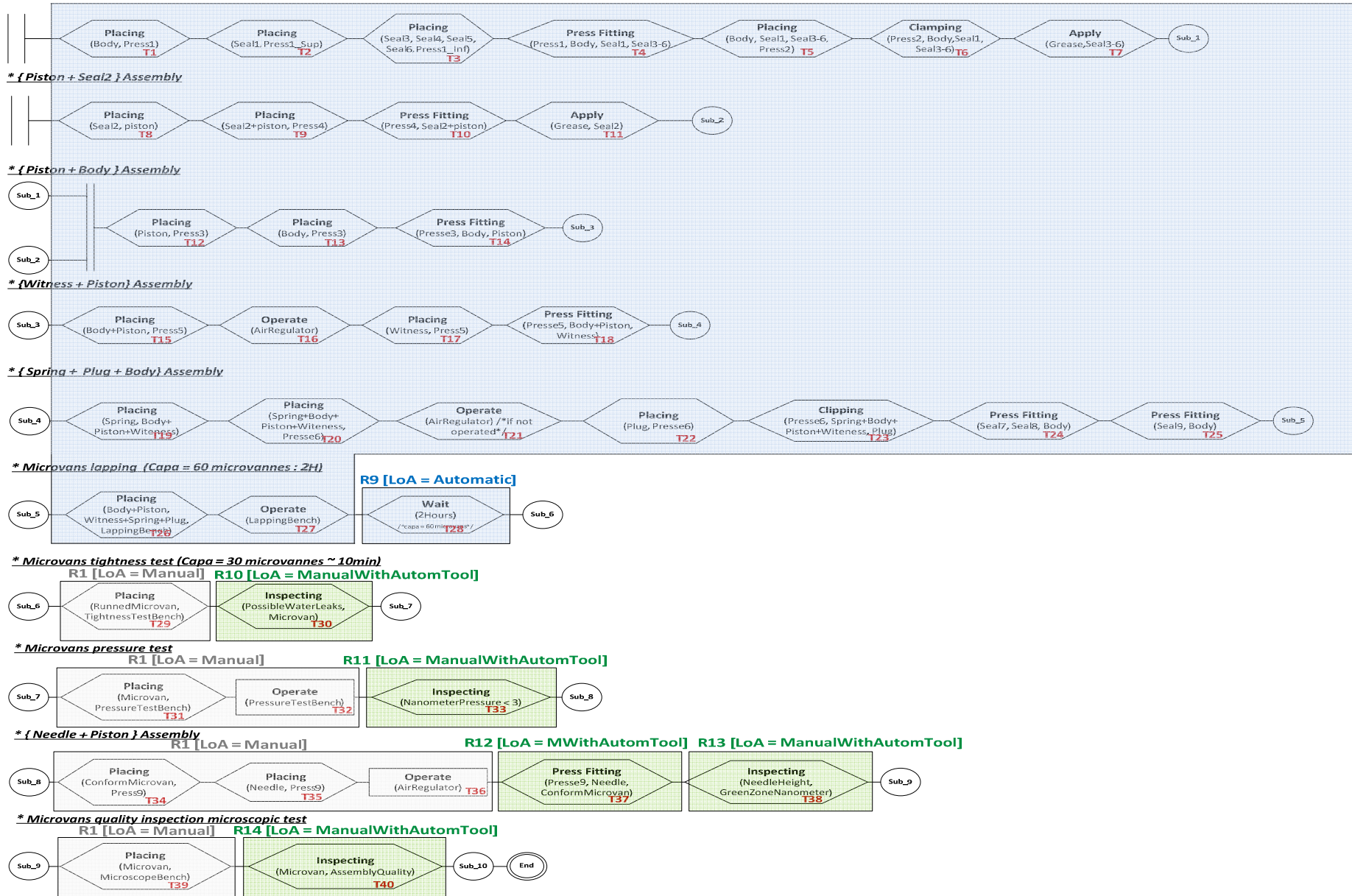
Annex C – Figure 4: A second alternative of a future assembly system: assembly operations automation
