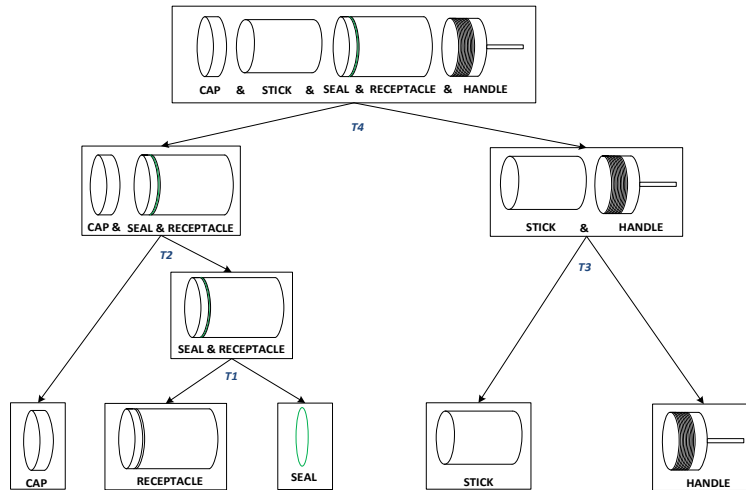
Figure 28: The defined assembly sequence
