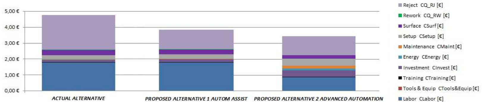
Annex D Figure 1: Obtained assembly costs per product for the different assembly systems alternatives
