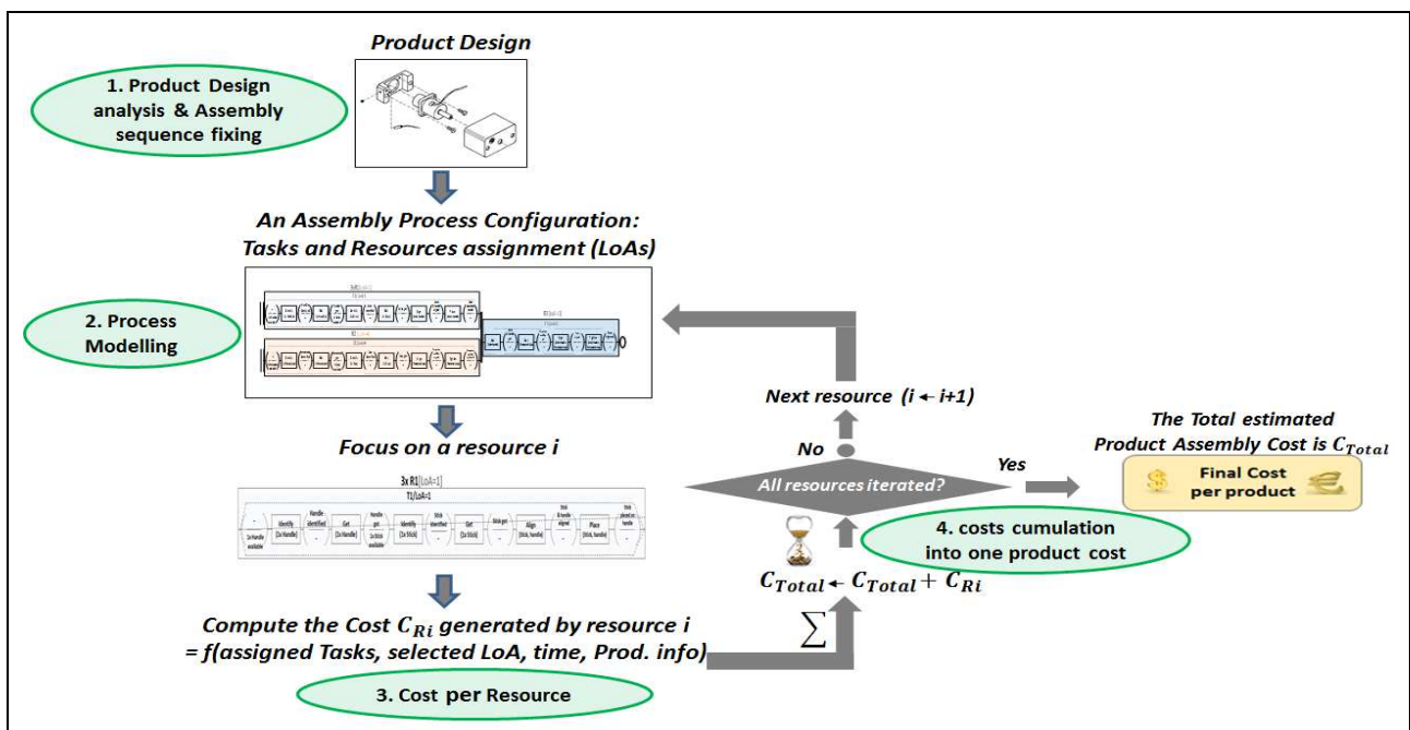
Figure 20: The product assembly cost estimation approach
