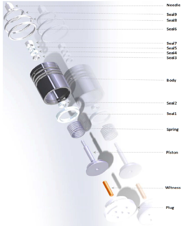
Figure 24: The product components to be assembled
