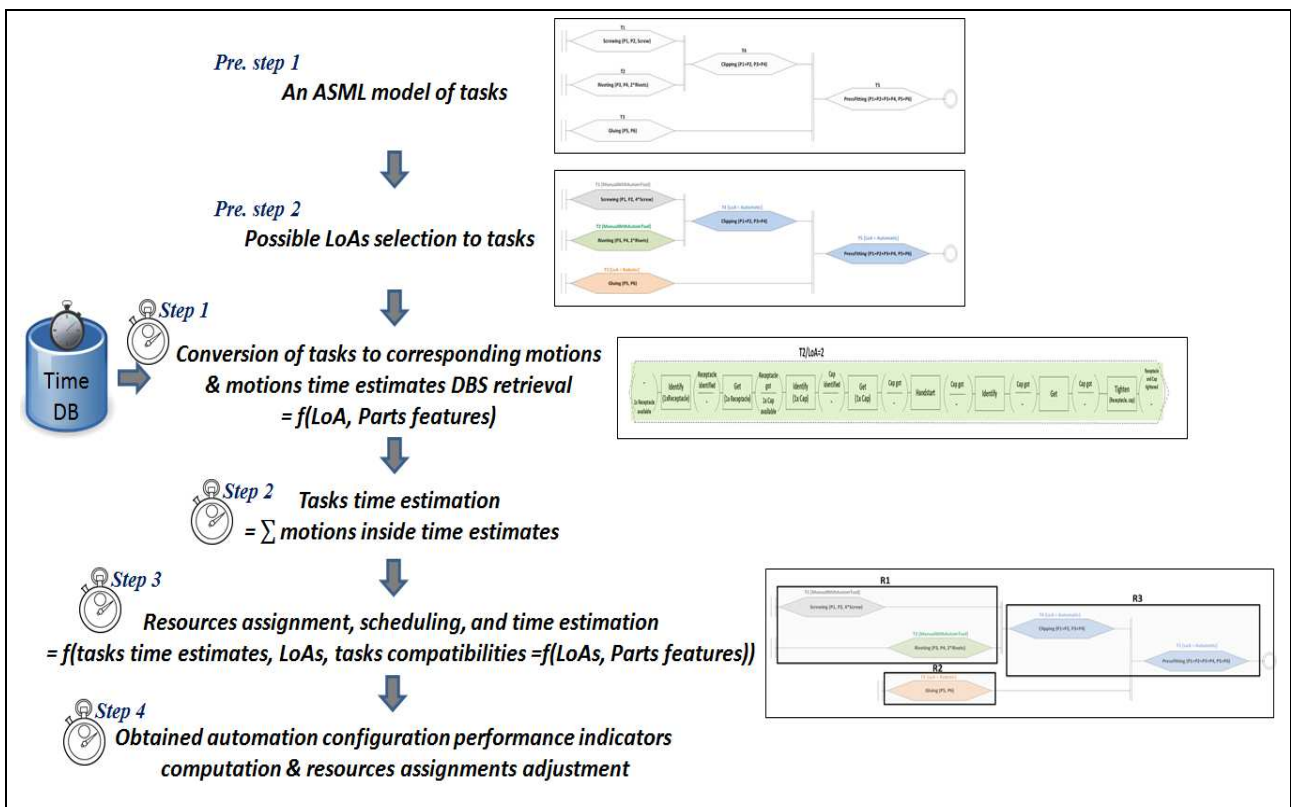
Figure 12: The decomposition of the previously considered automation configuration to motions
