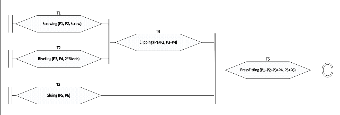
Figure 16: A product assembly example shown by its ASML tasks representation
