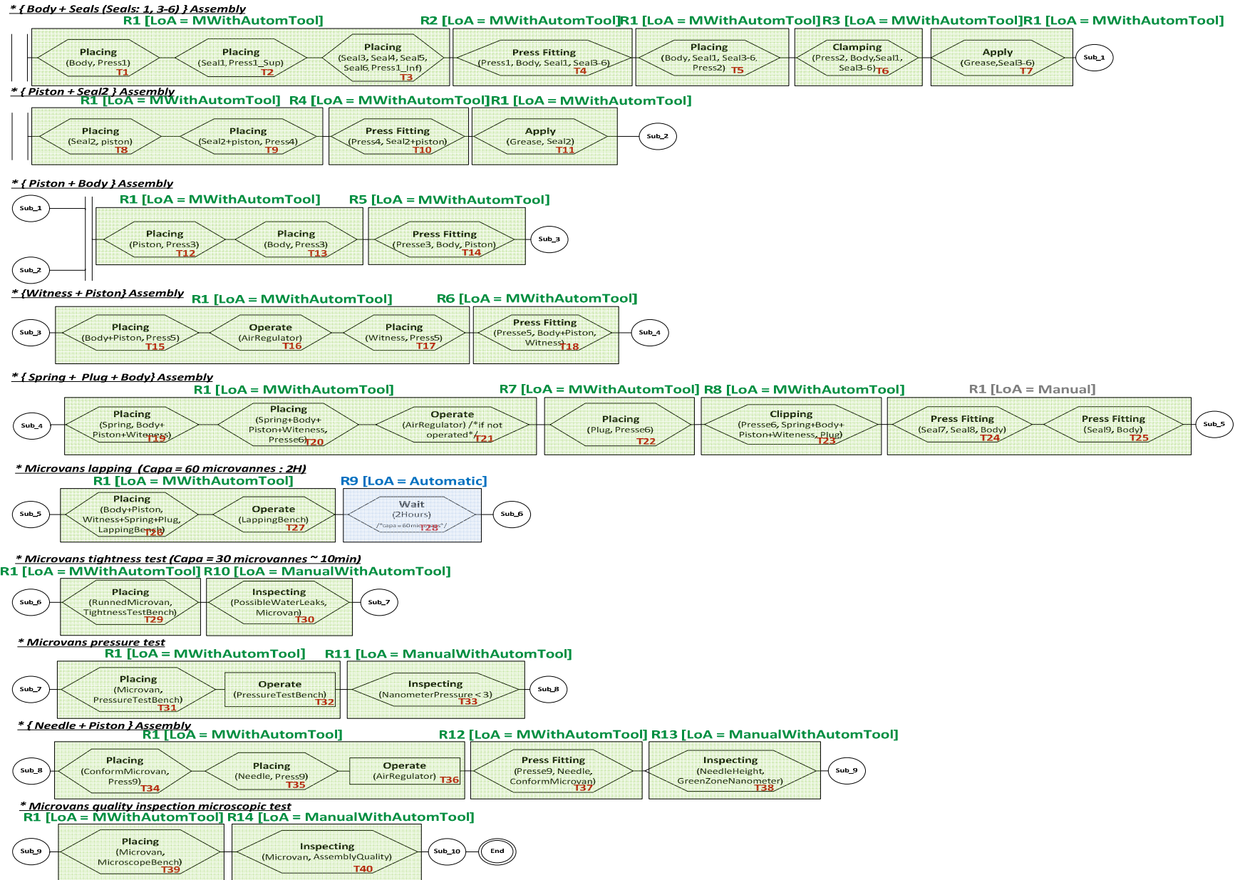
Annex C – Figure 3: The first alternative model: an automated assistance to guide and support operators during assembly
