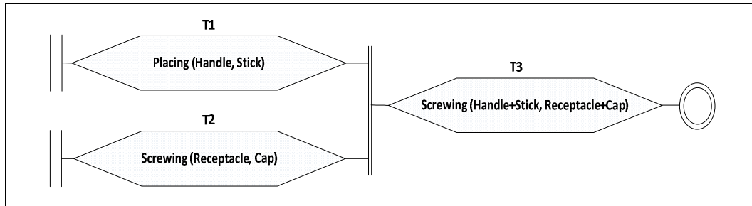
Figure 9: The initial assembly tasks generic representation for the given example
