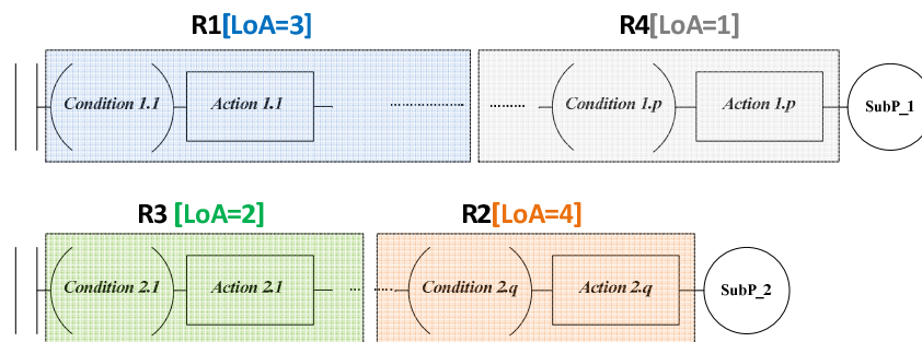
Figure 3: Resources representation in ASML
