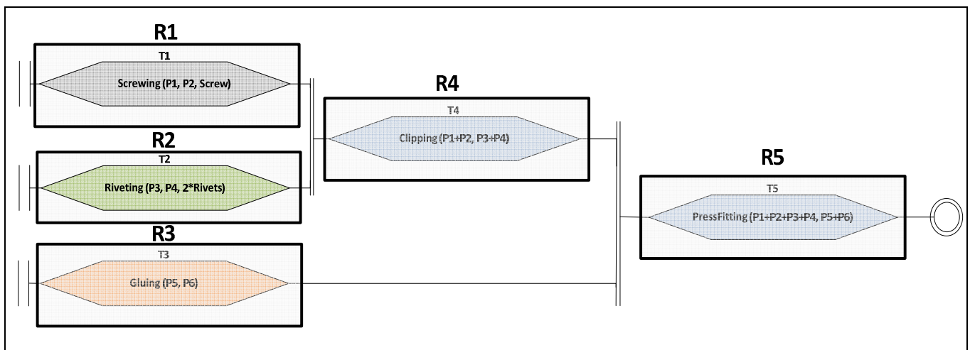
Figure 18: An alternative of resources assignments to tasks
