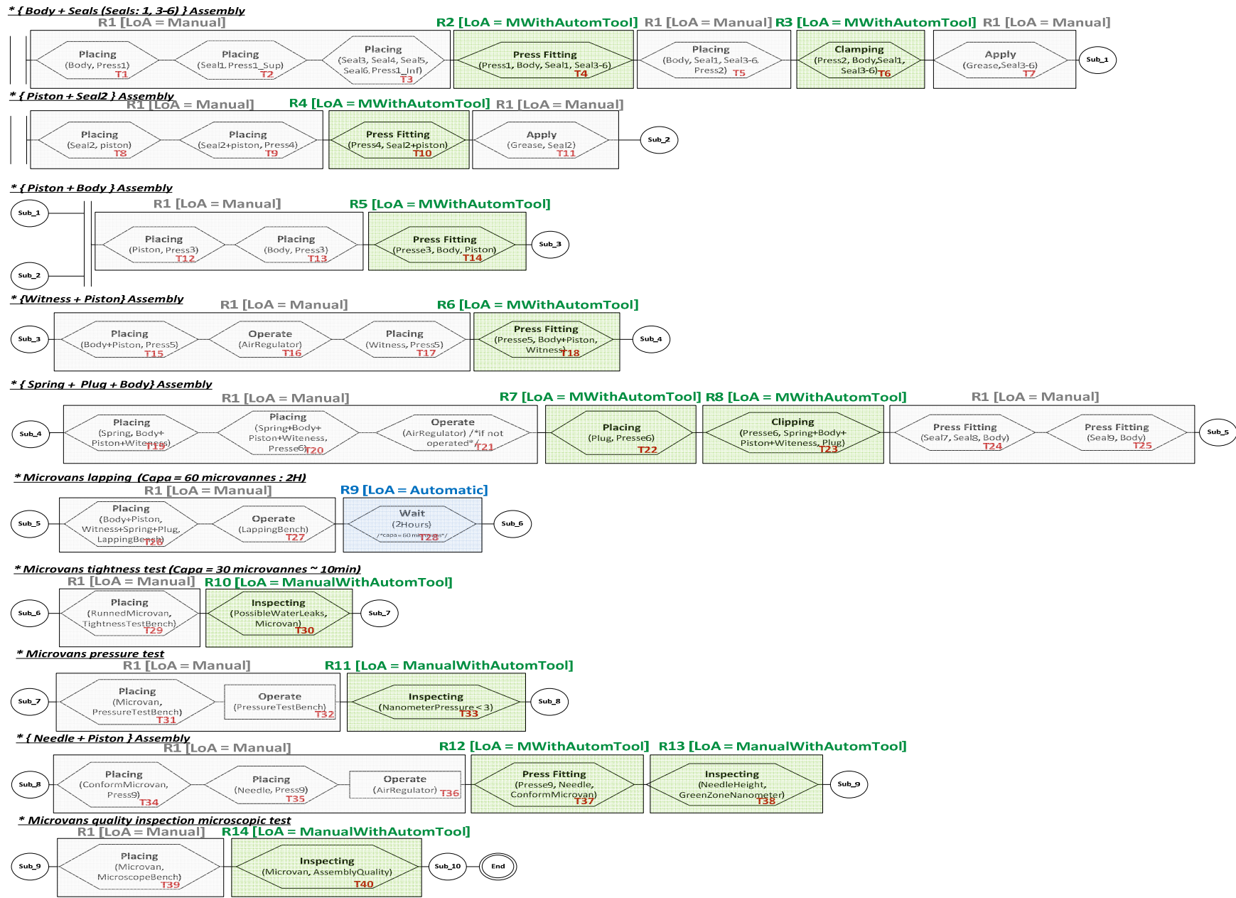
Annex C – Figure 2: The current assembly system model: an alternative with a minimum of investment
