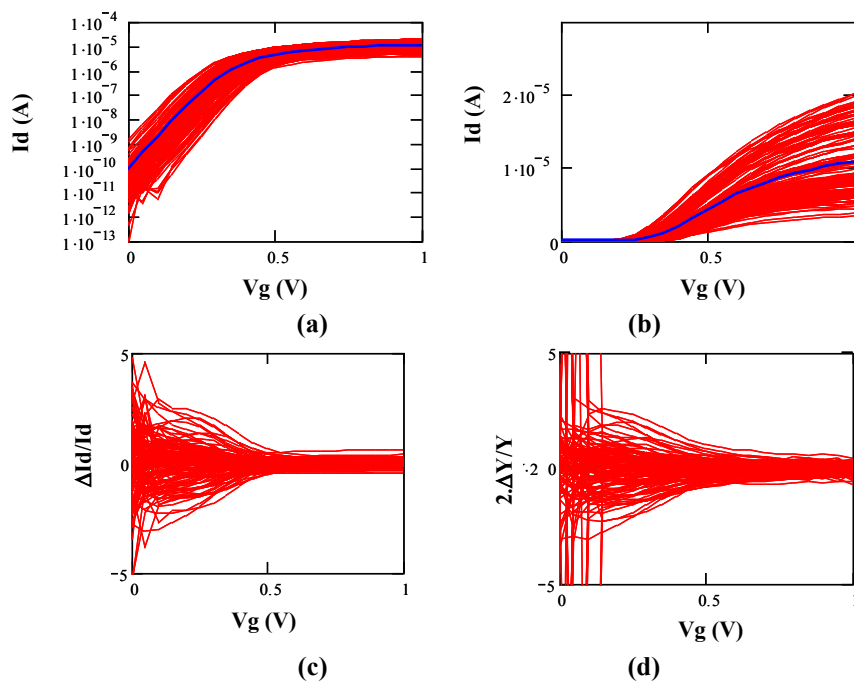
Figure V-23 Typical set of I_d(V_g) , \Delta I_d/I_d(V_g) and 2 \cdot \Delta Y/Y(V_g) curves for n-MOS FinFETs with N_{fin}=2 and L=28 nm. Bold blue line shows the mean value of I_d(V_g) characteristics.
