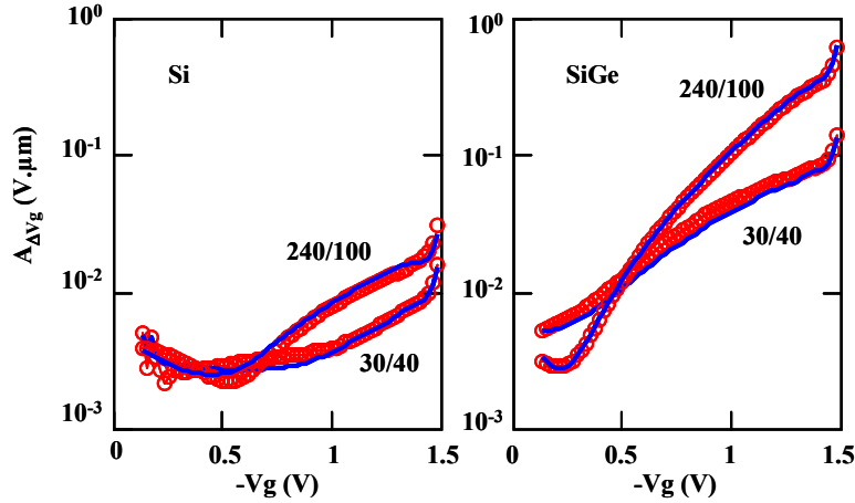
Figure V-16 Experimental (symbols) and modeled (solid lines) variations of i\Delta I_{\Delta V_g} with V_g for Si and SiGe p-MOSFETs (W/L in nm).
