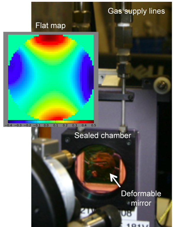
FIG. 4.— 2k DM mounted in the SCEXAO instrument. The gas supply lines to the sealed chamber can be seen along with the gold surface of the DM itself. Inset: The map applied to the DM in order to compensate for the DM surface figure. The map shows the magnitude of the modulation of the actuators in microns. The window is 50 actuators in diameter corresponding to the functioning region of the DM. The map required to flatten the DM surface is dominated by the Zernike which represents astigmatism.
