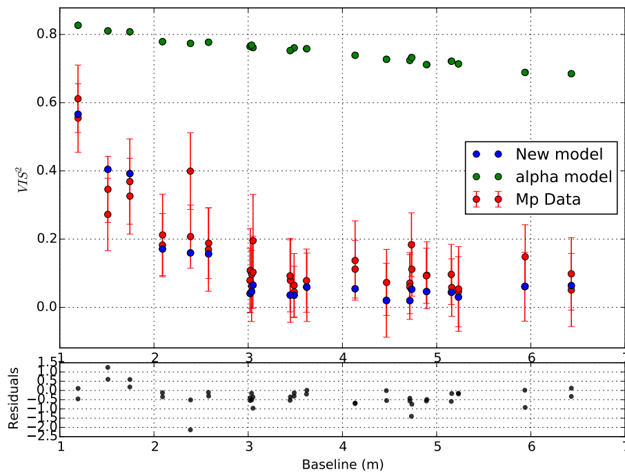
Figure 3.15: Same as Figure 3.13 but for Mp-band VIS2 data.
