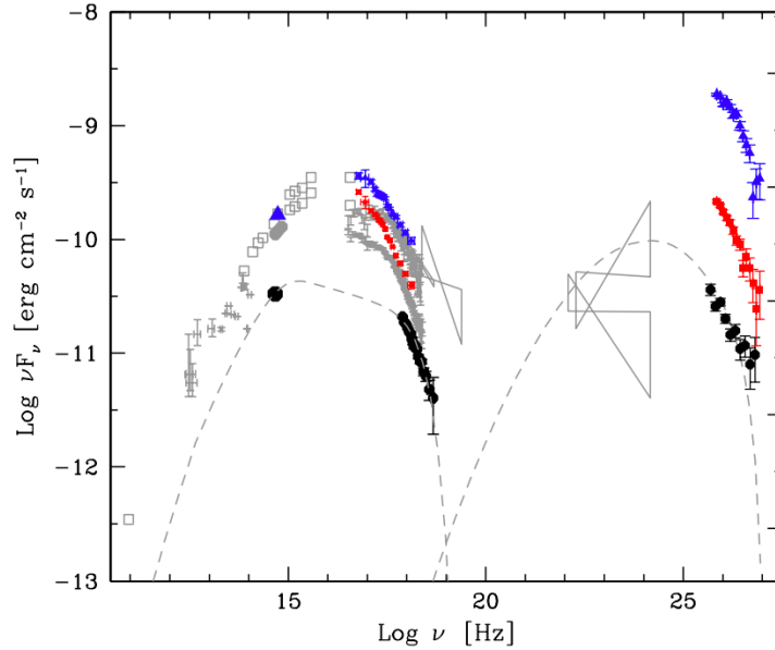
FIGURE 2.9: SED of PKS 2155-304 showing the lowest (red) and highest (blue) states of the flare. The black data are 2003 data of the quiescent state (Aharonian et al., 2009a).
