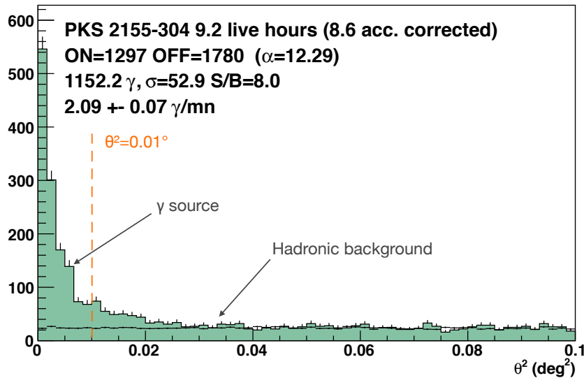
FIGURE 4.20: Events distribution versus the square of the angular distance from the pointing position (also called Theta 2 plot) for observations towards PKS 2155-304. The point source cut used for extragalactic observations is set at 0.01 \text{ deg}^2 .
