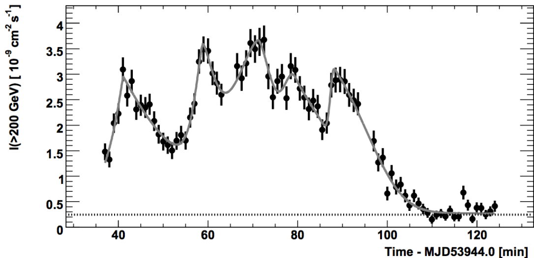
FIGURE 9.1: Light curve of the 2006 flare of PKS 2155-304 caught by H.E.S.S. (Aharonian et al., 2007a). Flux points are computed in 1 min bins. The dotted line represents, for comparison the flux of the Crab and the curve is the fit (five bursts and a constant flux).
