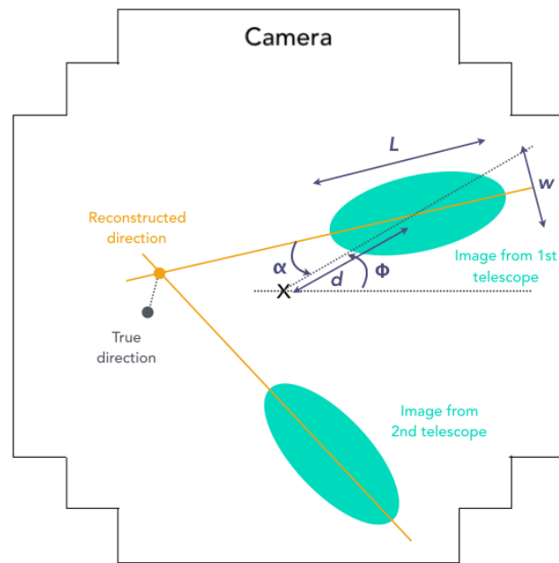
FIGURE 4.11: Hillas parametrisation.
