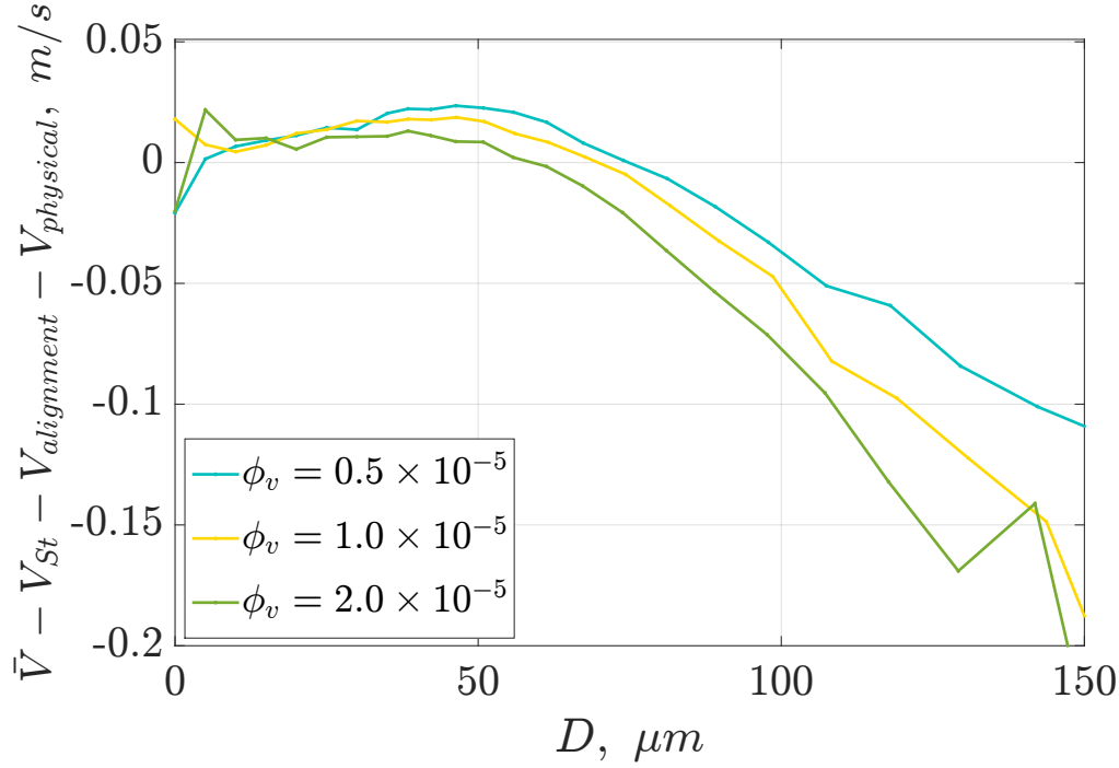
FIGURE 6.17: Settling velocity \bar{V} - V_{alignment} - V_{St} - V_{physical} m/s vs D of all measured particles, positive V is defined downwards
