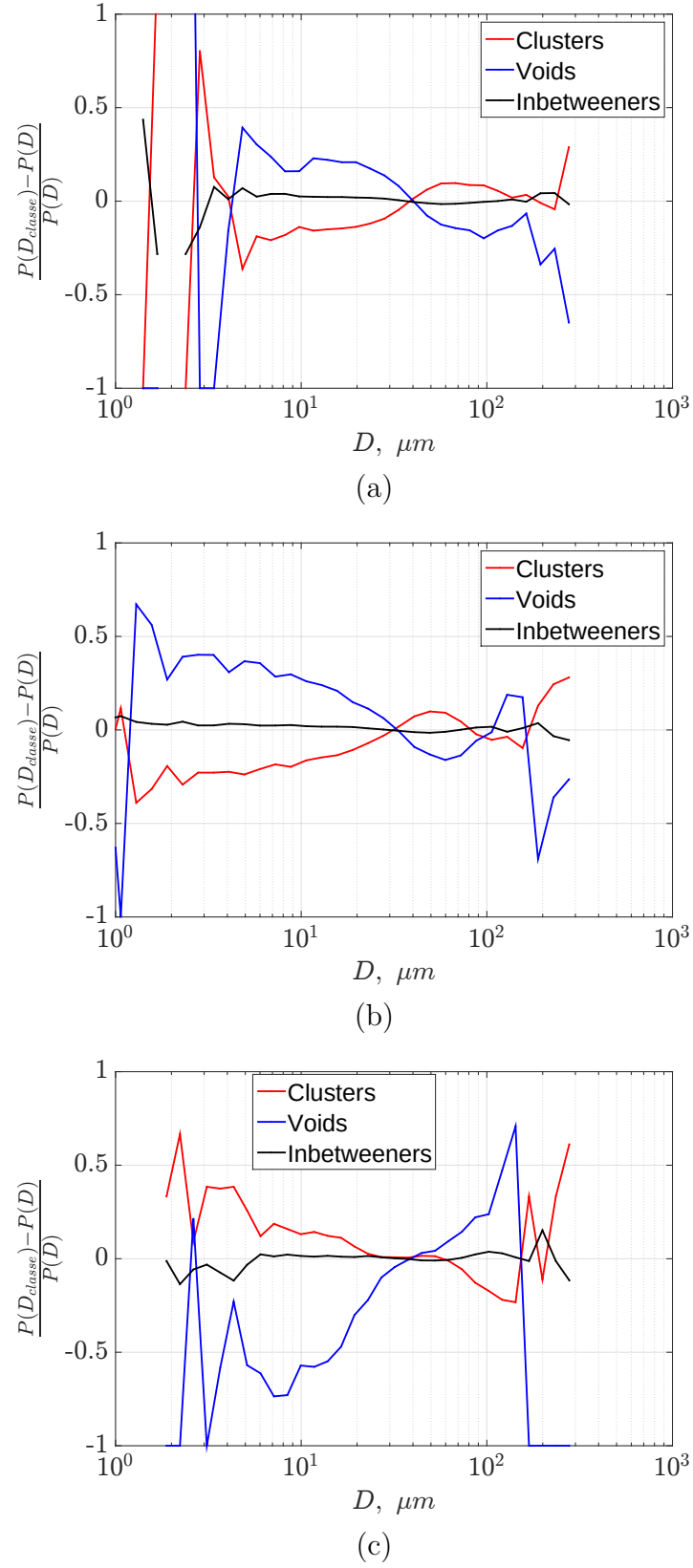
FIGURE 6.40: Quantity \frac{P(D_{classe}) - P(D)}{P(D)} vs D investigated for three experimental conditions: (a) \phi_v = 0.5 \times 10^{-5} , (b) \phi_v = 1.0 \times 10^{-5} and (c) \phi_v = 2.0 \times 10^{-5}
