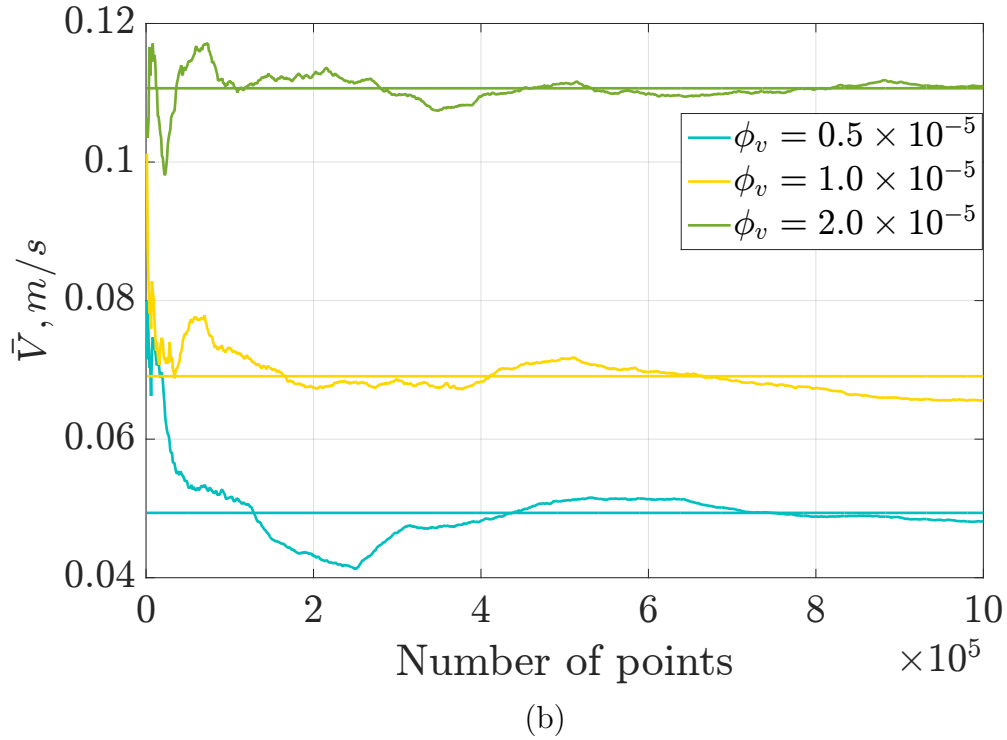
FIGURE 3.12: Convergence plots of mean velocity of (a) axial U (b) settling V
