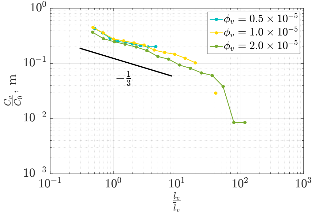
FIGURE 6.50: Concentration in voids \frac{\bar{C}_v}{\bar{C}_0} versus the length of voids l_v for three experimental conditions
