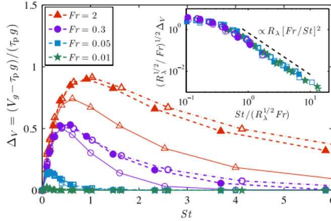
FIG. 2 (color online). Relative increase of the settling velocity \Delta V as a function of the Stokes number St for various Froude numbers, as labeled, and Re_\lambda = 130 (thin symbols, plain lines), Re_\lambda = 290 (filled symbols, dashed lines), and Re_\lambda = 460 (open symbols, broken lines). Inset: [Re_\lambda^{1/2} / Fr]^{1/2} \Delta V as a function of St / [Re_\lambda^{1/2} Fr] for the same data.
