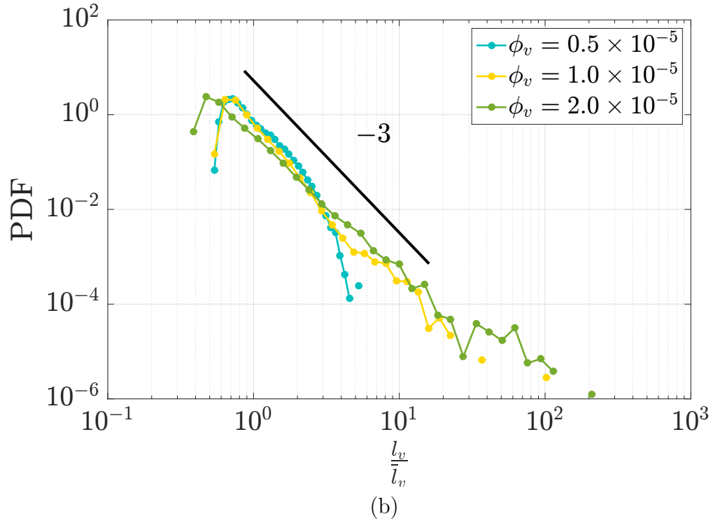
FIGURE 6.48: PDFs of length of voids (a) l_v and (b) \frac{l_v}{\bar{l}_v} for three experimental conditions
