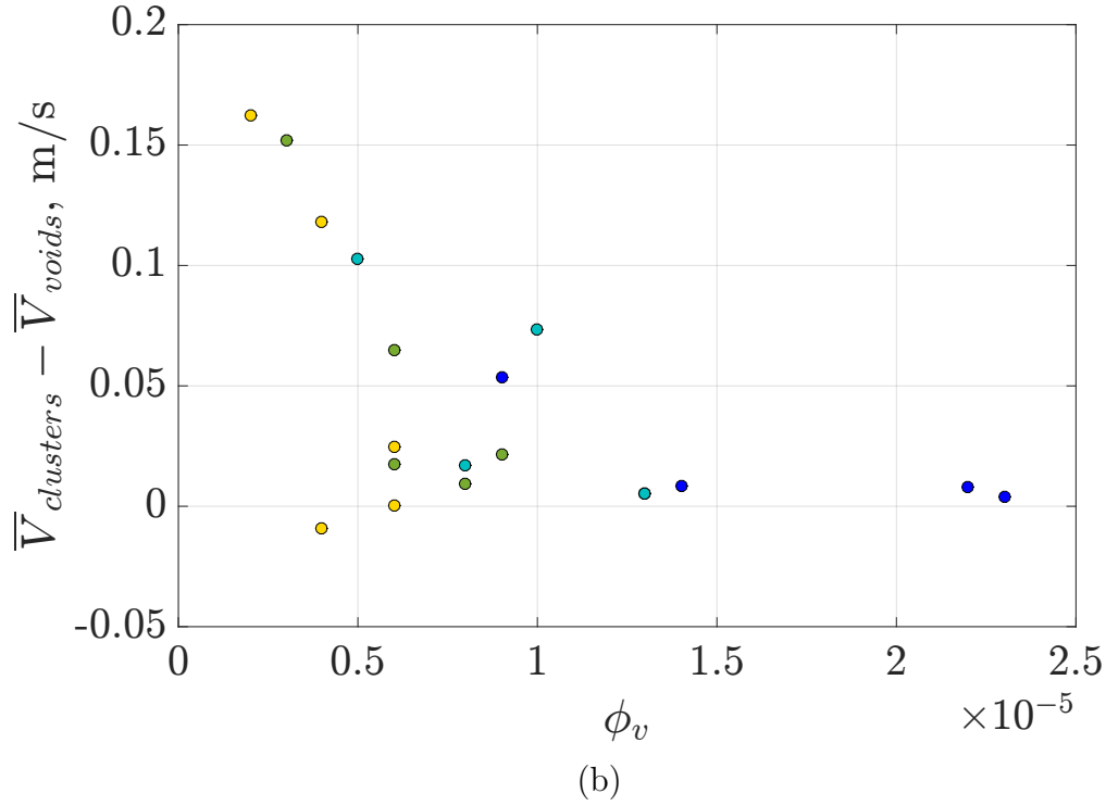
FIGURE 5.7: Difference between clusters and voids \bar{V}_{clusters} - \bar{V}_{voids} plotted versus (a) Re_\lambda (volume fraction \phi_v decreases both vertically and from right to left of the Re_\lambda ). and (b) \phi_v , the colors are attributed as follows: blue for Re_\lambda = 175 , light blue for Re_\lambda = 250 , green for Re_\lambda = 350 , yellow for Re_\lambda = 450 .
