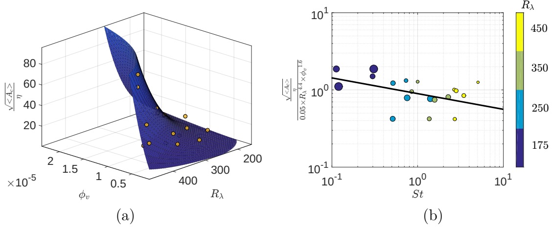
FIGURE 4.11: a). Scalings of \frac{\sqrt{\langle A_v \rangle}}{\eta} vs \phi_v and R_\lambda b). Reducing the original function of \frac{\sqrt{\langle A_v \rangle}}{\eta} shows the weak dependence on St
