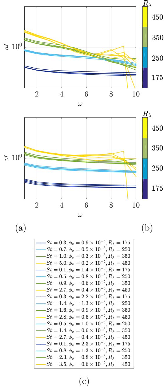
FIGURE 5.1: (a) u' vs tracks length \omega , (b) v' vs tracks length \omega . Note that \omega here is given in units of a frame number. (c) Experimental parameters corresponding to a) and b)
