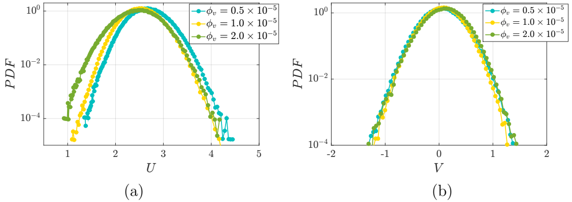
FIGURE 6.3: (a) Probability density function of axial U velocity (b) Probability density function of V_{settling} (raw data), positive V is defined downwards. Data for all particle sizes.
