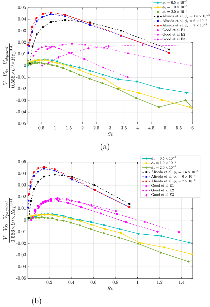
FIGURE 6.27: Scalings of settling velocity \frac{V - V_{St} - V_{physical}}{0.556 \times U_I \times Re_L^{0.41}} vs (a) St and (b) Ro
