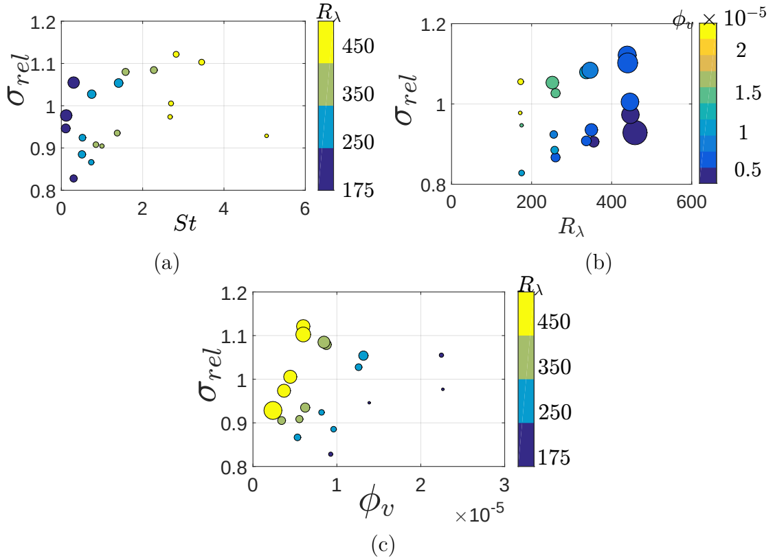
FIGURE 4.7: (a) Standard deviation \sigma vs St . Symbol colors represent the Reynolds number, while the size of the symbols encodes the volume fraction (larger symbols correspond to experiments at larger volume fraction). (b) Standard deviation \sigma vs Re_\lambda . Symbol colors indicate the volume fraction, while the size of the symbols encodes the Stokes number (larger symbols correspond to experiments with larger Stokes numbers). (c) Standard deviation \sigma vs \phi_v . Symbol colors reflect the Reynolds number, while the size of symbols encodes the Stokes number (larger symbols correspond to experiments with particles at larger Stokes number).
