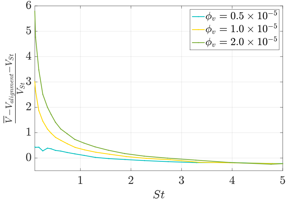
FIGURE 6.18: Corrected with alignment settling velocity \frac{\bar{V} - V_{\text{alignment}} - V_{St}}{V_{St}} vs St of all measured particles
