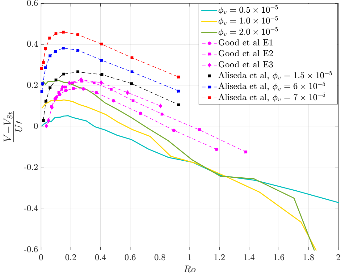
FIGURE 6.26: \frac{V-V_{St}}{U'} vs Ro for present and previous studies
