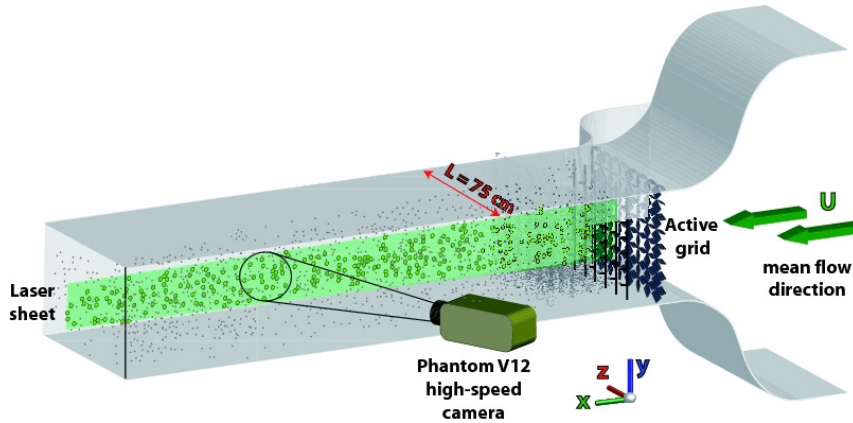
FIGURE 3.3: Schematic view of the experimental facility.
