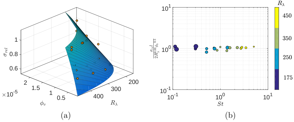
FIGURE 4.8: (a) \sigma_{rel} as a function of \phi_v and Re_\lambda with a power law fit \sigma_{rel} \propto Re_\lambda^\beta \phi_v^\gamma . (b) \sigma_{rel} compensated by Re_\lambda^\beta \phi_v^\gamma . Best fit is obtained for \beta \simeq 0.88 and \gamma \simeq 0.5 .
