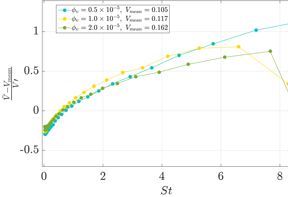
FIGURE 6.21: Settling velocity \frac{\bar{V} - V_{mean}}{V_I} vs St of all measured particles
