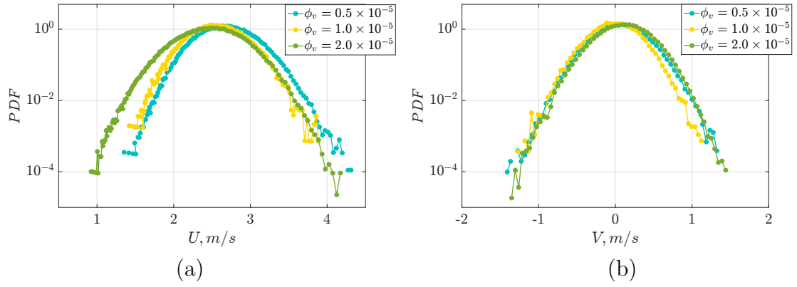
FIGURE 6.5: (a) Probability density function of axial U velocity for small particles (b) Probability density function of V_{settling} for small particles (raw data), positive V is defined downwards
