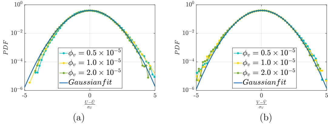
FIGURE 6.4: (a) PDF of centered and normalised axial U velocity (b) PDF of centered and normalised V_{\text{settling}} . Data for all particle sizes.
