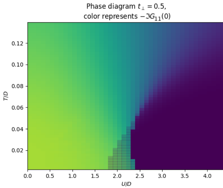
Figure 3.30: IPT phase diagram established by the spectral density at the Fermi energy. Coexistence region narrows in comparison to the t_{\perp} = 0.3 case and drifts to even lower values of U (cf. Fig.3.31).
