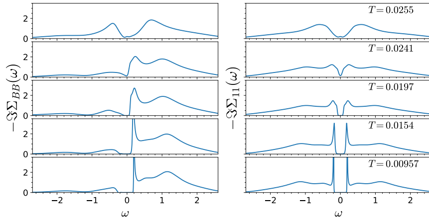
Figure 3.33: Change of the self-energy with temperature. The pole inside the Mott gap is broadened until disappearance. There is no connection between metal and insulator self-energy, their structures change drastically. Transition from a Mott insulator to a Fermi liquid
