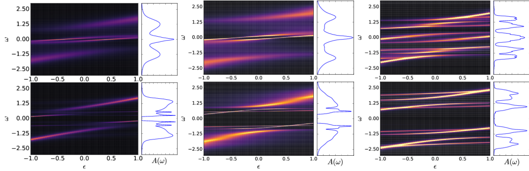
Figure 3.12: Comparison of the electronic structures in the Metal and Insulator phases at t_{\perp} = 0.3 . Left CT-QMC in the coexistence U = 2.15 , center IPT taken from main text U = 2.5 , right results from ED metal at U = 1.8 , insulator at U = 3
