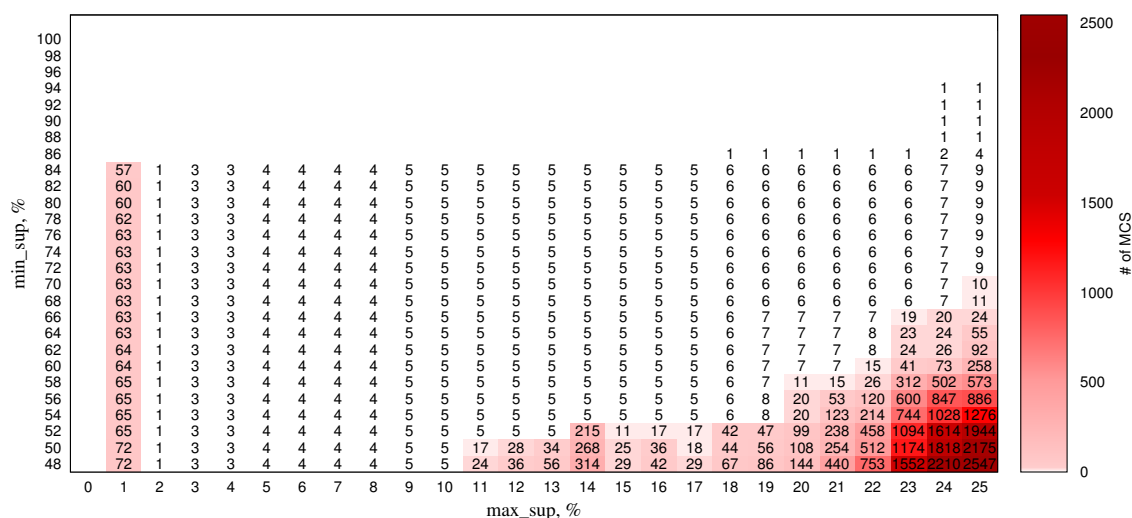
FIGURE 5.13: The number of minimal contrast sequences mined for the DVBTesT use case (with max\_length = 3 ).
