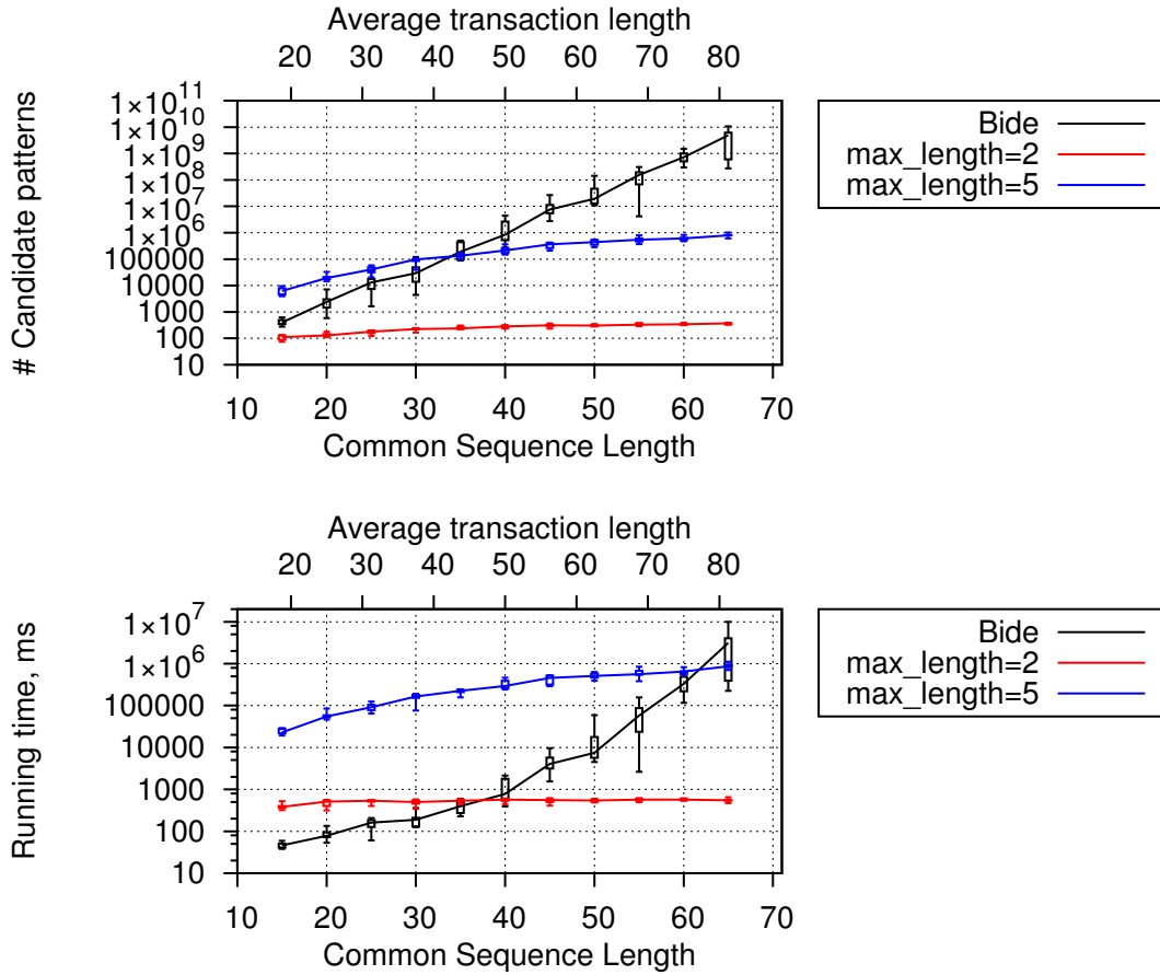
FIGURE 4.10: Comparison of the computational complexity of the Bide algorithm and of the SATM algorithm (tested with various max_length values) run on the same synthetic traces described in Figure 4.6
