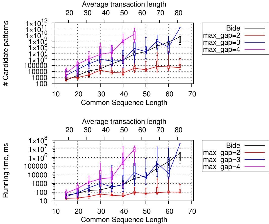
FIGURE 4.9: Comparison of the computational complexities of the Bide algorithm and of the ConSGapMiner algorithm (tested with various max_gap values) run on the same synthetic traces described in Figure 4.6 7 .
