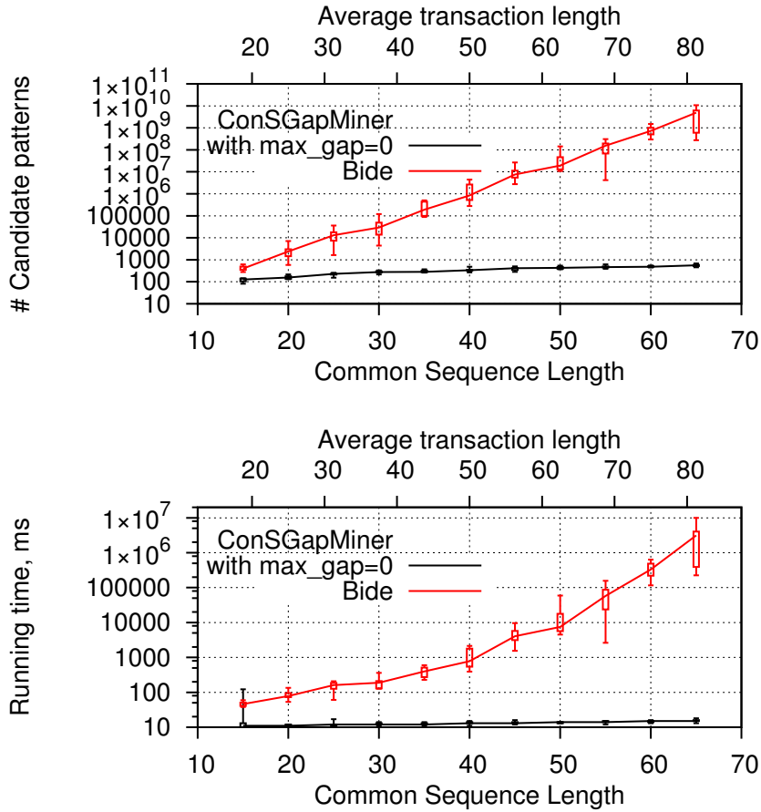
FIGURE 4.8: Comparison of the computational complexities of the Bide algorithm and of the ConSGapMiner algorithm with max\_gap fixed at 0 run on the same synthetic traces described in Figure 4.6
