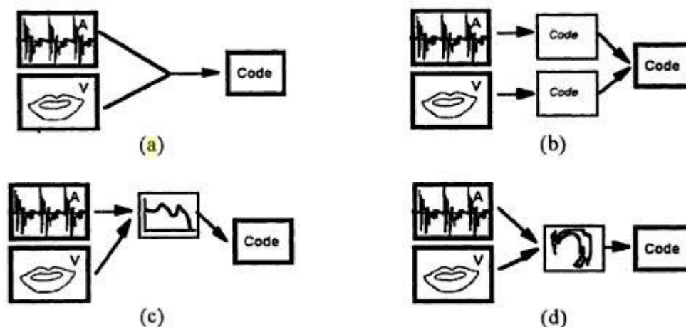
Figure 1-3 The four basic models of AV integration. a) Direct Identification (DI), b) Separate Identification (SI), c) Dominant Recoding (DR), d) Motor Recoding (MR). Taken from (Schwartz et al. , 1998).
