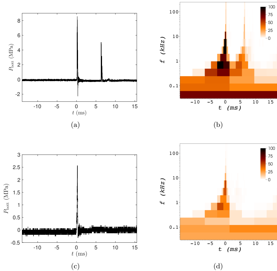
FIGURE 2.10: Left: Pressure signal at the bottom of the reactor obtained for d = 0 . Right: Daubechies wavelet of the pressure signal presented in (a) and (c). Up: H_0 = 20 mm and Down: H_0 = 8 mm. The color bar represents the absolute values of the wavelet coefficients, which represent a measure of the signal intensity.
