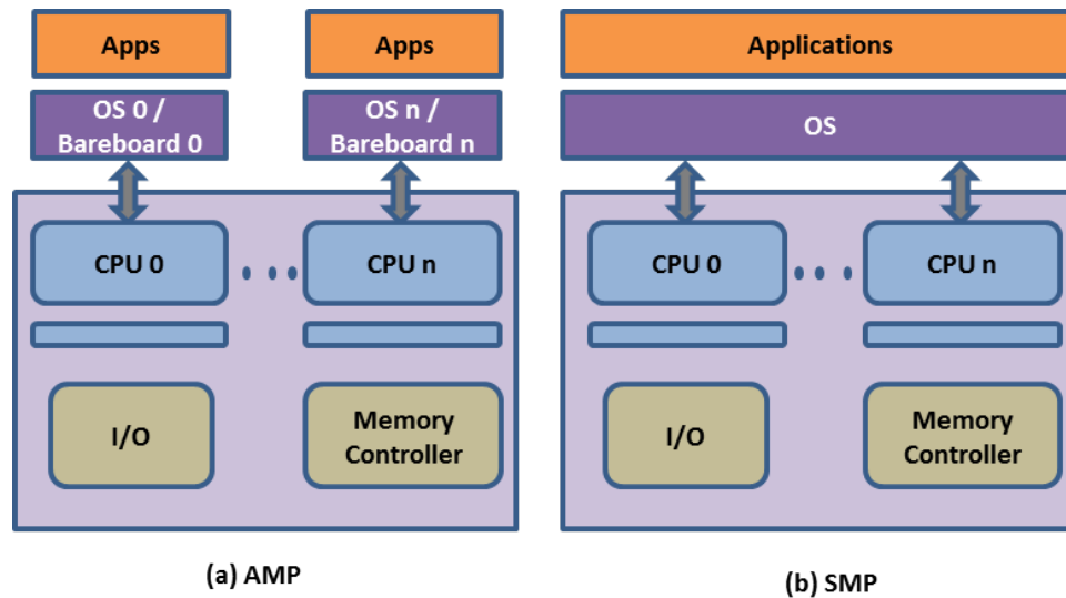
Figure 2.6: AMP and SMP modes
