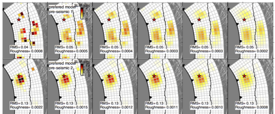
290 291 Figure S8: Pre-seismic slip distribution for different model roughnesses. Top: 8 months 292 pre-seismic (july 2013 – mid-March 2014), Bottom: 15-day pre-seismic (Mid-March to 293 End March 2014). 294
