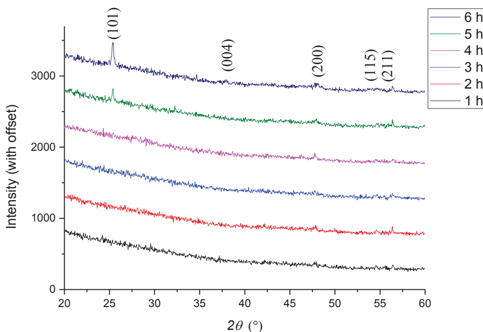
Fig. 3-15 High-temperature XRD analysis heating silicon-supported \text{TiO}_2 thin film at 300 °C with duration till 6 h.
