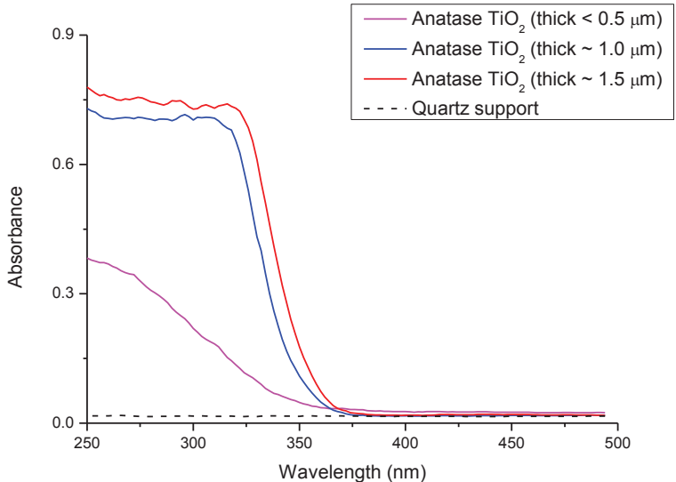
Fig. 3-28 Light absorbance of 400°C-annealed anatase TiO 2 films deposited on quartz.
