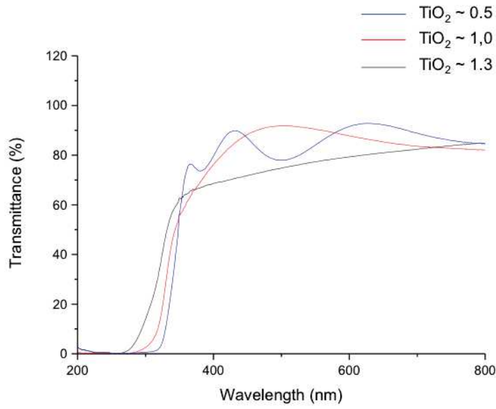
Fig. 3-31 Transmittance of light through glass-supported anatase \text{TiO}_2 films of different thickness (deposited with 7, 15 and 20 minutes).
