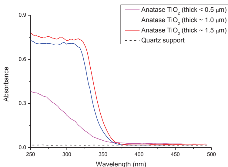
Fig. 3-28 Light absorbance of 400°C-annealed anatase \text{TiO}_2 films deposited on quartz.
