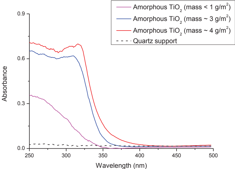
Fig. 3-27 Light absorbance of as-deposit amorphous TiO 2 films deposited on quartz.
