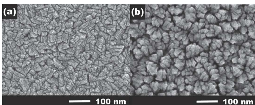
Fig.1-28 Surface morphology of glass-supported \text{TiO}_2 thin film (250 nm thick) obtained from PVD method at two working pressures: (a) 0.92 Pa and (b) 2.77 Pa with electric power 300 W. [154]
