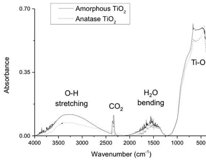
Fig. 3-23 FTIR spectra of as-deposit and 400°C-annealed \text{TiO}_2 film (deposited on silicon substrate).
