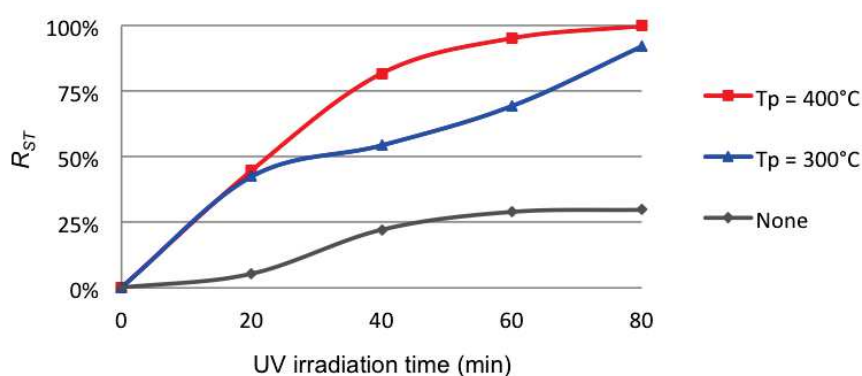
Fig. 4-4 Effect of post-annealing temp. ( T_p ) on photodegraded rate ( R_{ST} ): 300 °C and 400 °C-annealed and non-annealed \text{TiO}_2 thin films prepared at substrate temp. 150^\circ\text{C} .
