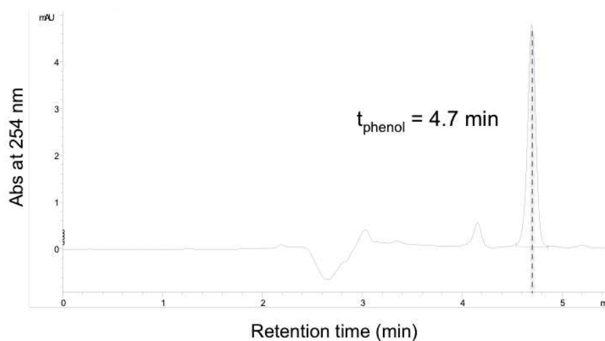
Fig. 4-31 HPLC-UV analysis on phenol in aqueous solution.
