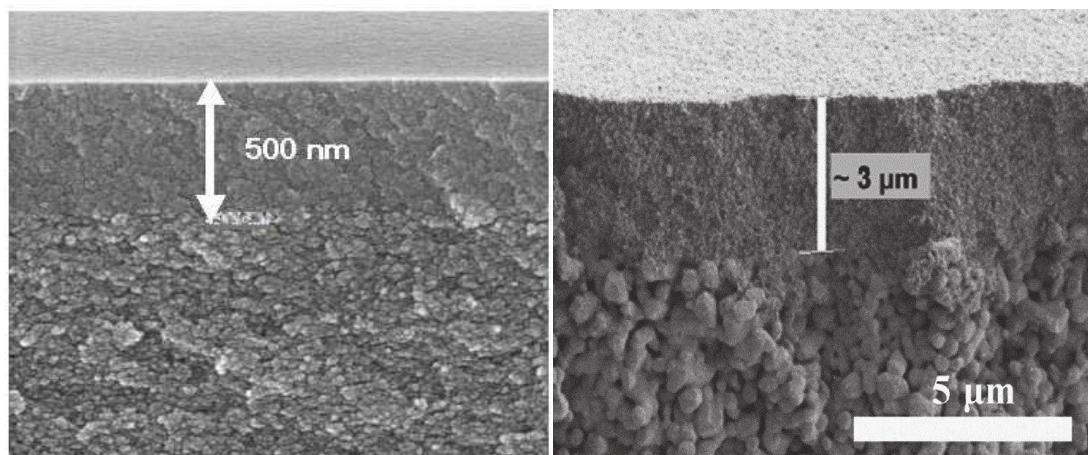
Fig. 1-26 SEM images of \text{TiO}_2/\text{Al}_2\text{O}_3 composite membrane : dip-coated \text{TiO}_2 layers on (a) 5 nm pore-sized top layer \text{Al}_2\text{O}_3 [123] and (b) tubular macroporous \text{Al}_2\text{O}_3 . [14]
