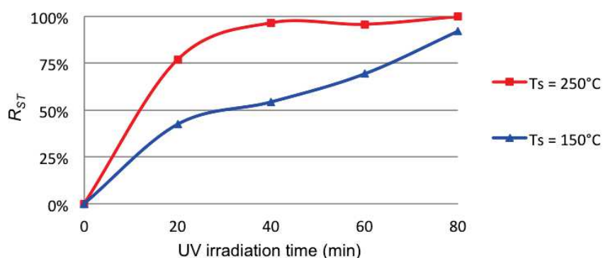
Fig. 4-3 Effect of PECVD substrate temp. ( T_s ) on photodegraded rate ( R_{ST} ): on 300 °C -annealed \text{TiO}_2 thin films prepared at T_s = 150^\circ\text{C} and 250^\circ\text{C} .
