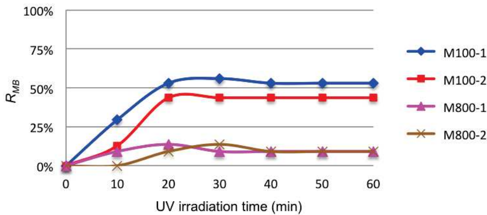
Fig. 4-19 Measured photodegradation R_{MB} on membranes M100 (duplicated) and M800 (duplicated) in the pilot-scale unit with constant UV irradiation ( 50 \text{ W/m}^2 , 355 nm).
