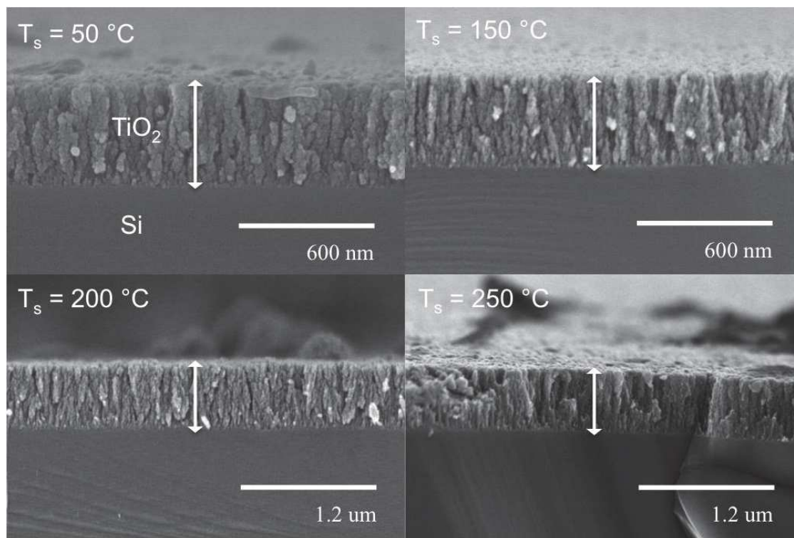
Fig. 3-2 \text{TiO}_2 thickness measured in cross-sectional SEM investigation for samples B1 to B5 deposited at different substrate temperatures from 50 to 250 °C.
