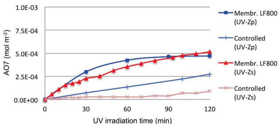
Fig. 4-27 Effect of irradiation spectrum on on photodegraded AO7 per unit surface area ( \text{mol m}^{-2} ) for membrane LF800 and the support (controlled) using 500 W UV lamp with alternative emission of Zp-type (UVA, UVB and UVC) and Zs-type (UVA).
