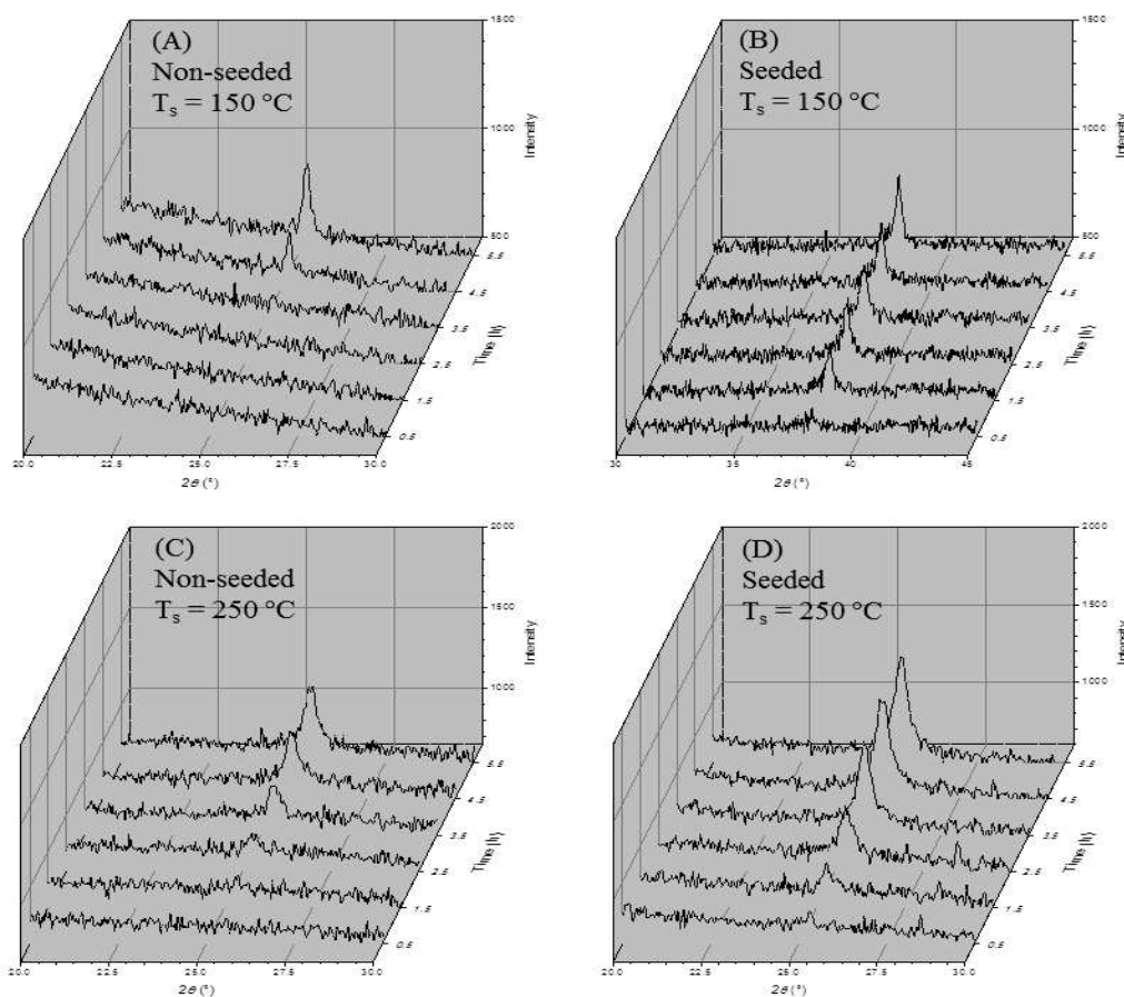
Fig. 3-21 Crystallization kinetics with seeding-effect: high-temperature XRD analysis (heated at 300^\circ\text{C} lasting 6 h) of \text{TiO}_2 thin films on silicon deposited at T_s = 150 and 250^\circ\text{C} (A and C) and on seeded-silicon at T_s = 150 and 250^\circ\text{C} (B and D).
