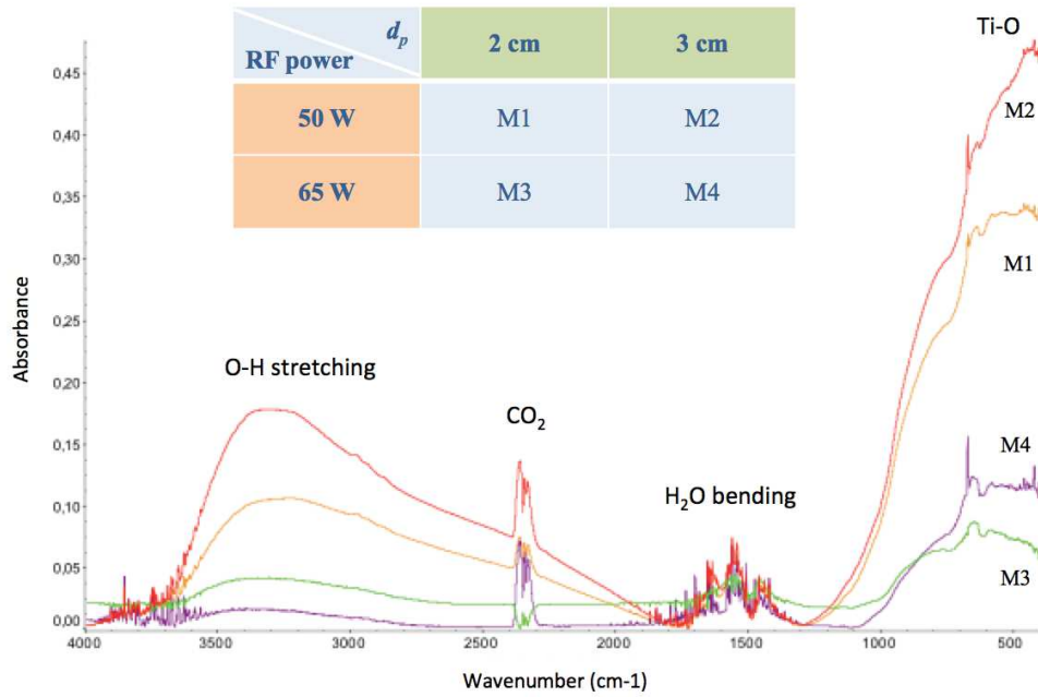
Fig. 3-12 Normalized FTIR spectra (independent from the thickness) of \text{TiO}_2 thin films deposited on silicon as samples M1 – M4.
