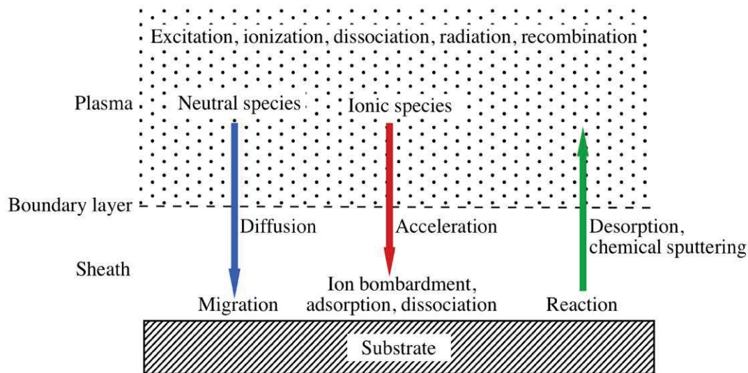
Fig. 1-30 Occurring events in a PECVD reactor. [174]
