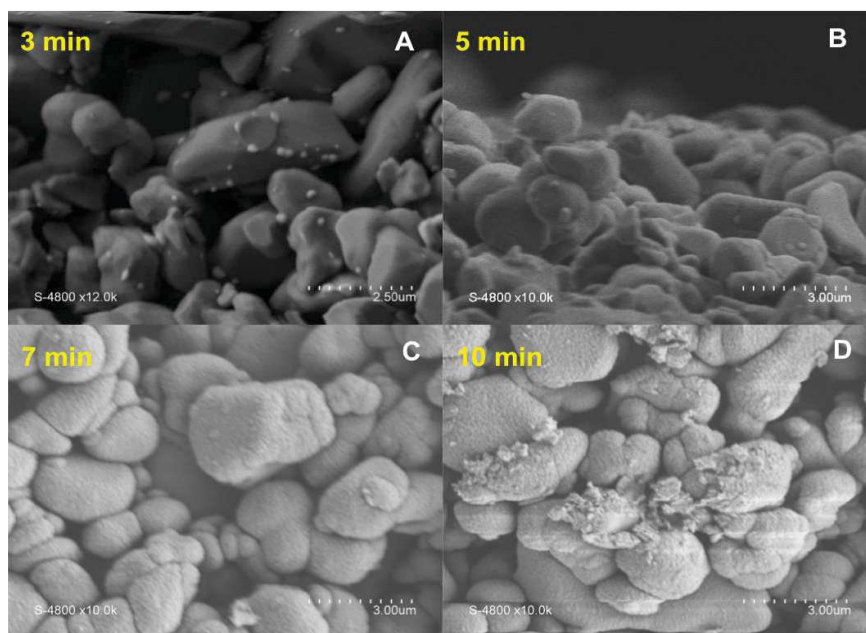
Fig. 4-13 SEM surface images of \text{TiO}_2 skin-covering on ceramic with variant PECVD deposition duration: (A) 3 min, (B) 5 min, (C) 7 min and (D) 10 min.
