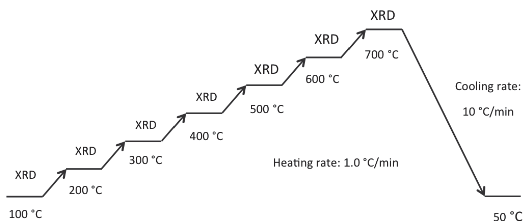
Fig. 2-9 High-temperature X-ray diffraction (HT-XRD) heating program.
