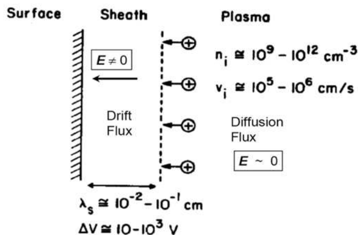
Fig. 1-33 Plasma and sheath in PECVD process. [173]
