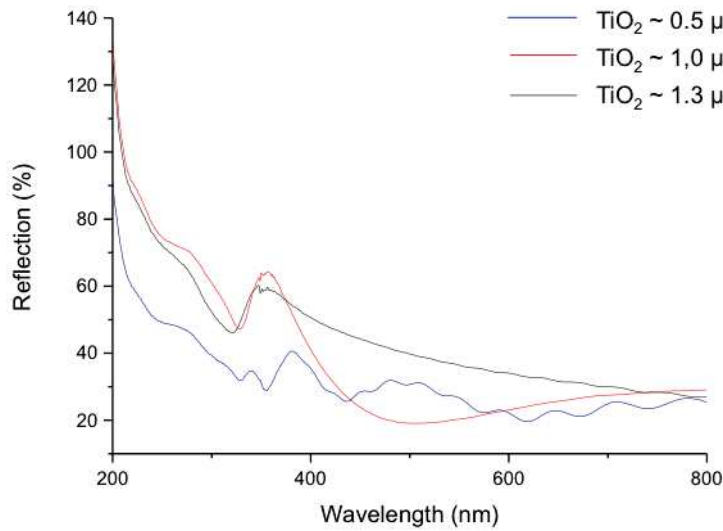
Fig. 3-32 Reflection of light from glass-supported anatase \text{TiO}_2 films of different thickness (deposited with 7, 15 and 20 minutes).
