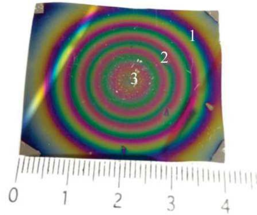
Fig. 3-33 Photo of the optimal anatase TiO 2 film (on silicon) for ellipsometry spectroscopy analysis on three spots (marked as 1, 2 and 3).
