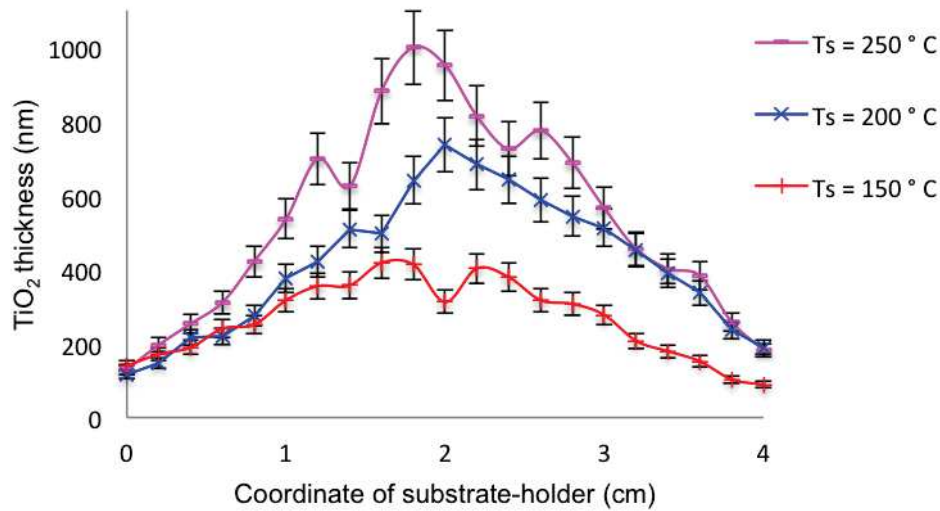
Fig. 3-3 Thickness profile of \text{TiO}_2 thin films versus the coordinate of substrate (at 2cm is the center of the electrode) prepared with PECVD T_s from 150 – 250 ^{\circ}\text{C} (the bars indicating SEM instrumental error for thickness measurement).
