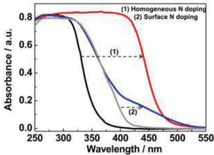
Fig. 1-14 Homogeneous N doping in \text{Cs}_{0.68}\text{Ti}_{1.83}\text{O}_4 . The left panel: UV-visible absorption spectra of (1) homogeneous N doped \text{Cs}_{0.68}\text{Ti}_{1.83}\text{O}_4 and (2) surface N doped \text{TiO}_2 . [103]
