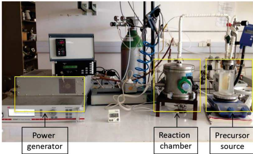
Fig. 2-1 Photo of the PECVD apparatus.
