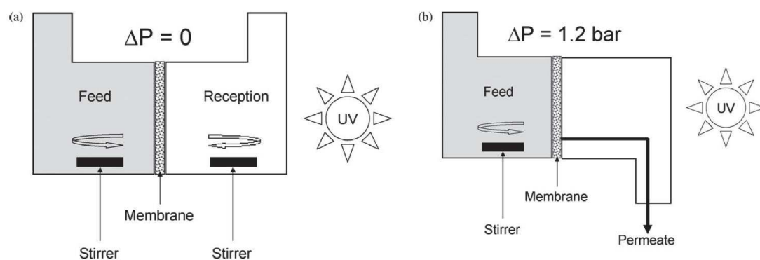
Fig. 1-19 Cell configuration for testing the photocatalytic efficiency of the titania membrane: (a) diffusion cell and (b) permeation cell. [14]
