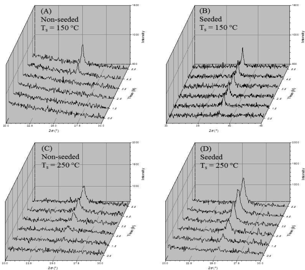
Fig. 3-21 Crystallization kinetics with seeding-effect: high-temperature XRD analysis (heated at 300°C lasting 6 h) of TiO 2 thin films on silicon deposited at T_s = 150 and 250°C (A and C) and on seeded-silicon at T_s = 150 and 250°C (B and D).
