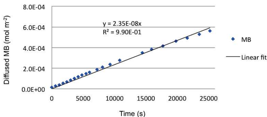
Fig. 4-8 Measurement on diffusion coefficient ( D_i ) of MB compound in water.
