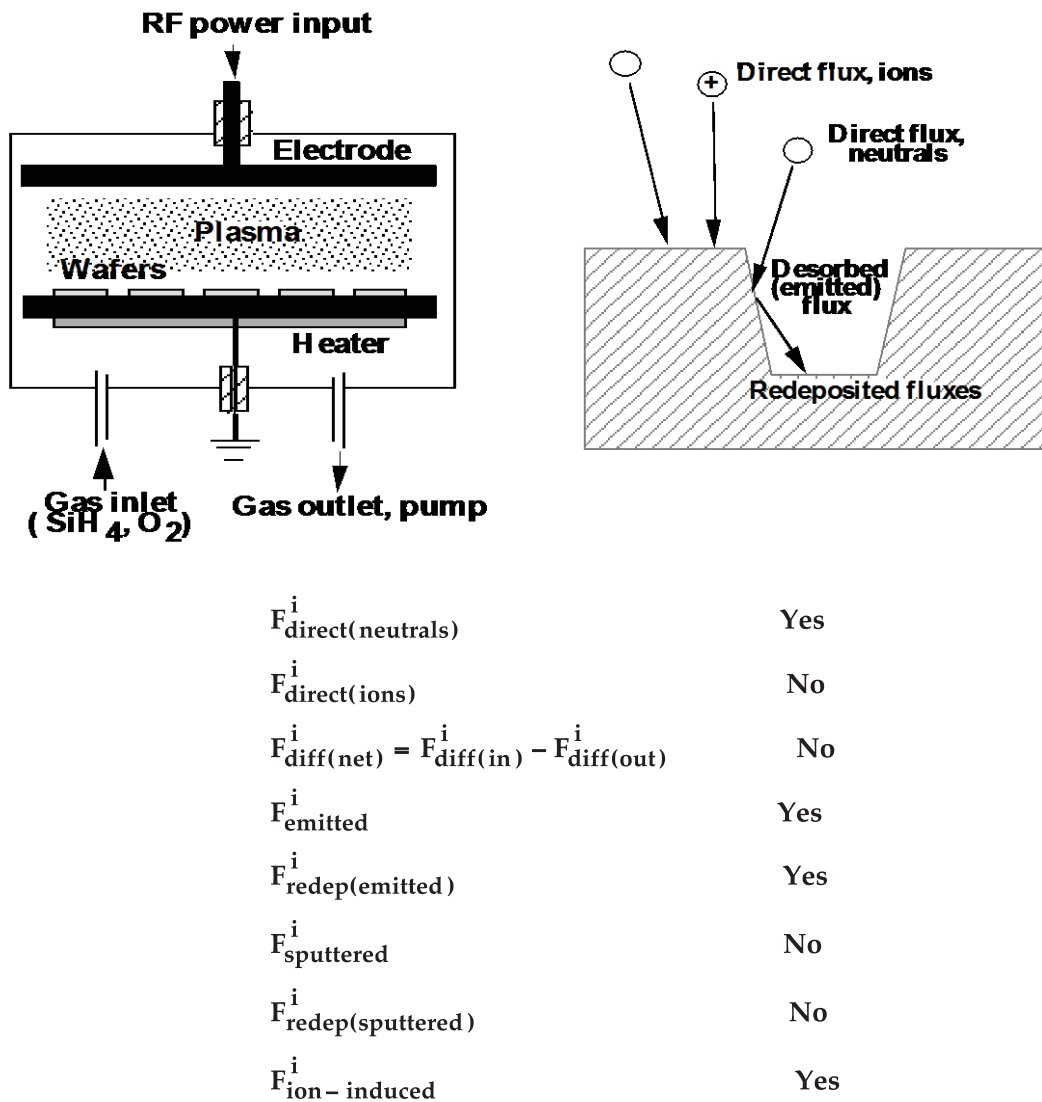
Fig. 1-35 PECVD reactor and relevant fluxes in the deposition process. [173]
