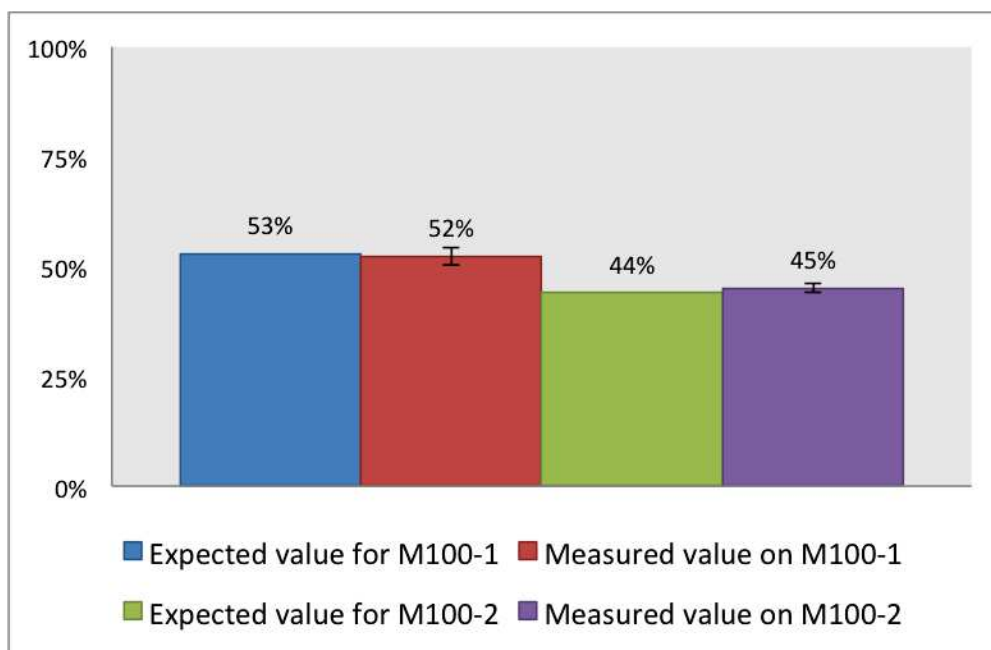
Fig. 4-20 Expected and experimental R_{MB} values on duplicate membrane M100-1 and M100-2 with UV irradiation ( 50 \text{ W m}^{-2} , 355 nm).
