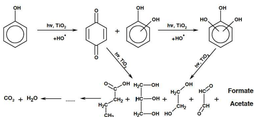
Fig. 1-16 A possible mechanism of phenol destruction on illuminated \text{TiO}_2 . [112]
