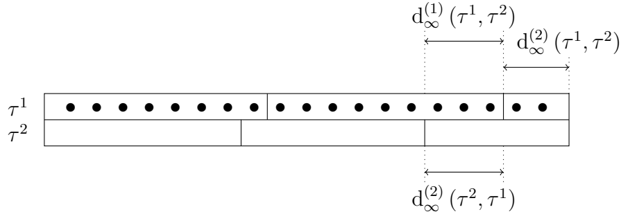
Figure 3-1 – Illustration of the definition of d_\infty^{(i)} , with n = 19 , \tau^1 = [0, 8, 17, 19] and \tau^2 = [0, 7, 14, 19] . In this example, D_{\tau^1} = D_{\tau^2} = 3 . We can compute d_\infty^{(1)}(\tau^1, \tau^2) = d_\infty^{(1)}(\tau^2, \tau^1) = d_\infty^{(2)}(\tau^2, \tau^1) = d_\infty^{(3)}(\tau^1, \tau^2) = 3 and d_\infty^{(2)}(\tau^1, \tau^2) = 2 .
