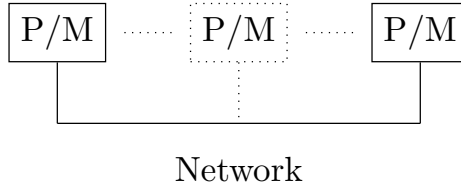
Figure 1.3: A BSP computer.
