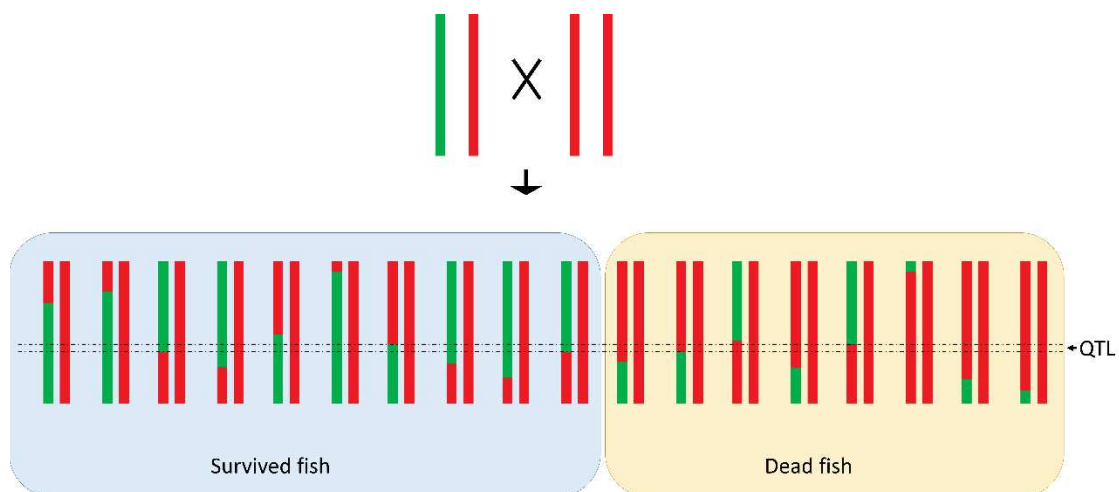
Figure 5.4: Segregation of a QTL of resistance in a progeny derived from the backcross mating of a heterozygous resistant fish and his homozygous sensitive parent. In green, the chromosome carrying the resistant allele at the QTL and in red the chromosome with the sensitive allele at the QTL.
