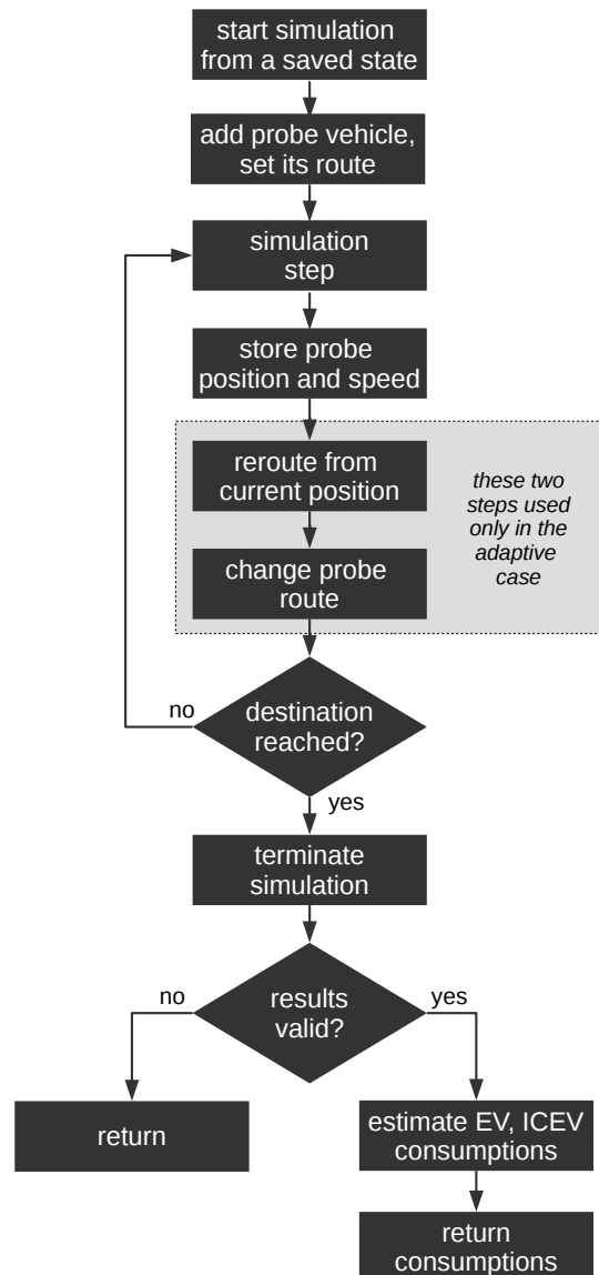
FIGURE 7.4: Simulation workflow.
