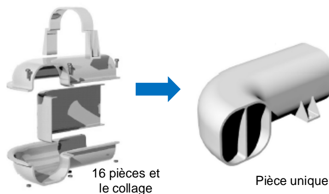
Figure 1.8. Reconcepting of a duct reducing the number of components from 15 to one (Hopkinson, 2006).
