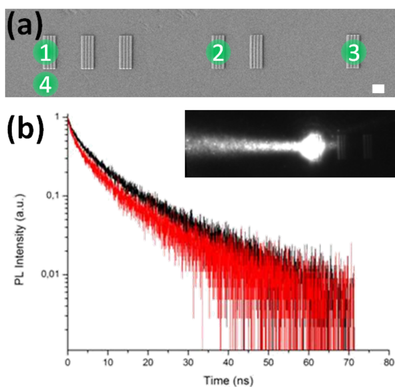
Fig. 5.6 Lifetime measurement for the coupler systems. (a) SEM images of triple-, double- and single-coupler system. The green spots indicate the excitation position of the green laser and they are also the positions for the lifetime measurement. (b) The curve of photoluminescence decay shows the log scale of fluorescence intensity as a function of the time. The red and black curves represent the fluorescence decays of the CdSe nanocrystals at the position 1 and 4 indicated as the green spots in Figure 5.6 (a) respectively. The inset shows the fluorescence image when the laser spot is excited at position 1.
