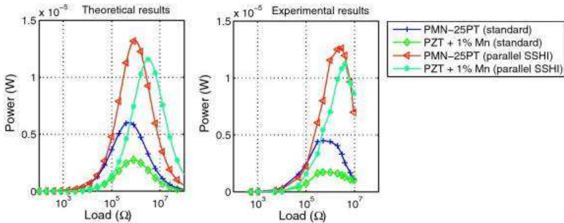
Figure 2.16: Experimental harvested power using standard and SSHI approaches [Rakbamrung et al., 2010].
