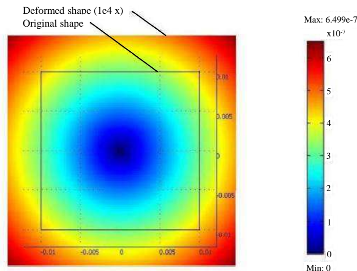
Figure 2.34: Surface variation FEM simulation for a PMN-PT[001] (30% PT) plate, measured in mm [Ivan et al., 2010]. Deformed shape is magnified 10,000 times for optimal visualization.
