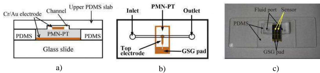
Figure 2.19: Cross sectional schematic (a), top view configuration (b), and photograph (c) of the microfluidic acoustic device integrated with a shear mode PMN-PT piezoelectric single crystal resonator [Zhang et al., 2011a].
