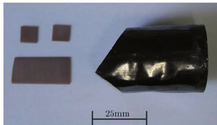
Figure 2.10: 0.71PMN-0.29PT crystal grown [Luo et al., 2009].
