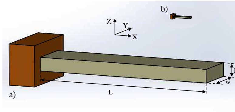
Figure 1.11: Scale induced dynamic changes for a) generic cantilever B_1 and an identically designed b) downscaled (to 10%) cantilever beam B_2
