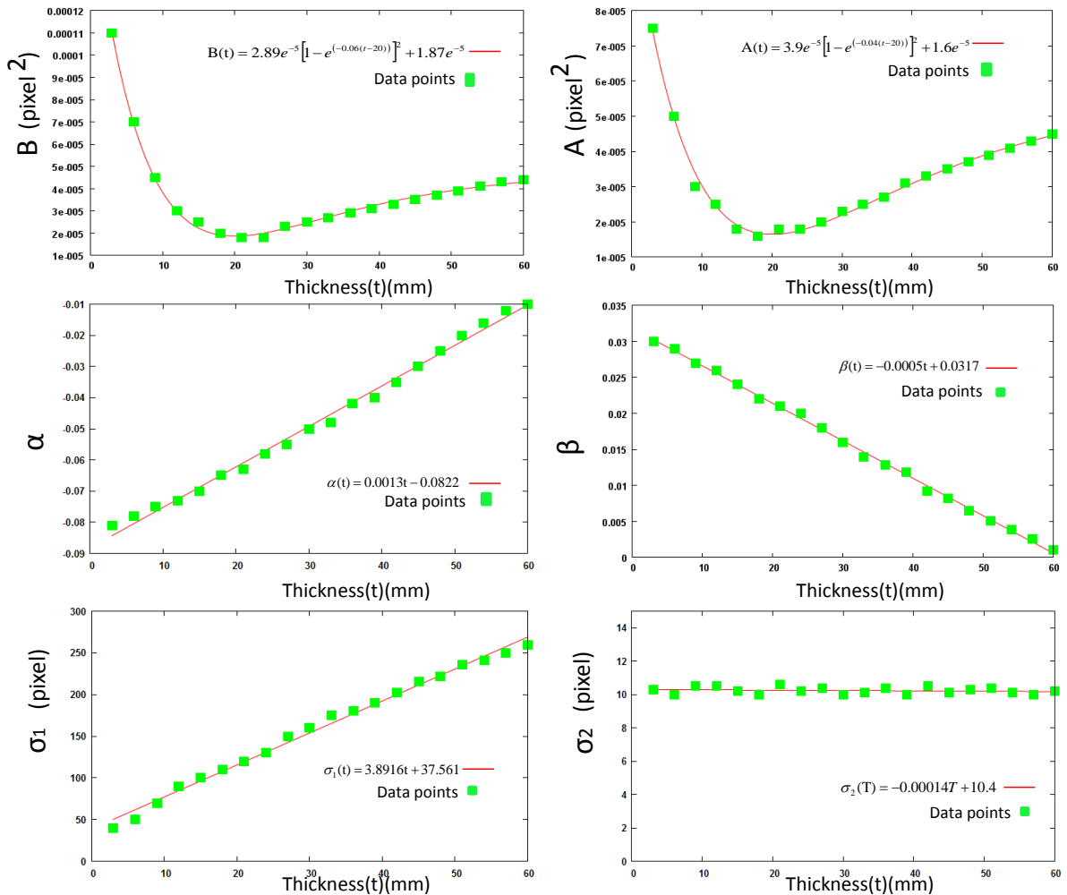
Figure 2.6: Fitting of parameters \alpha , \beta , A , B , \sigma_1 , \sigma_2 with thickness
