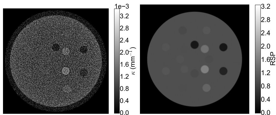
Figure 5.4: The \kappa -map (left) and RSP -map (right) of the Gammex 467 phantom for reconstructions using the MLP . The maximum value of the grayscale was chosen to be twice the maximum theoretical reconstruction value of the insert, which in this case is SB3. The factor 2 is necessary to account for the increase of \kappa at the borders due to the overshoot at these regions. In both imaging acquisitions, the minimum gray level was set to zero.
