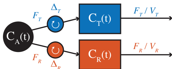
Figure 5-3c: Block diagram of the relative one-compartment model in case of a single region of interest.
