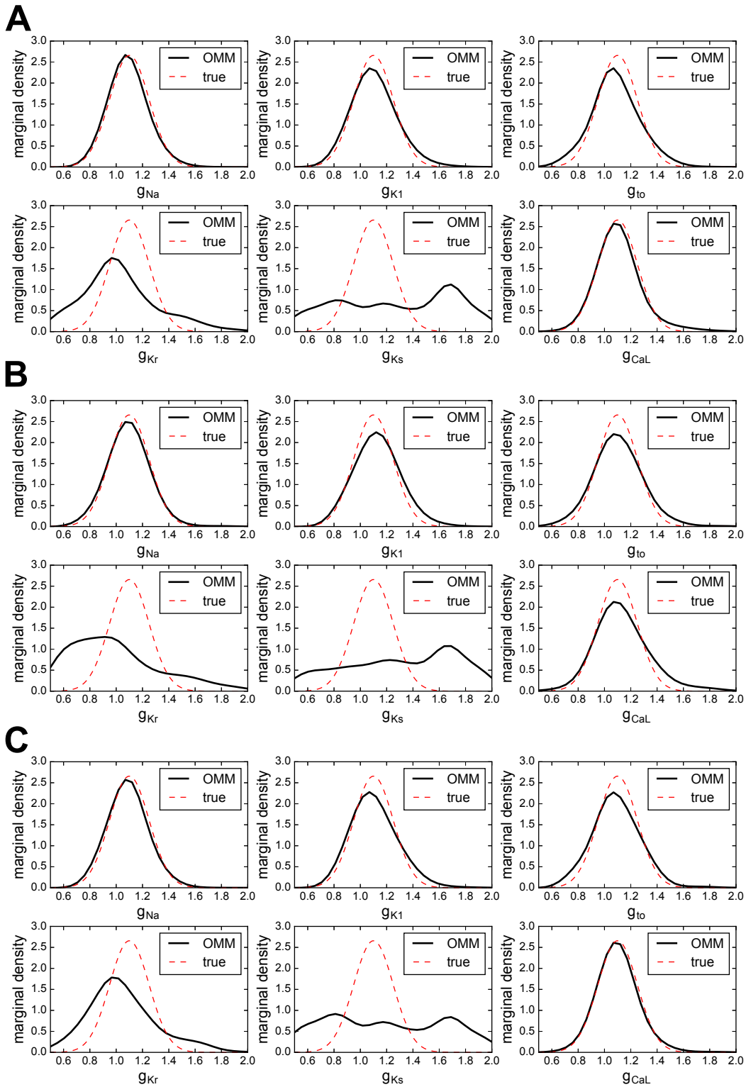
Figure 3.4: Test Case 2 using the Courtemanche model and synthetic data. Conductances estimated marginal densities in (A) control conditions (1Hz stimulation frequency), (B) fast pacing conditions (2Hz stimulation frequency) and (C) with combined data from 1Hz and 2Hz pacing.
