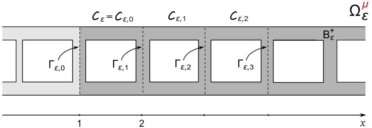
Figure 3.3: The cells \mathcal{C}_{\varepsilon,n} and the boundaries \Gamma_{\varepsilon,n}
