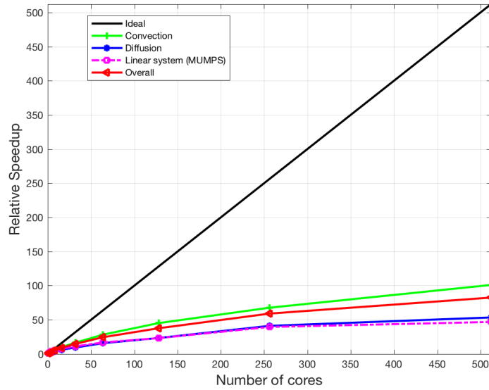
Figure 4.14: Speedup of different parts of parallel 3D streamer code using mesh with 657542 cells
