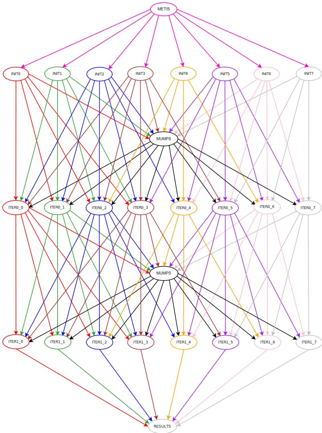
Figure 5.1: The ADAPT workflow
