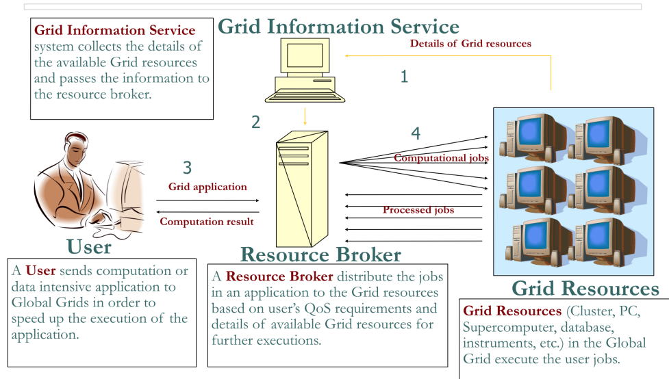
Figure 3.4: Grid computing
