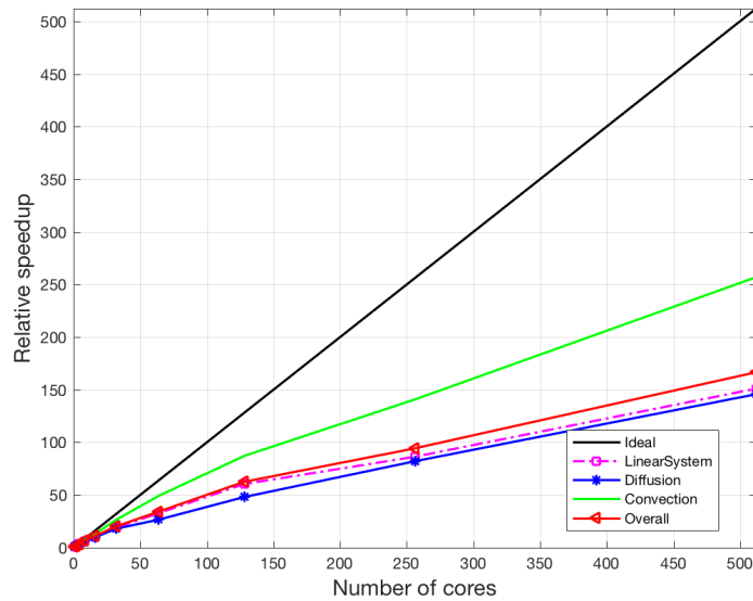
Figure 4.17: Speedup of different parts of parallel 3D streamer code using mesh with 2000186 cells
