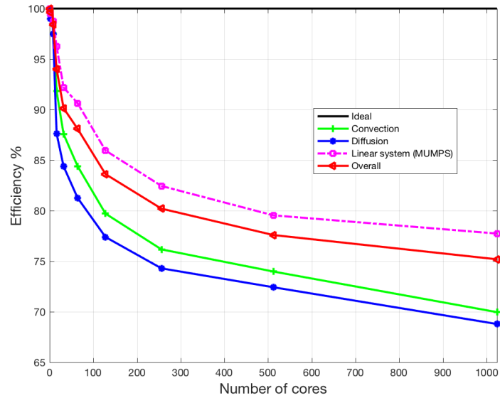
Figure 4.11: Efficiency of different parts of parallel 2D streamer code using mesh with 1324486 cells
