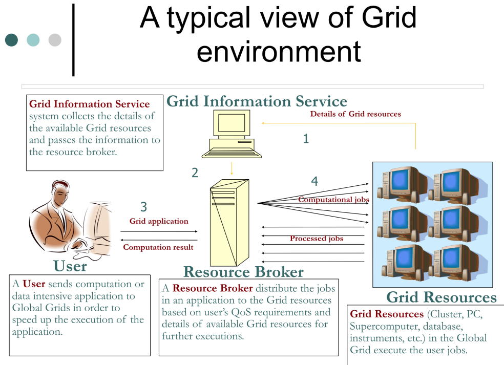
Figure 3.4: Grid computing
