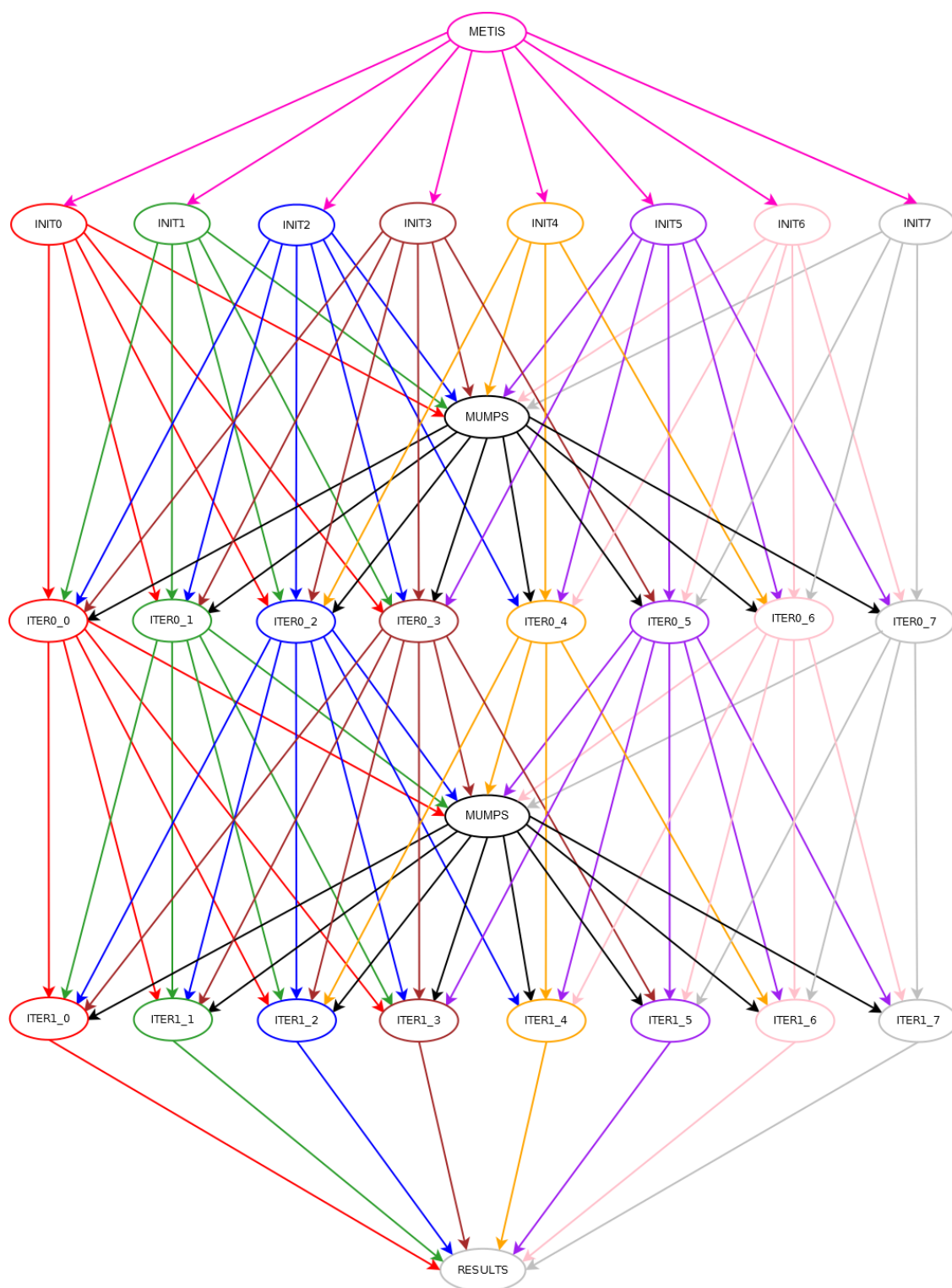
Figure 5.1: The ADAPT workflow
