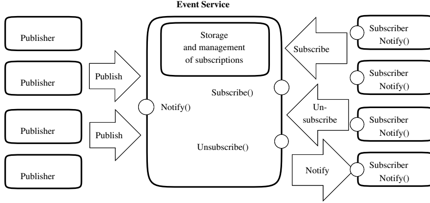
Figure 3.5: The publish-Subscribe paradigm in action
