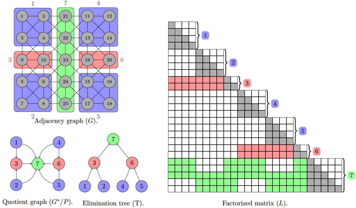
Figure 2.14: Symbolic factorization and elimination tree
