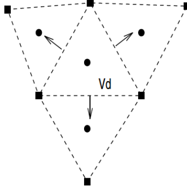
Figure 4.2: Cell-centered
