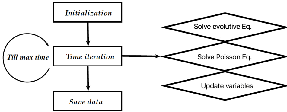
Figure 4.5: The main procedure of ADAPT solver
