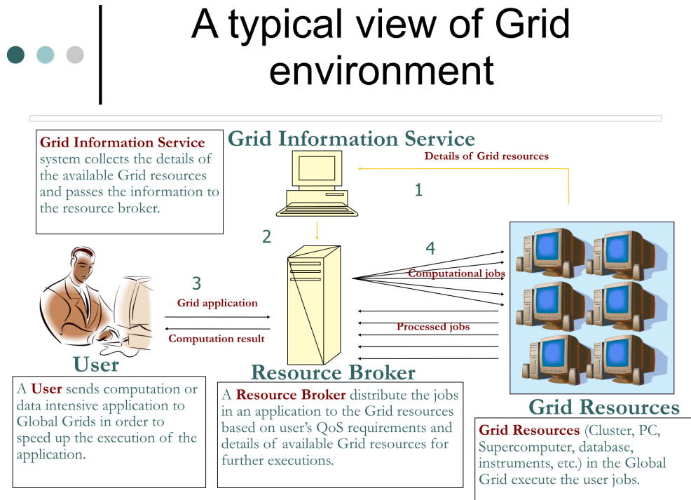
Figure 3.4: Grid computing
