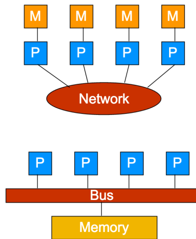
Figure 2.5: Shared vs Distributed memory
