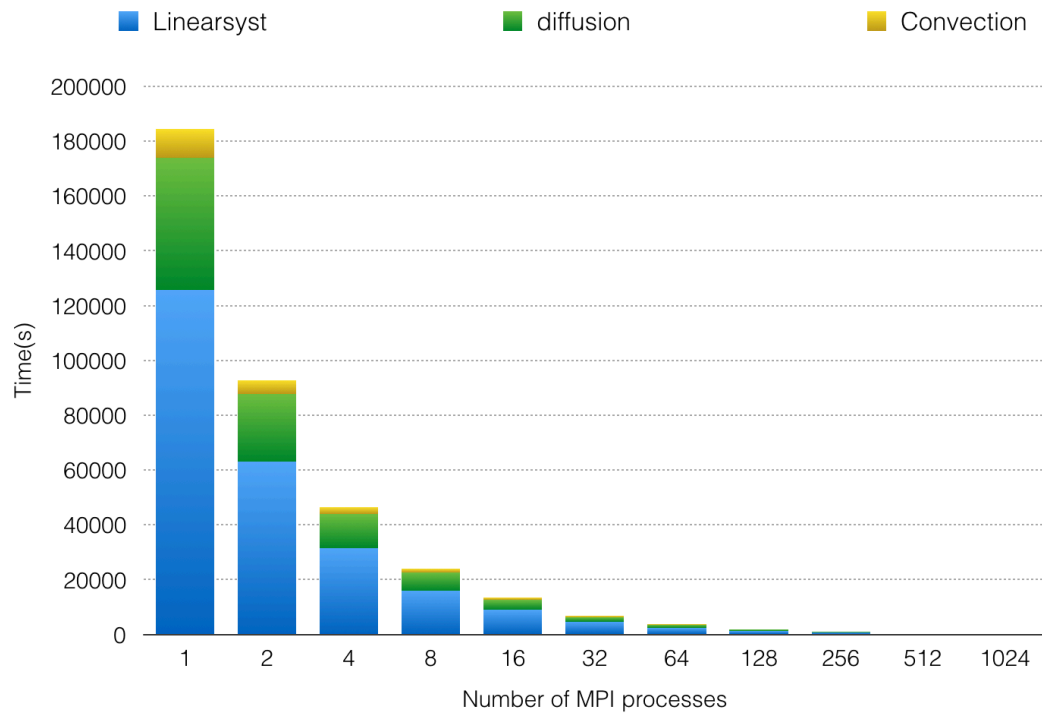
Figure 4.6: Time breakdown for running 2D streamer code using 529240 cells
