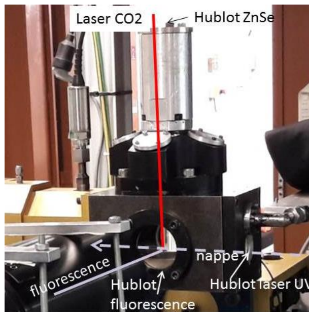
Figure 4.4 Enceinte CHAMADE
