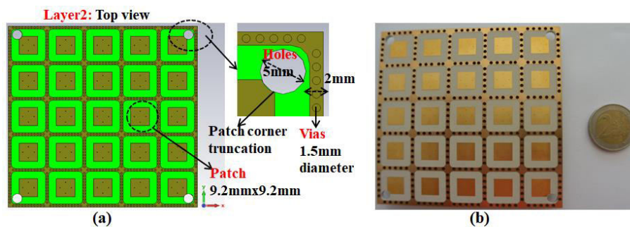
Figure IV-24. Layer2, patches and metallic plates: (a) top view, (b) fabrication.
