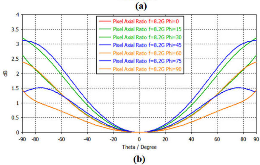
Figure II-18. Pixel with patch fed by four ports, (a) gain pattern, (b) axial ratio pattern.
