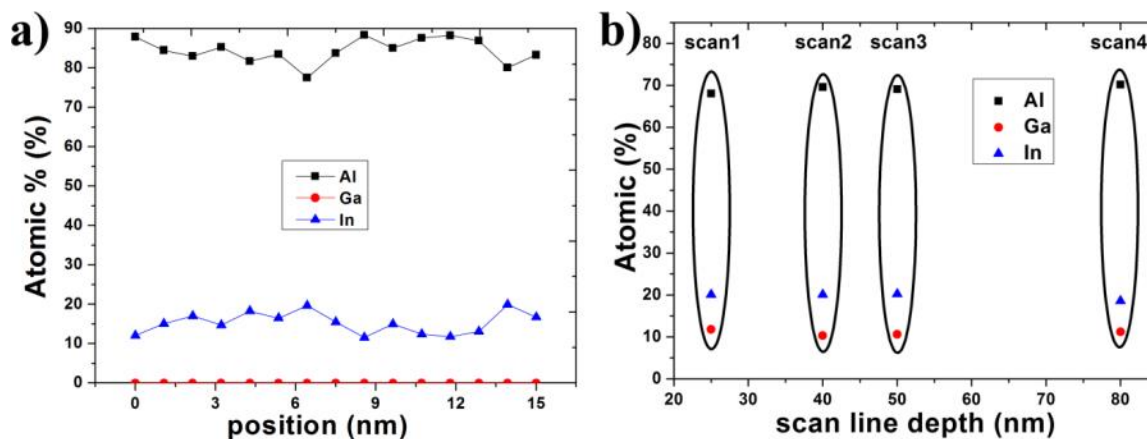
Figure 3.5: a) and b) are EDS measurements made on A383 and TS241, respectively. No gallium has been detected in A383. For TS241, higher indium content is highlighted than given by XRD, in addition, the presence of gallium is not negligible
