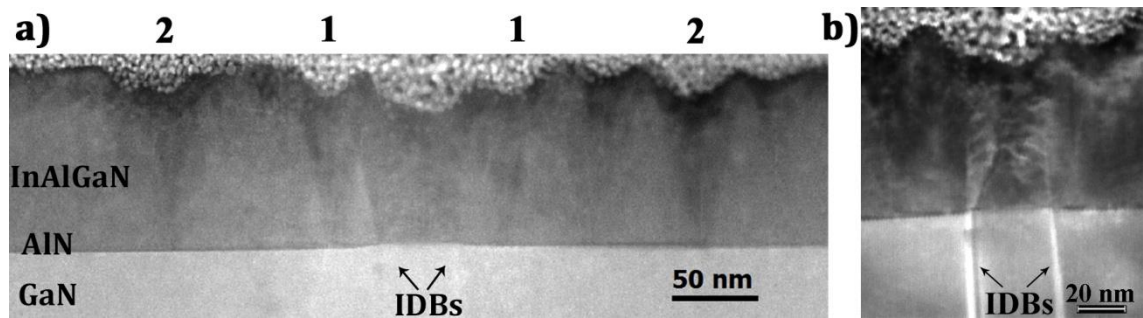
Figure 4.10: The material that is grown on top of an N-polar GaN. a) ADF low magnification cross section showing the whole trench structure along a \langle 112\bar{0} \rangle zone axis. b) Magnified ADF image of the inner part of the ID recorded using a large camera length in order to display the local strain
