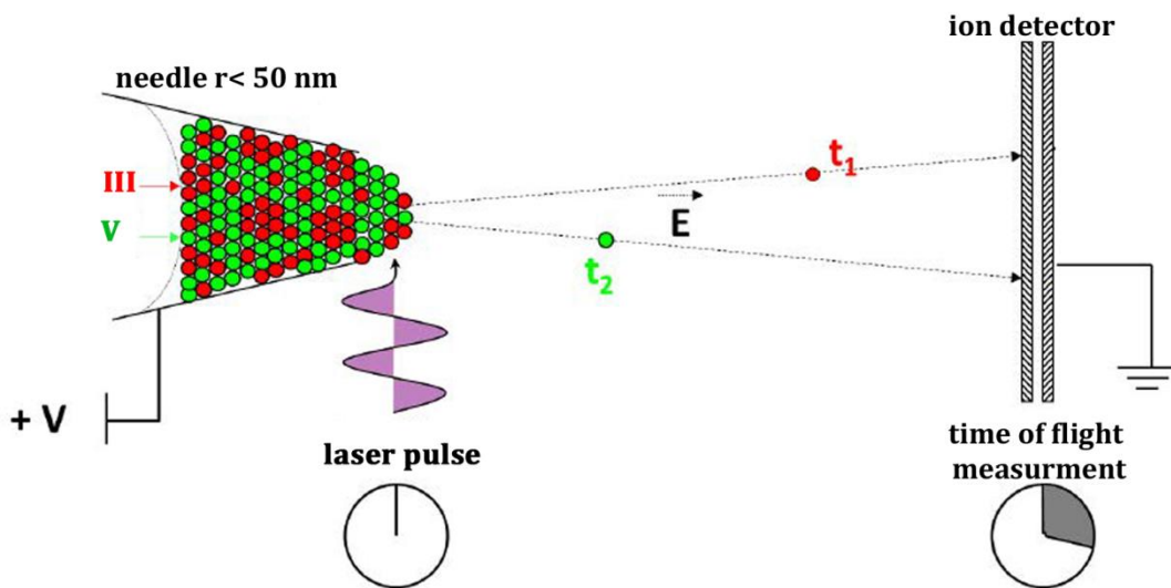
Figure 2.9: Schematic showing the principle of the APT process. With modifications from [71].
