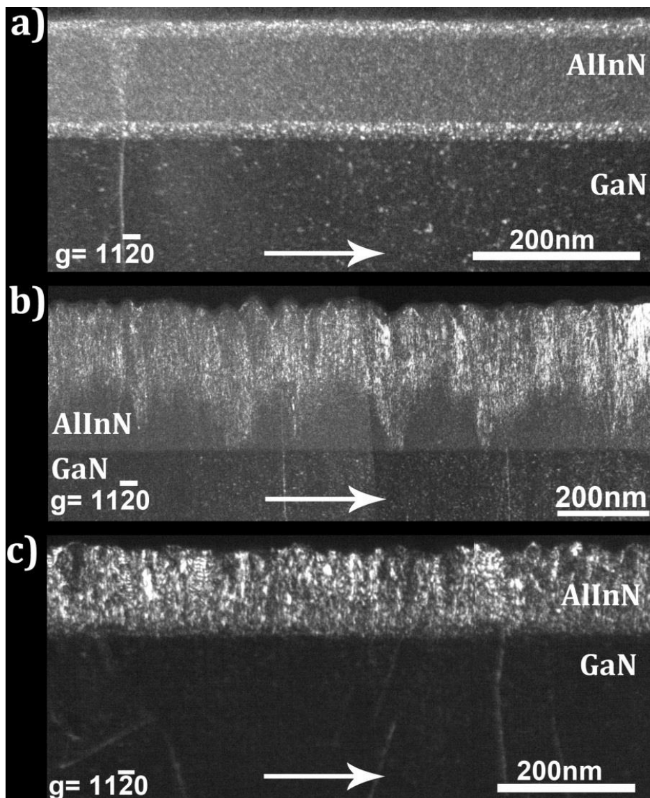
Figure 6.3: Weak beam dark field micrographs were recorded with g = 11\bar{2}0 for a) A383, b) 1363 and c) MD3156. Clearly, the microstructure does not only depend on the TDs but also on the thickness and the strain state.
