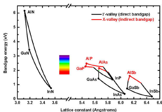
Figure 1: Band gap of semiconductors plotted as a function of their lattice parameter[2].
