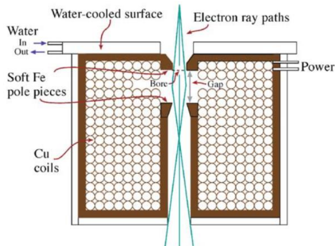
Figure 2.4: Cross-section view of a magnetic lens[64].
