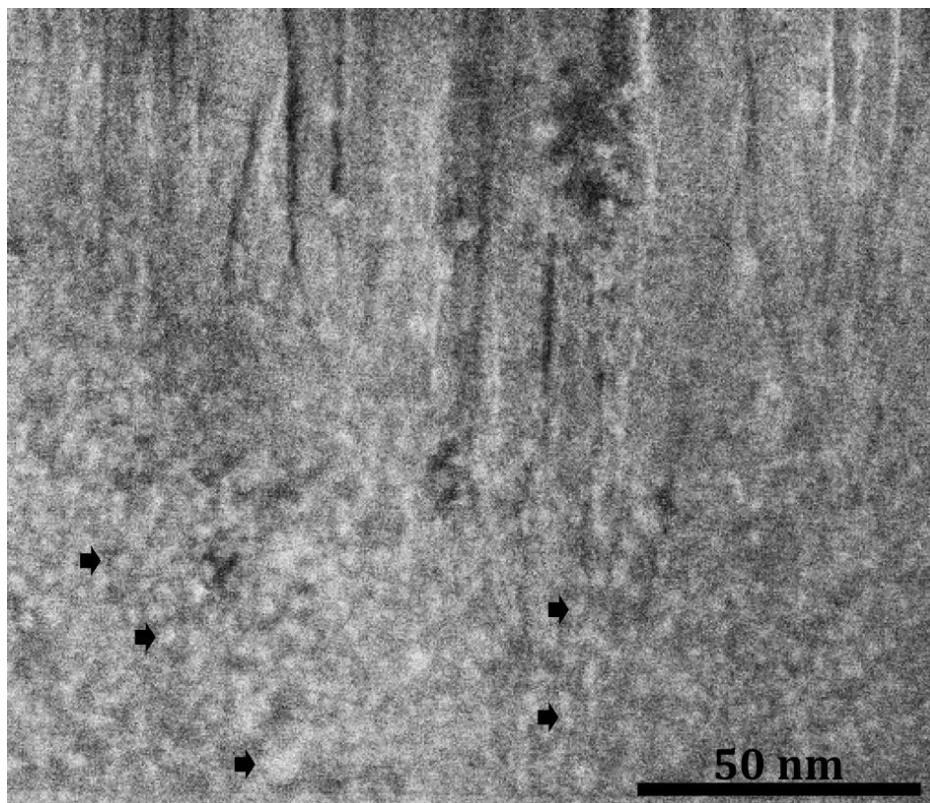
Figure 6.13: HAADF micrograph recorded with 6 cm camera length showing different Z-contrast near \langle 10\bar{1}0 \rangle zone axis. This region is taken near the interface AlInN/GaN.
