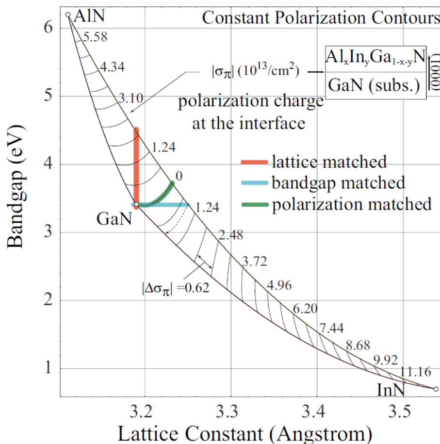
Figure 3: The possibilities that offer AlGaInN alloys in terms of the lattice parameters, bandgap, and polarization matches while grown on (0001)-GaN[23].
