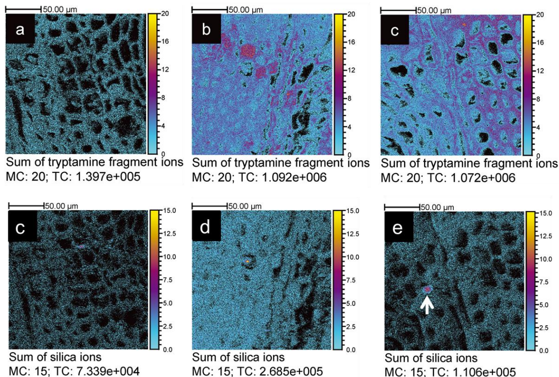
Figure 26: Distribution of tryptamine and silica on the transverse surface of D. guianensis . (a) & (c): sapwood. (b) & (d): transition zone. (c) & (e): heartwood. Images have been cropped to zoom on areas of interest of 200\ \mu\text{m} \times 200\ \mu\text{m} size. The white arrows show the silica grain [58].
