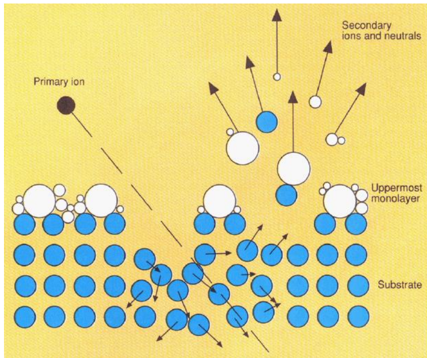
Figure 1: Secondary ions and neutrals emission induced by the primary ions via a collision cascade [5].
