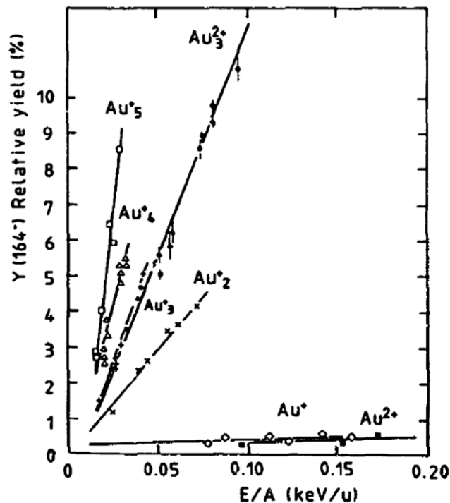
Figure 4: Molecular ion ( m/z 164.2, [\text{M}-\text{H}]^+ ) yield from a phenylalanine target as a function of energy per mass unit ( E/A ) of gold clusters \text{Au}_n^{q+} ( n=1-5 , q=1-2 ) [24].
