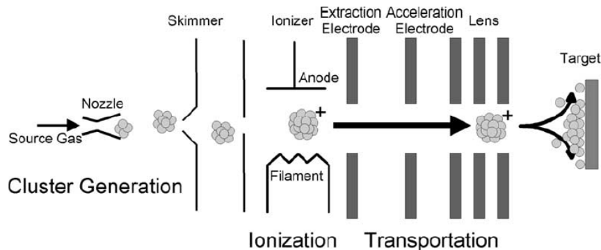
Figure 14: Schematic diagram of gas cluster ion beam generation [39].
