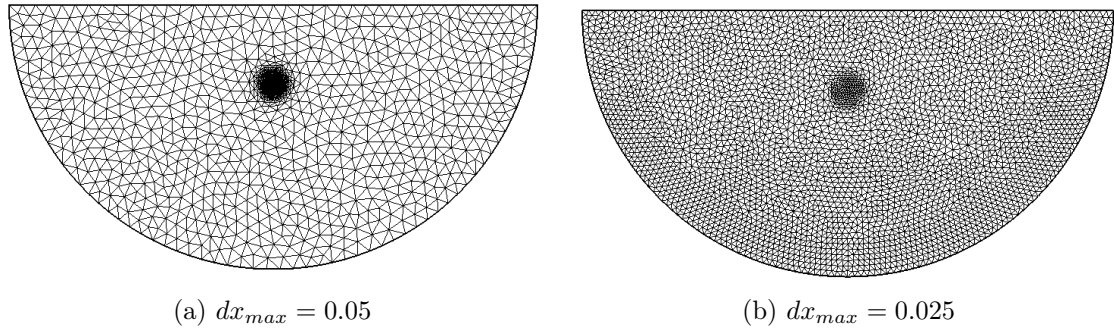
Figure 5.1: Two different meshes of the computational domain. Both are adjusted around the injection point.
