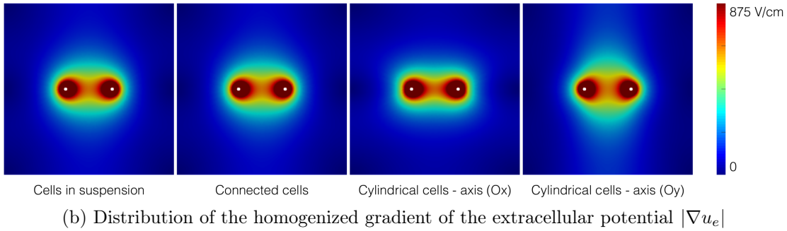
Figure 3.10: Spatial distribution of two homogenized quantities computed in the linear case: (a) |v| and (b) |\nabla u_e| are obtained in all 4 cases of reference cells presented in Figure 3.4.
