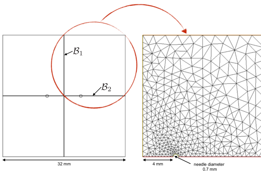
Figure 2.4: 2D full domain and final computational mesh obtained considering the symmetry of the problem.
