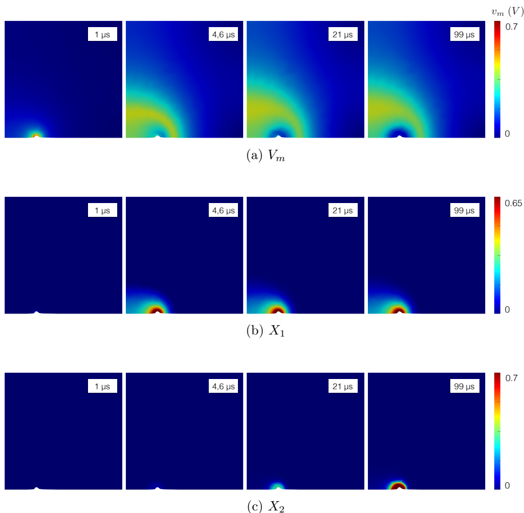
Figure 2.23: Spatial distribution over time of the magnitude of the mean transmembrane potential v_m and for both electroporation processes X_1 and X_2 computed with the dynamic model using two current densities for an applied voltage of 875 V/cm.
