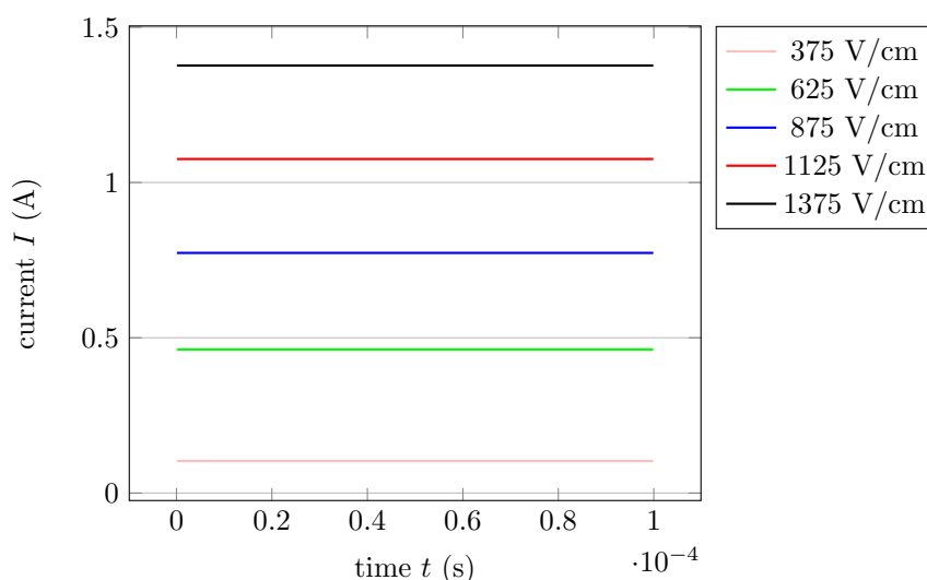
Figure 2.12: Simulated current of the static model for five different voltage applied.
