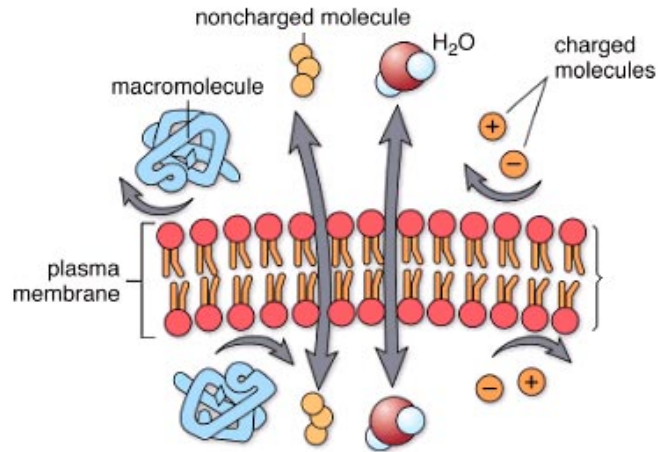
Figure 3: Transport of molecules across the plasma membrane: schematic representation of membrane selective permeability.
