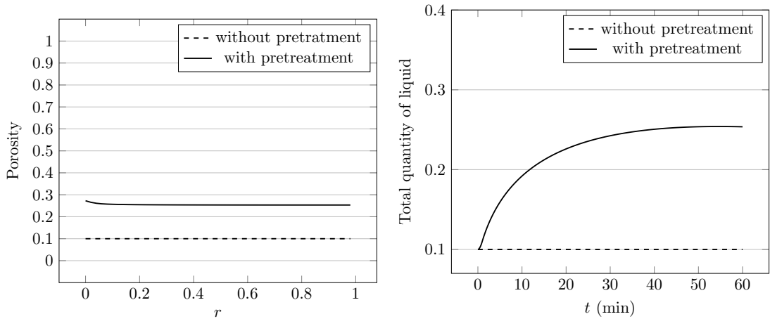
(a) Porosity versus radial position 60 minutes after the injection. (b) Quantity of fluid in the tissue versus time after the injection.
