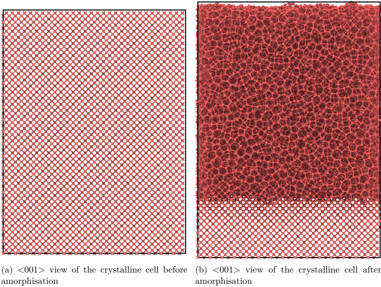
Figure II.11: Simulation cell preparation for MD calculations. Views generated by OVITO [Stukowski 2010]
