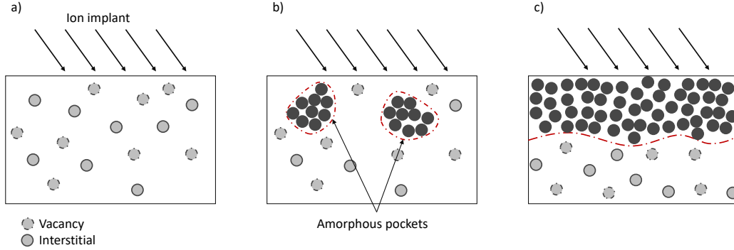
Figure I.13: Continuous cascades leading to a continuous amorphous layer
