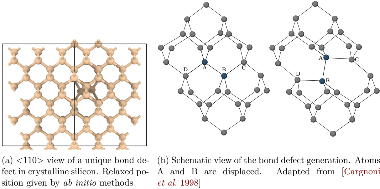
Figure II.6: The bond defect
