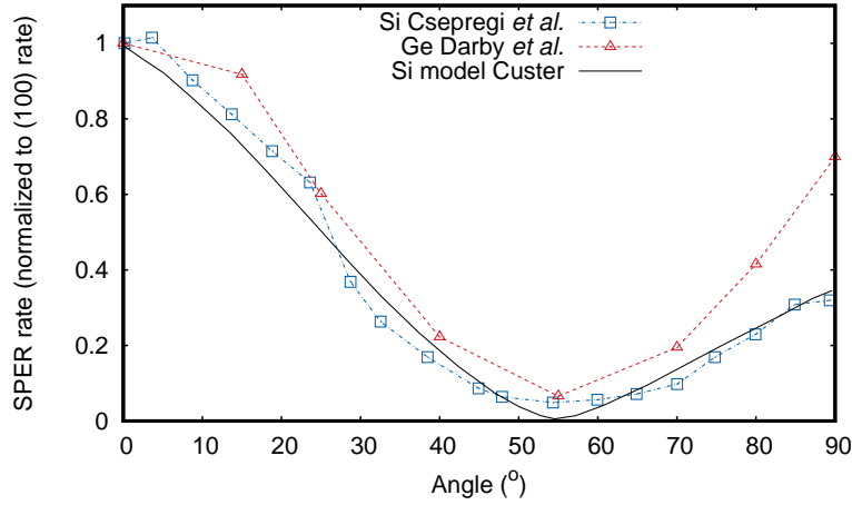
Figure I.19: Regrowth rates for silicon and germanium SPER showing their substrate orientation dependences. Experimental data from [Csepregi et al. 1978] and [Darby et al. 2013]. Model from [Custer 1992]
